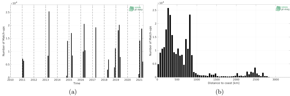
Figure 1: Number of match-ups between TSG (CSIC-UTM) and SMOS SSS L3 v2 - 9-Days (BEC) SSS as a function of time (a) and as function of the distance to coast (b) over the South Atlantic Ocean Pi-MEP region and for the full satellite product period.
