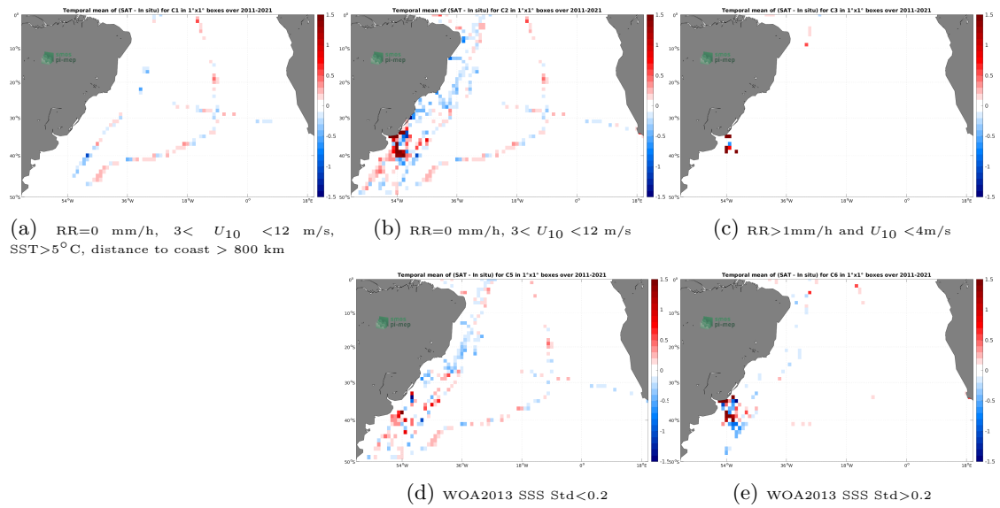
Figure 12: Temporal mean gridded over spatial boxes of size 1^\circ \times 1^\circ of \Delta SSS (SMOS SSS L3 v2 - 9-Days (BEC) - TSG (CSIC-UTM)) for 5 different subdatasets corresponding to:RR=0 mm/h, 3 < U_{10} < 12 m/s, SST >5^\circ\text{C} , distance to coast > 800 km (a), RR=0 mm/h, 3 < U_{10} < 12 m/s (b), RR >1 mm/h and U_{10} < 4 m/s (c), WOA2013 SSS Std <0.2 (d), WOA2013 SSS Std >0.2 (e).
