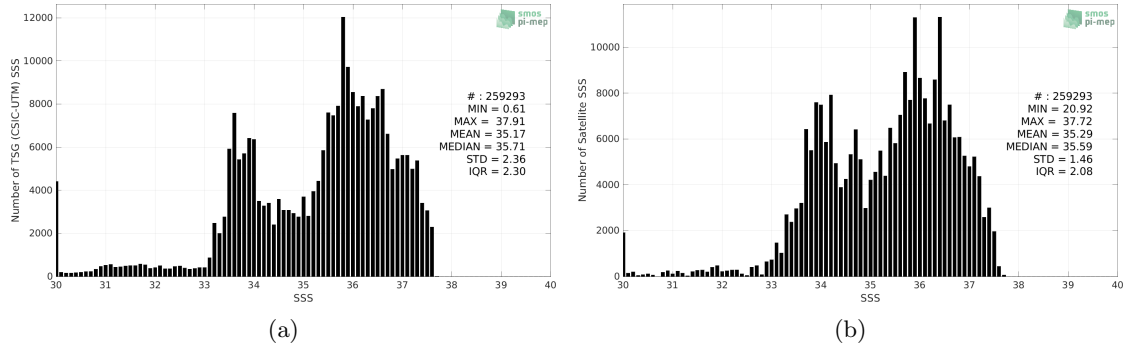
Figure 2: Histograms of SSS from TSG (CSIC-UTM) (a) and SMOS SSS L3 v2 - 9-Days (BEC) (b) considering all match-up pairs per bins of 0.1 over the South Atlantic Ocean Pi-MEP region and for the full satellite product period.
