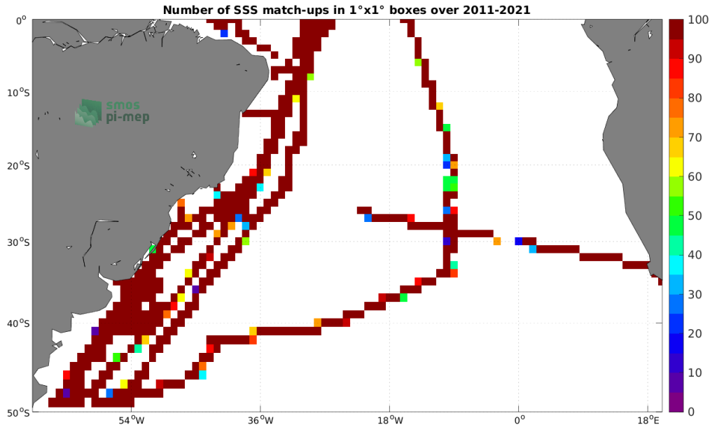
Figure 4: Number of SSS match-ups between TSG (CSIC-UTM) SSS and the SMOS SSS L3 v2 - 9-Days (BEC) SSS product for the South Atlantic Ocean Pi-MEP region over 1^\circ \times 1^\circ boxes and for the full satellite product period.
