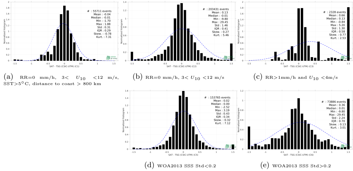
Figure 13: Normalized histogram of \Delta SSS (SMOS SSS L3 v2 - 9-Days (BEC) - TSG (CSIC-UTM)) for 5 different subdatasets corresponding to: RR=0 mm/h, 3 < U_{10} < 12 m/s, SST>5°C, distance to coast > 800 km (a), RR=0 mm/h, 3 < U_{10} < 12 m/s (b), RR>1mm/h and U_{10} < 4 m/s (c), WOA2013 SSS Std<0.2 (d), WOA2013 SSS Std>0.2 (e).
