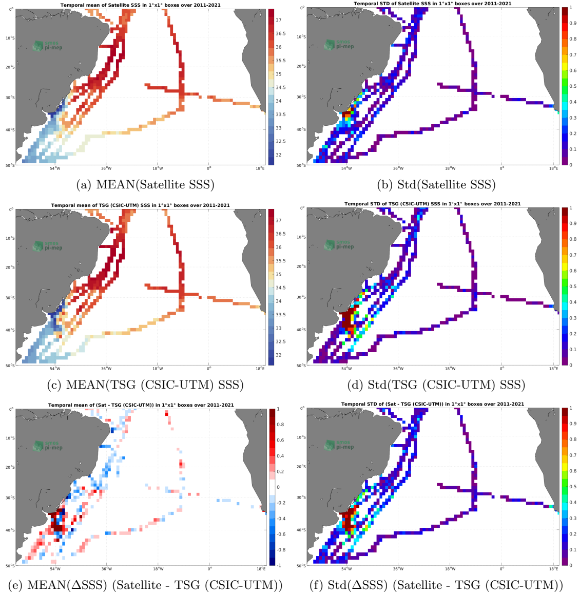
Figure 6: Temporal mean (left) and Std (right) of SSS from SMOS SSS L3 v2 - 9-Days (BEC) (top), TSG (CSIC-UTM) (middle), and of \Delta SSS (Satellite - TSG (CSIC-UTM)). Only match-up pairs are used to generate these maps.
