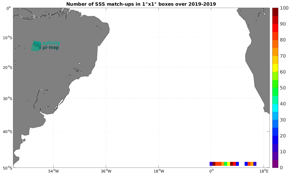
Figure 5: Number of SSS match-ups between Sairdrone SSS and the SMOS SSS L3 v2 - 9-Days (BEC) SSS product for the South Atlantic Ocean Pi-MEP region over 1^{\circ} \times 1^{\circ} boxes and for the full satellite product period.
