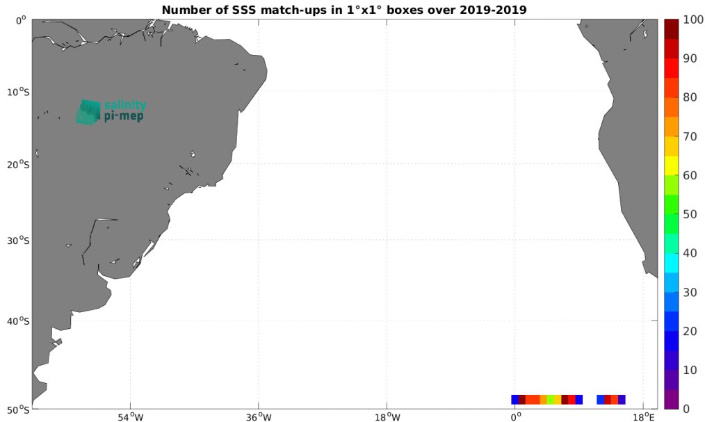
Figure 4: Number of SSS match-ups between Sairdrone SSS and the SMOS SSS L3 v2 - 9-Days (BEC) SSS product for the South Atlantic Ocean Pi-MEP region over 1^{\circ} \times 1^{\circ} boxes and for the full satellite product period.
