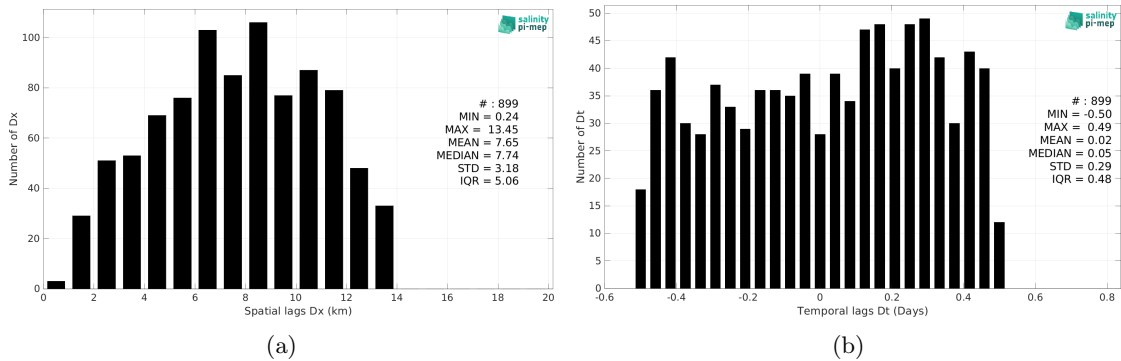
Figure 5: Histograms of the spatial (a) and temporal (b) lags between the location/time of the Sairdrone measurement and the date of the corresponding SMOS SSS L3 v2 - 9-Days (BEC) SSS pixel.
