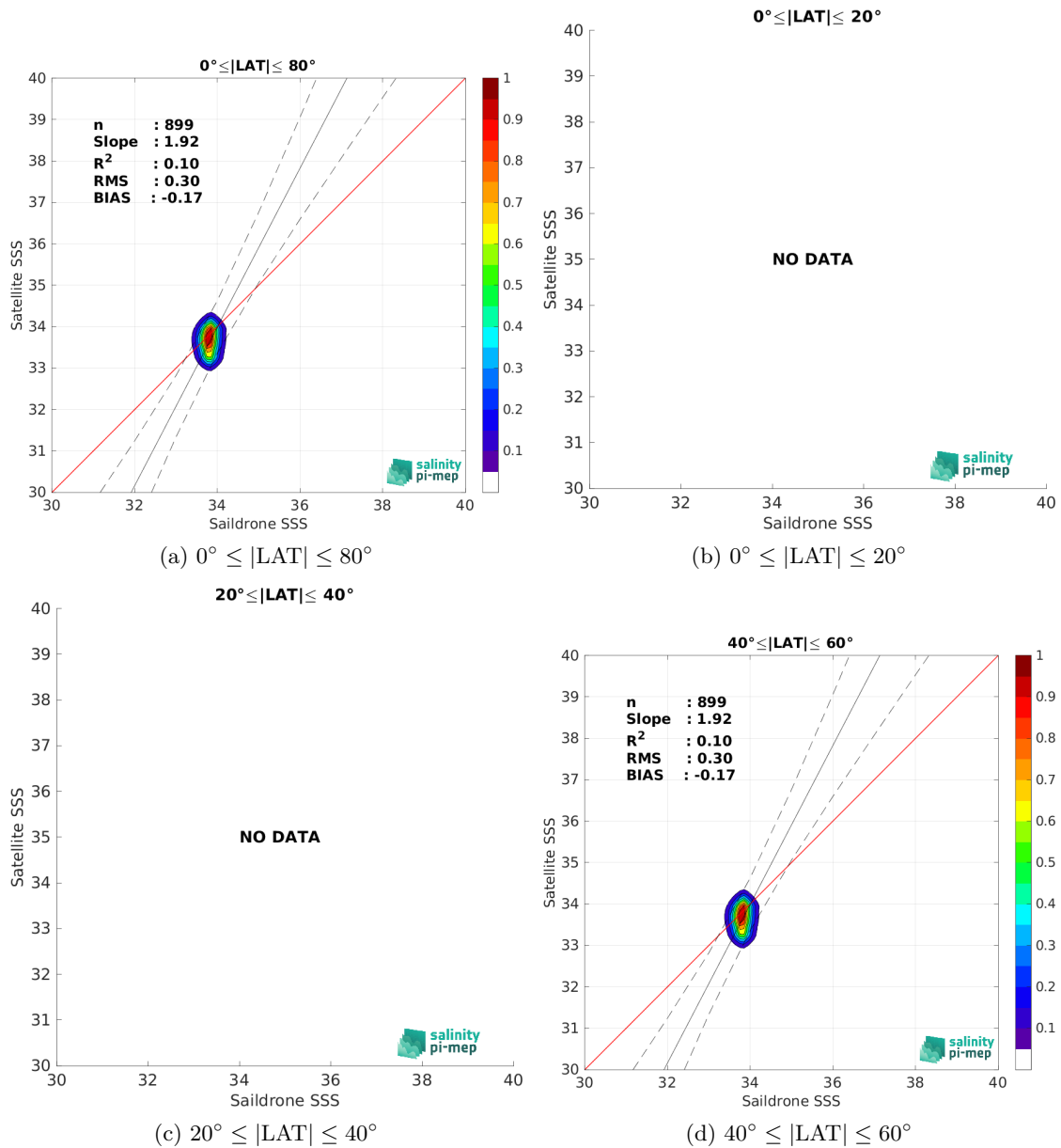
Figure 9: Contour maps of the concentration of SMOS SSS L3 v2 - 9-Days (BEC) SSS (y-axis) versus Saildrone SSS (x-axis) at match-up pairs for different latitude bands. For each plot, the red line shows x=y . The black thin and dashed lines indicate a linear fit through the data cloud and the \pm 95\% confidence levels, respectively. The number match-up pairs n , the slope and R^2 coefficient of the linear fit, the root mean square (RMS) and the mean bias between satellite and in situ data are indicated for each latitude band in each plots.
