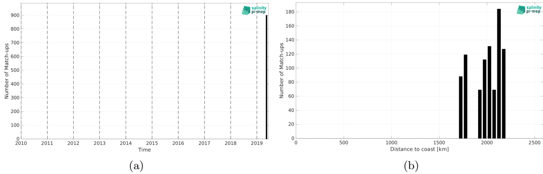
Figure 1: Number of match-ups between Saildrone and SMOS SSS L3 v2 - 9-Days (BEC) SSS as a function of time (a) and as function of the distance to coast (b) over the South Atlantic Ocean Pi-MEP region and for the full satellite product period.
