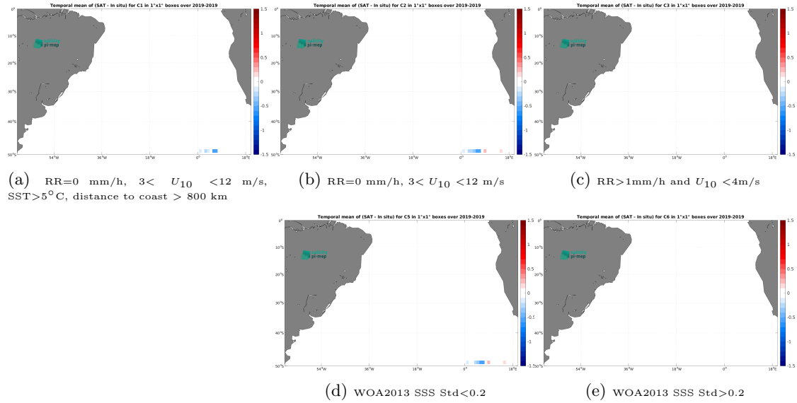
Figure 12: Temporal mean gridded over spatial boxes of size 1^{\circ}\times 1^{\circ} of \Delta\text{SSS} (SMOS SSS L3 v2 - 9-Days (BEC) - Saildrone) for 5 different subdatasets corresponding to:RR=0 mm/h, 3 < U_{10} < 12 m/s, SST >5^{\circ}\text{C} , distance to coast > 800 km (a), RR=0 mm/h, 3 < U_{10} < 12 m/s (b), RR >1 mm/h and U_{10} < 4 m/s (c), WOA2013 SSS Std <0.2 (d), WOA2013 SSS Std >0.2 (e).
