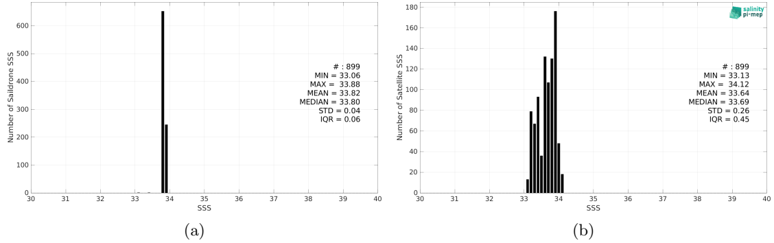
Figure 2: Histograms of SSS from Saildrone (a) and SMOS SSS L3 v2 - 9-Days (BEC) (b) considering all match-up pairs per bins of 0.1 over the South Atlantic Ocean Pi-MEP region and for the full satellite product period.
