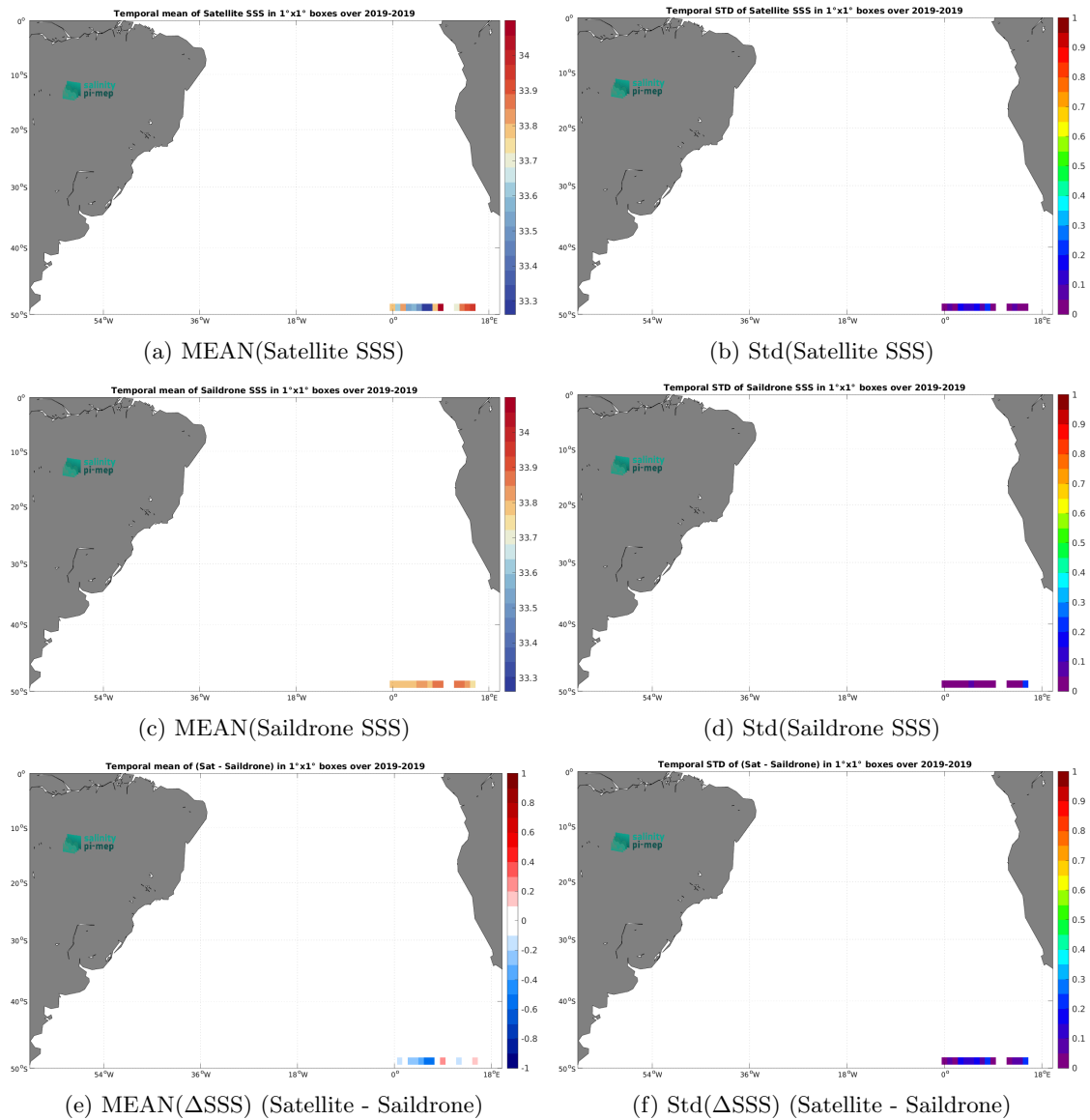
Figure 6: Temporal mean (left) and Std (right) of SSS from SMOS SSS L3 v2 - 9-Days (BEC) (top), Saildrone (middle), and of \Delta SSS (Satellite - Saildrone). Only match-up pairs are used to generate these maps.
