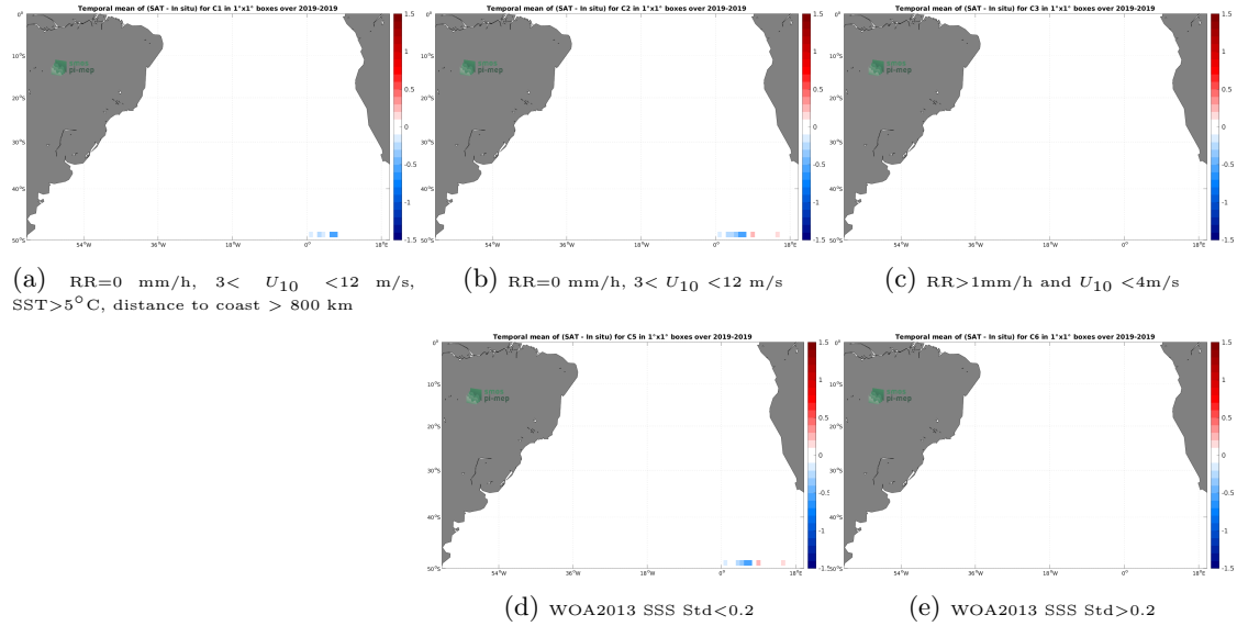
Figure 12: Temporal mean gridded over spatial boxes of size 1^{\circ} \times 1^{\circ} of \Delta\text{SSS} (SMOS SSS L3 v2 - 9-Days (BEC) - Saildrone) for 5 different subdatasets corresponding to: RR=0 mm/h, 3 < U_{10} < 12 m/s, SST > 5^{\circ}\text{C} , distance to coast > 800 km (a), RR=0 mm/h, 3 < U_{10} < 12 m/s (b), RR > 1 mm/h and U_{10} < 4 m/s (c), WOA2013 SSS Std < 0.2 (d), WOA2013 SSS Std > 0.2 (e).
