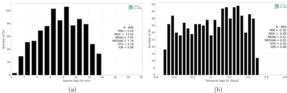
Figure 5: Histograms of the spatial (a) and temporal (b) lags between the location/time of the Sairdrone measurement and the date of the corresponding SMOS SSS L3 v2 - 9-Days (BEC) SSS pixel.
