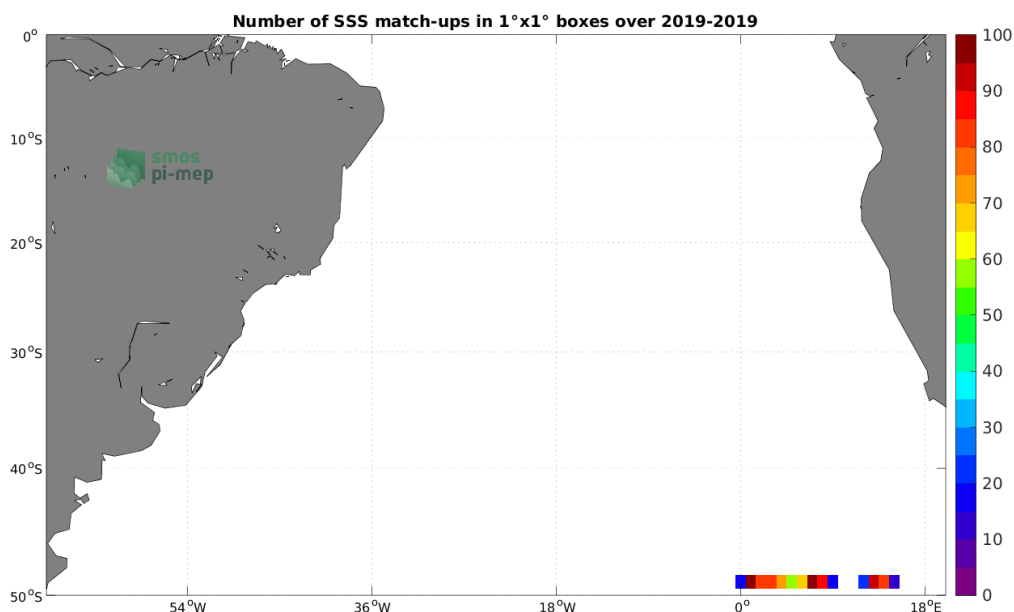
Figure 4: Number of SSS match-ups between Sairdrone SSS and the SMOS SSS L3 v2 - 9-Days (BEC) SSS product for the South Atlantic Ocean Pi-MEP region over 1^\circ \times 1^\circ boxes and for the full satellite product period.
