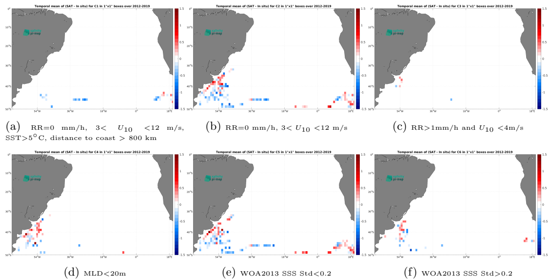
Figure 12: Temporal mean gridded over spatial boxes of size 1^\circ \times 1^\circ of \Delta SSS (SMOS SSS L3 v2 - 9-Days (BEC) - Marine mammals) for 6 different subdatasets corresponding to:RR=0 mm/h, 3 < U_{10} < 12 m/s, SST > 5^\circ\text{C} , distance to coast > 800 km (a), RR=0 mm/h, 3 < U_{10} < 12 m/s (b), RR > 1 mm/h and U_{10} < 4 m/s (c),MLD < 20 m (d),WOA2013 SSS Std < 0.2 (e),WOA2013 SSS Std > 0.2 (f).
