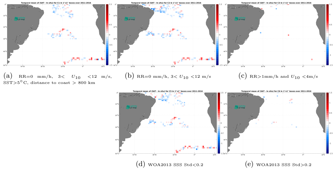
Figure 11: Temporal mean gridded over spatial boxes of size 1^\circ \times 1^\circ of \Delta SSS (SMOS SSS L3 v2 - 9-Days (BEC) - Surface drifters) for 5 different subdatasets corresponding to:RR=0 mm/h, 3 < U_{10} < 12 m/s, SST >5^\circ\text{C} , distance to coast > 800 km (a), RR=0 mm/h, 3 < U_{10} < 12 m/s (b), RR >1 mm/h and U_{10} < 4 m/s (c), WOA2013 SSS Std <0.2 (d), WOA2013 SSS Std >0.2 (e).
