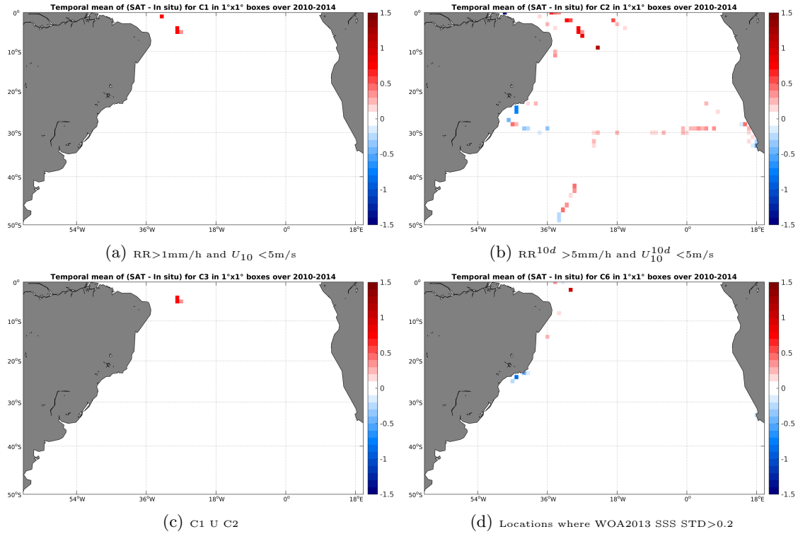
Figure 12: Temporal mean gridded over spatial boxes of size 1^\circ \times 1^\circ of \Delta SSS (SMOS-L3-BEC-OA-V1-9DAYS-0.25DEG - TSG-SAMOS) for 4 different subdatasets corresponding to: RR > 1mm/h and U_{10} < 5 m/s (a), RR^{10d} > 5 mm/h and U_{10}^{10d} < 5 m/s (b), C1 U C2 (c), Locations where WOA2013 SSS STD > 0.2 (d).
