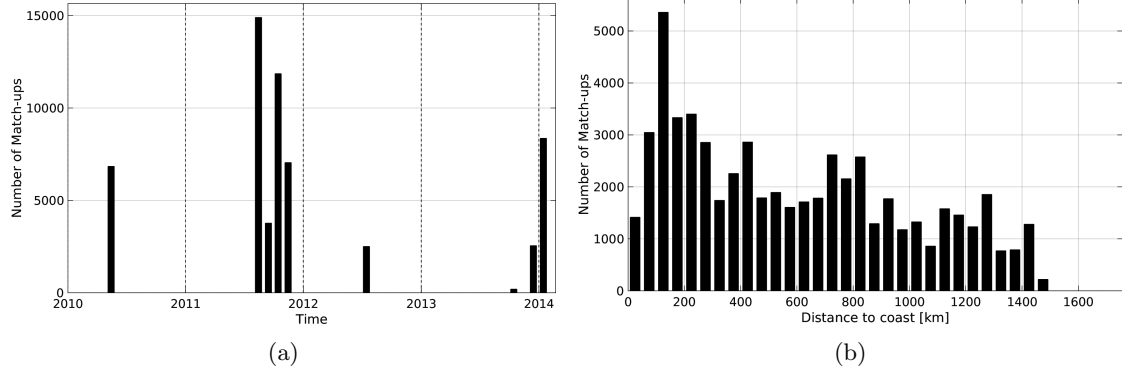
Figure 1: Number of match-ups between TSG-SAMOS and SMOS-L3-BEC-OA-V1-9DAYS-0.25DEG SSS as a function of time (a) and as function of the distance to coast (b) over the South Atlantic Ocean Pi-MEP region and for the full satellite product period.
