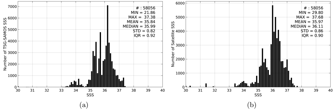
Figure 2: Histograms of SSS from TSG-SAMOS (a) and SMOS-L3-BEC-OA-V1-9DAYS-0.25DEG (b) considering all match-up pairs per bins of 0.1 over the South Atlantic Ocean Pi-MEP region and for the full satellite product period.
