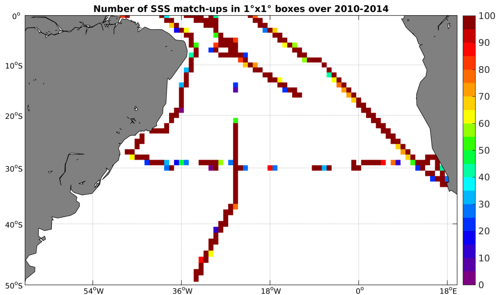
Figure 4: Number of SSS match-ups between TSG-SAMOS SSS and the SMOS-L3-BEC-OA-V1-9DAYS-0.25DEG SSS product for the South Atlantic Ocean Pi-MEP region over 1^\circ \times 1^\circ boxes and for the full satellite product period.
