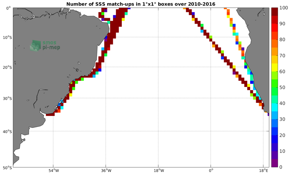
Figure 4: Number of SSS match-ups between TSG-LEGOS-DM SSS and the SMOS-L3-BEC-OA-V1-9DAYS-0.25DEG SSS product for the South Atlantic Ocean Pi-MEP region over 1^\circ \times 1^\circ boxes and for the full satellite product period.
