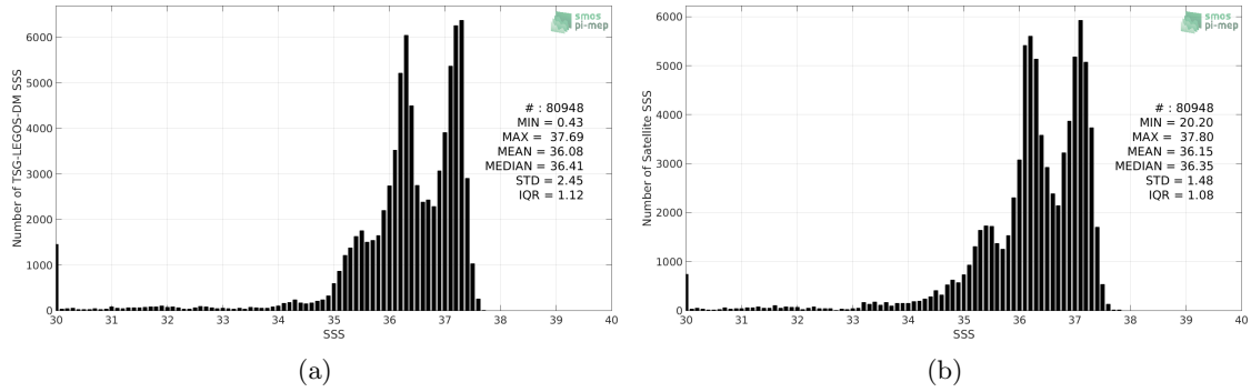
Figure 2: Histograms of SSS from TSG-LEGOS-DM (a) and SMOS-L3-BEC-OA-V1-9DAYS-0.25DEG (b) considering all match-up pairs per bins of 0.1 over the South Atlantic Ocean Pi-MEP region and for the full satellite product period.
