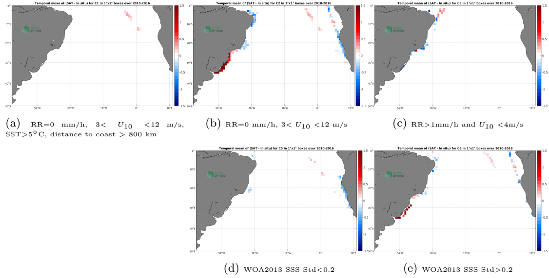
Figure 12: Temporal mean gridded over spatial boxes of size 1^\circ \times 1^\circ of \Delta SSS (SMOS-L3-BEC-OA-V1-9DAYS-0.25DEG - TSG-LEGOS-DM) for 5 different subdatasets corresponding to: RR=0 mm/h, 3 < U_{10} < 12 m/s, SST > 5^\circ C , distance to coast > 800 km (a), RR=0 mm/h, 3 < U_{10} < 12 m/s (b), RR > 1 mm/h and U_{10} < 4 m/s (c), WOA2013 SSS Std < 0.2 (d), WOA2013 SSS Std > 0.2 (e).
