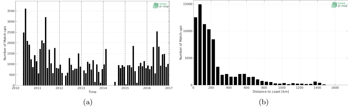
Figure 1: Number of match-ups between TSG-LEGOS-DM and SMOS-L3-BEC-OA-V1-9DAYS-0.25DEG SSS as a function of time (a) and as function of the distance to coast (b) over the South Atlantic Ocean Pi-MEP region and for the full satellite product period.
