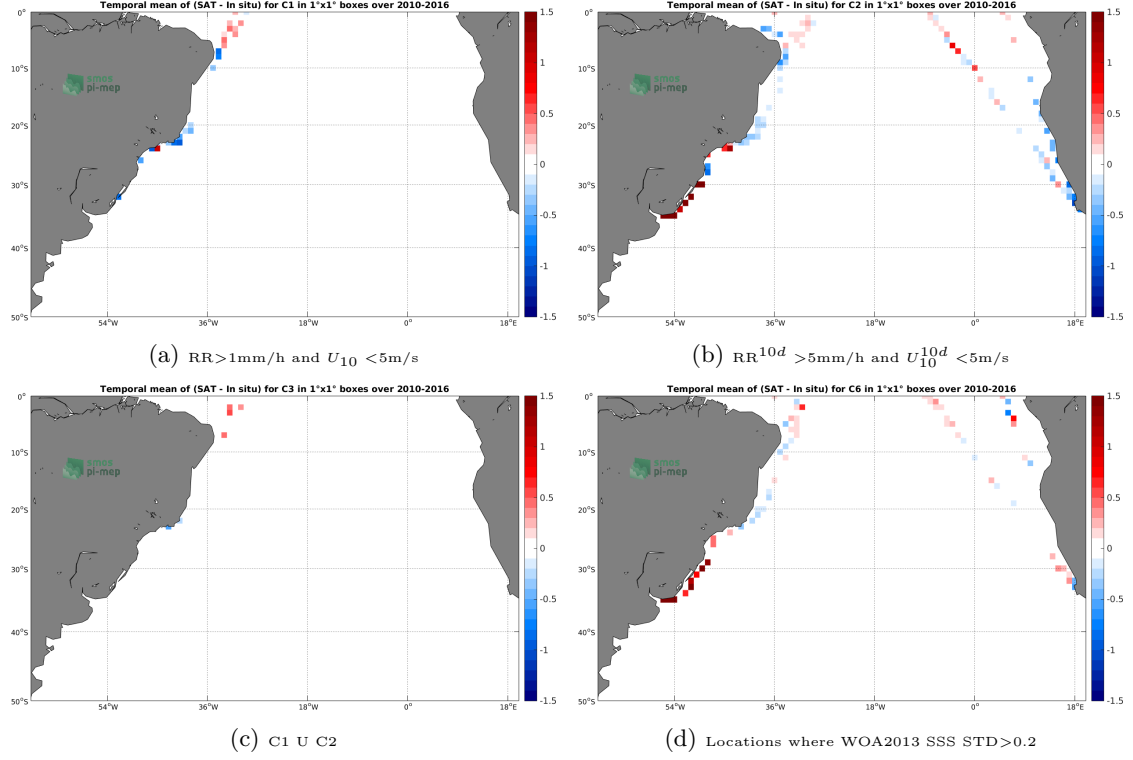
Figure 12: Temporal mean gridded over spatial boxes of size 1^\circ \times 1^\circ of \Delta SSS (SMOS-L3-BEC-OA-V1-9DAYS-0.25DEG - TSG-LEGOS-DM) for 4 different subdatasets corresponding to: RR > 1\text{mm/h} and U_{10} < 5\text{m/s} (a), RR^{10d} > 5\text{mm/h} and U_{10}^{10d} < 5\text{m/s} (b), C1 U C2 (c), Locations where WOA2013 SSS STD > 0.2 (d).
