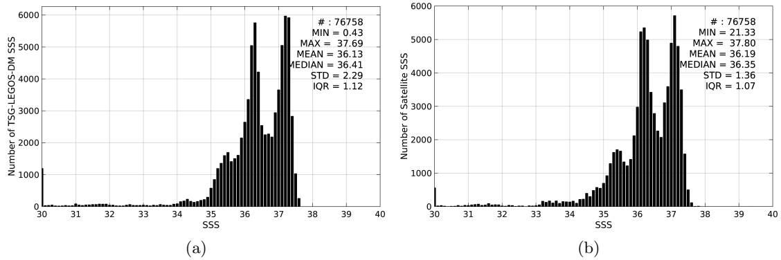
Figure 2: Histograms of SSS from TSG-LEGOS-DM (a) and SMOS-L3-BEC-OA-V1-9DAYS-0.25DEG (b) considering all match-up pairs per bins of 0.1 over the South Atlantic Ocean Pi-MEP region and for the full satellite product period.
