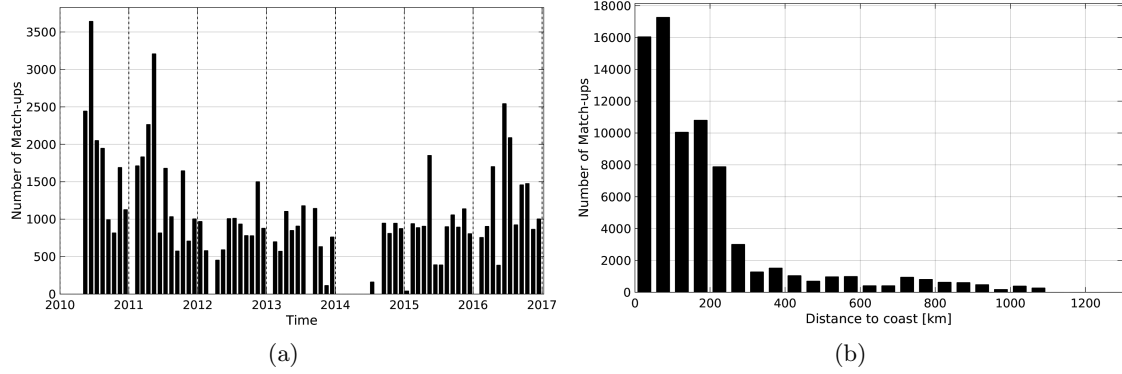
Figure 1: Number of match-ups between TSG-LEGOS-DM and SMOS-L3-BEC-OA-V1-9DAYS-0.25DEG SSS as a function of time (a) and as function of the distance to coast (b) over the South Atlantic Ocean Pi-MEP region and for the full satellite product period.
