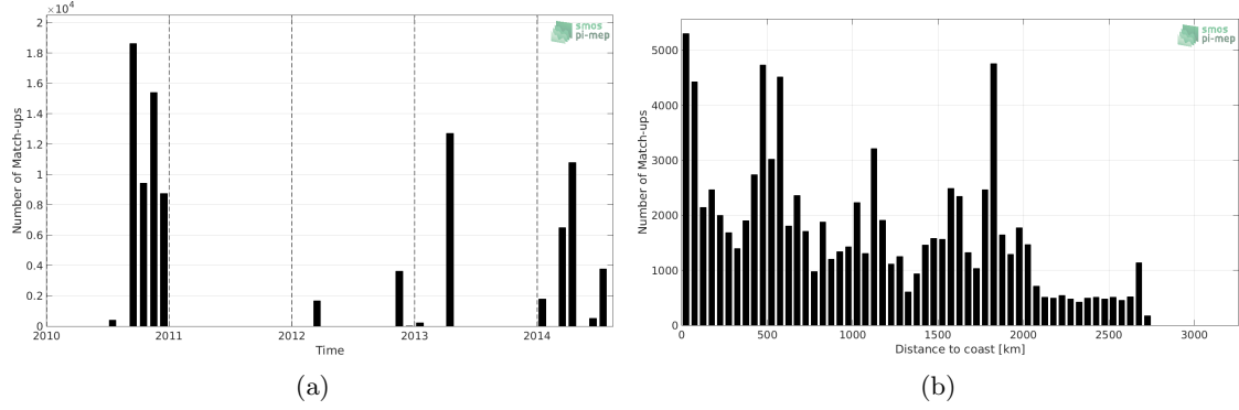
Figure 1: Number of match-ups between TSG-GOSUD-Sailing-ship and SMOS-L3-BEC-OA-V1-9DAYS-0.25DEG SSS as a function of time (a) and as function of the distance to coast (b) over the South Atlantic Ocean Pi-MEP region and for the full satellite product period.
