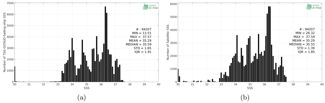
Figure 2: Histograms of SSS from TSG-GOSUD-Sailing-ship (a) and SMOS-L3-BEC-OA-V1-9DAYS-0.25DEG (b) considering all match-up pairs per bins of 0.1 over the South Atlantic Ocean Pi-MEP region and for the full satellite product period.
