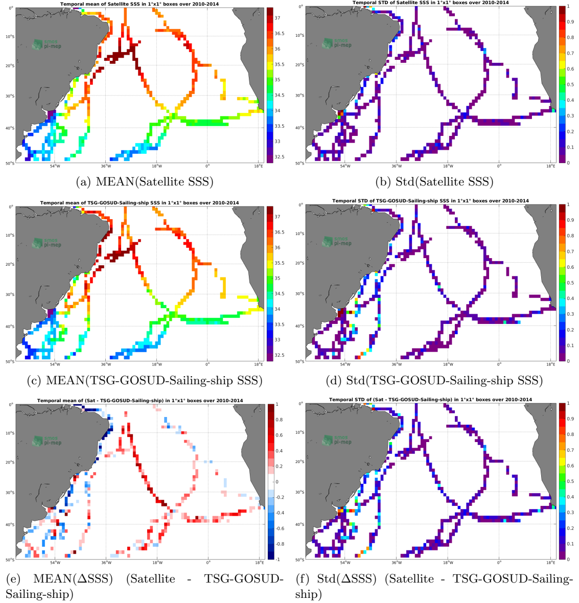
Figure 6: Temporal mean (left) and Std (right) of SSS from SMOS-L3-BEC-OA-V1-9DAYS-0.25DEG (top), TSG-GOSUD-Sailing-ship (middle), and of \Delta SSS (Satellite - TSG-GOSUD-Sailing-ship). Only match-up pairs are used to generate these maps.
