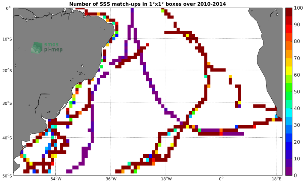
Figure 4: Number of SSS match-ups between TSG-GOSUD-Sailing-ship SSS and the SMOS-L3-BEC-OA-V1-9DAYS-0.25DEG SSS product for the South Atlantic Ocean Pi-MEP region over 1^\circ \times 1^\circ boxes and for the full satellite product period.
