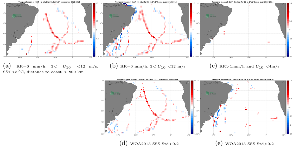
Figure 12: Temporal mean gridded over spatial boxes of size 1^\circ \times 1^\circ of \Delta SSS (SMOS-L3-BEC-OA-V1-9DAYS-0.25DEG - TSG-GOSUD-Sailing-ship) for 5 different subdatasets corresponding to: RR=0 mm/h, 3 < U_{10} < 12 m/s, SST >5^\circ\text{C} , distance to coast > 800 km (a), RR=0 mm/h, 3 < U_{10} < 12 m/s (b), RR >1 mm/h and U_{10} < 4 m/s (c), WOA2013 SSS Std <0.2 (d), WOA2013 SSS Std >0.2 (e).
