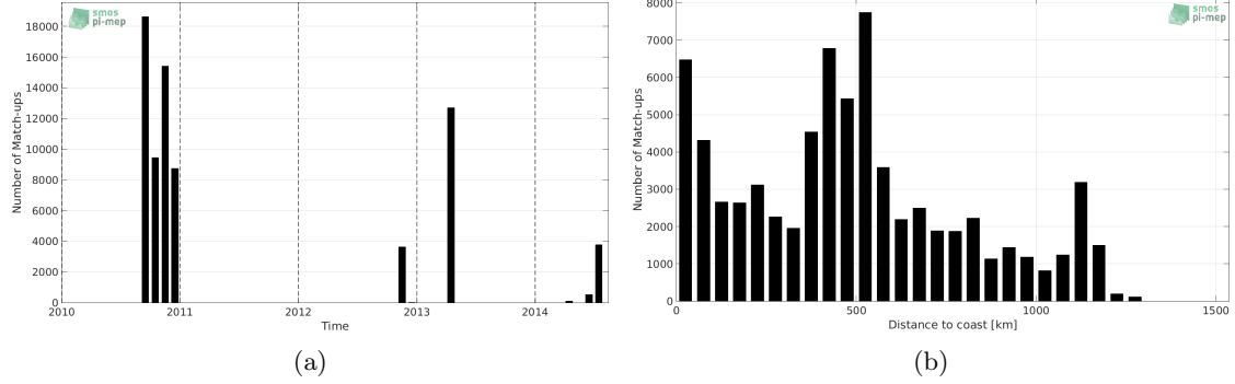
Figure 1: Number of match-ups between TSG-GOSUD-Sailing-ship and SMOS-L3-BEC-OA-V1-9DAYS-0.25DEG SSS as a function of time (a) and as function of the distance to coast (b) over the South Atlantic Ocean Pi-MEP region and for the full satellite product period.
