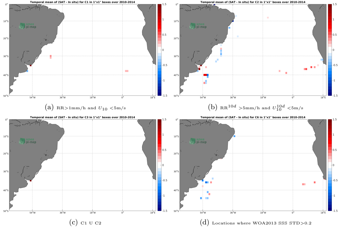
Figure 12: Temporal mean gridded over spatial boxes of size 1^\circ \times 1^\circ of \Delta SSS (SMOS-L3-BEC-OA-V1-9DAYS-0.25DEG - TSG-GOSUD-Sailing-ship) for 4 different subdatasets corresponding to: RR > 1mm/h and U_{10} < 5\text{m/s} (a), RR^{10d} > 5\text{mm/h} and U_{10}^{10d} < 5\text{m/s} (b), C1 U C2 (c), Locations where WOA2013 SSS STD > 0.2 (d).
