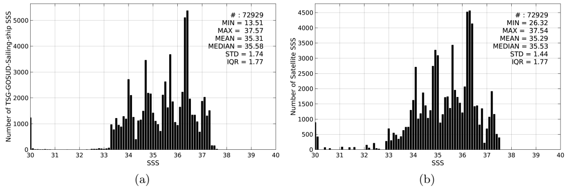
Figure 2: Histograms of SSS from TSG-GOSUD-Sailing-ship (a) and SMOS-L3-BEC-OA-V1-9DAYS-0.25DEG (b) considering all match-up pairs per bins of 0.1 over the South Atlantic Ocean Pi-MEP region and for the full satellite product period.
