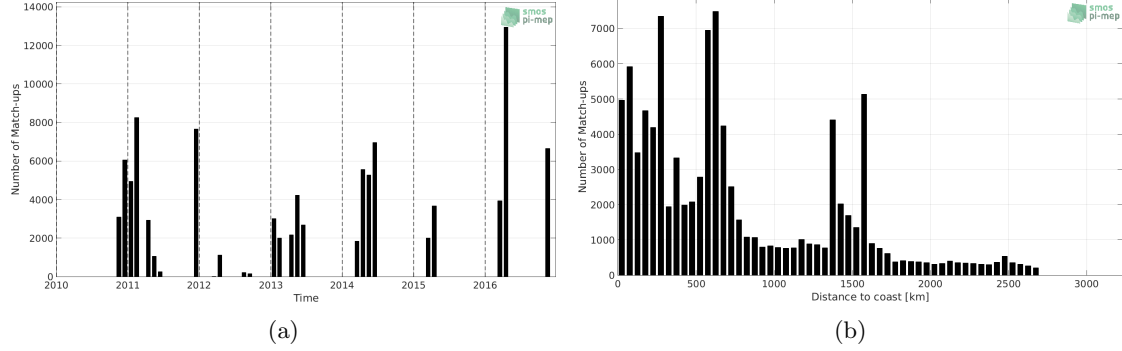
Figure 1: Number of match-ups between TSG-GOSUD-Research-vessel and SMOS-L3-BEC-OA-V1-9DAYS-0.25DEG SSS as a function of time (a) and as function of the distance to coast (b) over the South Atlantic Ocean Pi-MEP region and for the full satellite product period.
