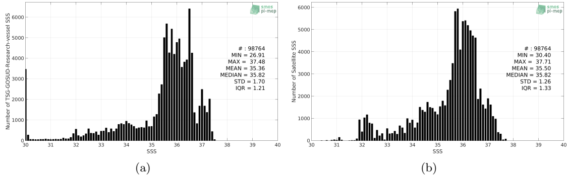
Figure 2: Histograms of SSS from TSG-GOSUD-Research-vessel (a) and SMOS-L3-BEC-OA-V1-9DAYS-0.25DEG (b) considering all match-up pairs per bins of 0.1 over the South Atlantic Ocean Pi-MEP region and for the full satellite product period.
