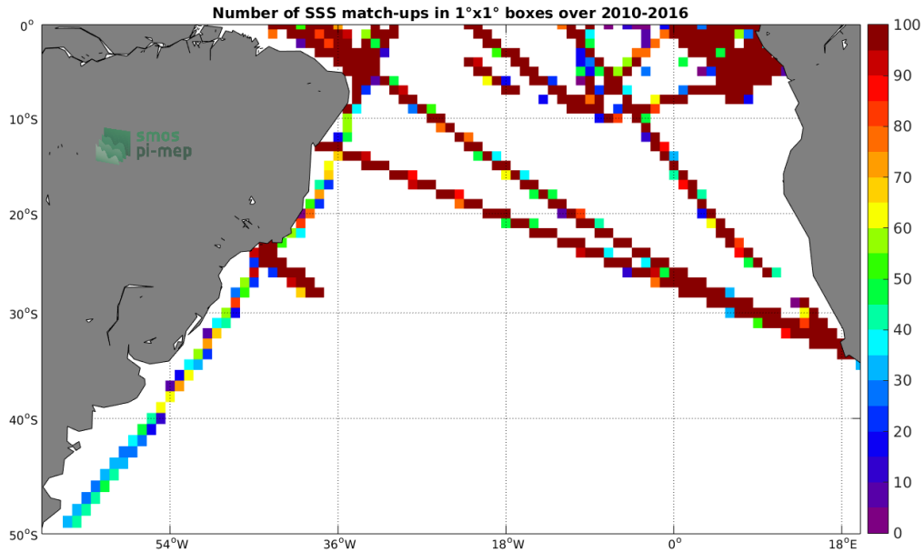
Figure 4: Number of SSS match-ups between TSG-GOSUD-Research-vessel SSS and the SMOS-L3-BEC-OA-V1-9DAYS-0.25DEG SSS product for the South Atlantic Ocean Pi-MEP region over 1°x1° boxes and for the full satellite product period.
