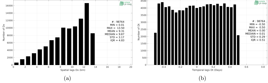
Figure 5: Histograms of the spatial (a) and temporal (b) lags between the time of the TSG-GOSUD-Research-vessel measurements and the date of the corresponding SMOS-L3-BEC-OA-V1-9DAYS-0.25DEG SSS product.
