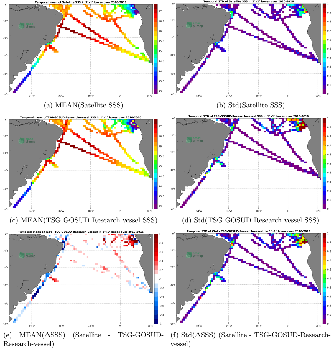
Figure 6: Temporal mean (left) and Std (right) of SSS from SMOS-L3-BEC-OA-V1-9DAYS-0.25DEG (top), TSG-GOSUD-Research-vessel (middle), and of \Delta SSS (Satellite - TSG-GOSUD-Research-vessel). Only match-up pairs are used to generate these maps.
