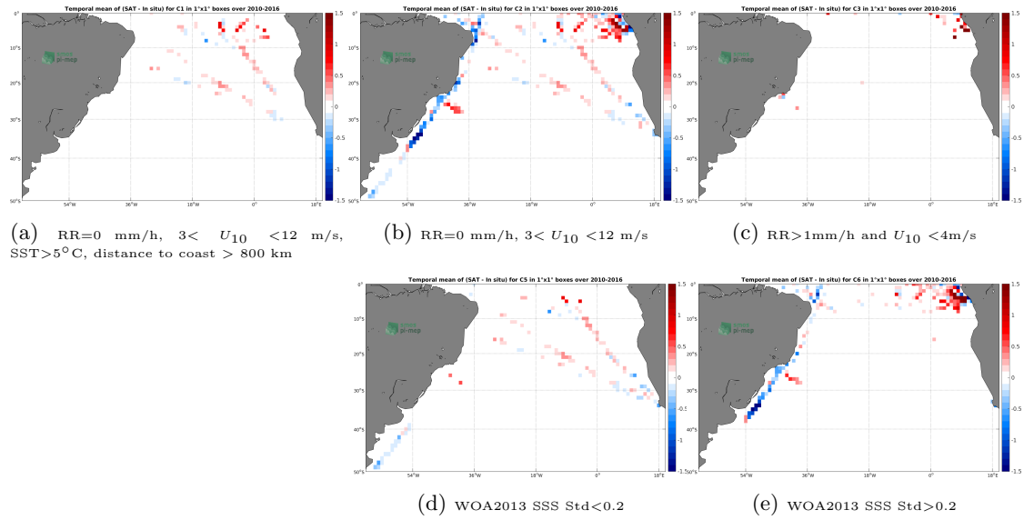
Figure 12: Temporal mean gridded over spatial boxes of size 1^\circ \times 1^\circ of \Delta SSS (SMOS-L3-BEC-OA-V1-9DAYS-0.25DEG - TSG-GOSUD-Research-vessel) for 5 different subdatasets corresponding to: RR=0 mm/h, 3 < U_{10} < 12 m/s, SST > 5^\circ C , distance to coast > 800 km (a), RR=0 mm/h, 3 < U_{10} < 12 m/s (b), RR > 1 mm/h and U_{10} < 4 m/s (c), WOA2013 SSS Std < 0.2 (d), WOA2013 SSS Std > 0.2 (e).
