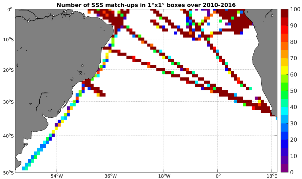
Figure 4: Number of SSS match-ups between TSG-GOSUD-Research-vessel SSS and the SMOS-L3-BEC-OA-V1-9DAYS-0.25DEG SSS product for the South Atlantic Ocean Pi-MEP region over 1^\circ \times 1^\circ boxes and for the full satellite product period.
