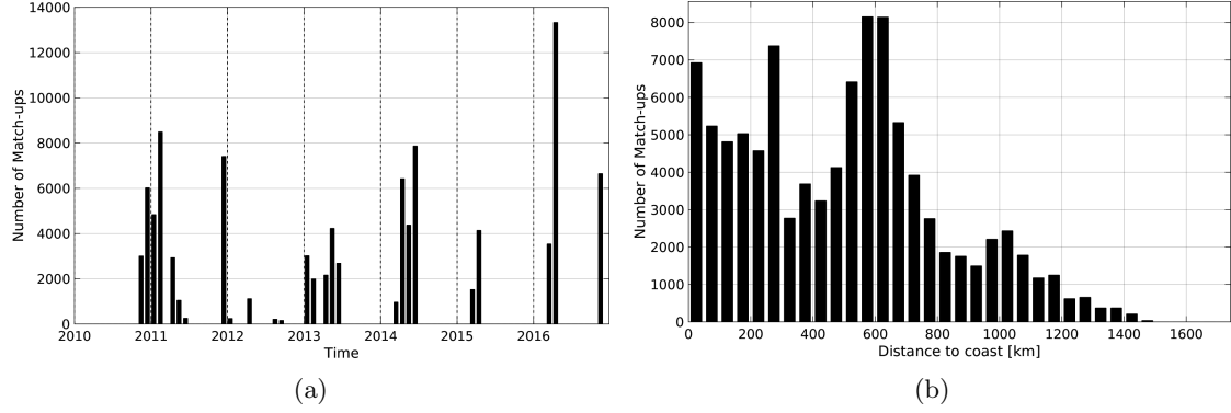
Figure 1: Number of match-ups between TSG-GOSUD-Research-vessel and SMOS-L3-BEC-OA-V1-9DAYS-0.25DEG SSS as a function of time (a) and as function of the distance to coast (b) over the South Atlantic Ocean Pi-MEP region and for the full satellite product period.
