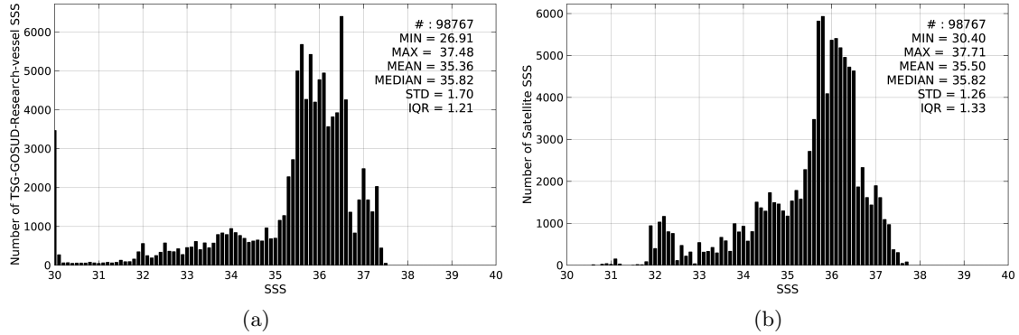
Figure 2: Histograms of SSS from TSG-GOSUD-Research-vessel (a) and SMOS-L3-BEC-OA-V1-9DAYS-0.25DEG (b) considering all match-up pairs per bins of 0.1 over the South Atlantic Ocean Pi-MEP region and for the full satellite product period.
