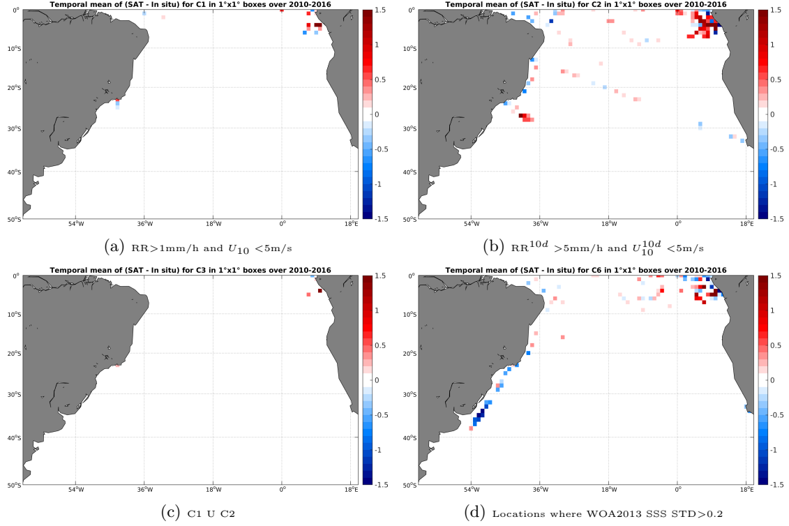
Figure 12: Temporal mean gridded over spatial boxes of size 1^\circ \times 1^\circ of \Delta SSS (SMOS-L3-BEC-OA-V1-9DAYS-0.25DEG - TSG-GOSUD-Research-vessel) for 4 different subdatasets corresponding to: RR > 1\text{mm/h} and U_{10} < 5\text{m/s} (a), RR^{10d} > 5\text{mm/h} and U_{10}^{10d} < 5\text{m/s} (b), C1 U C2 (c), Locations where WOA2013 SSS STD > 0.2 (d).
