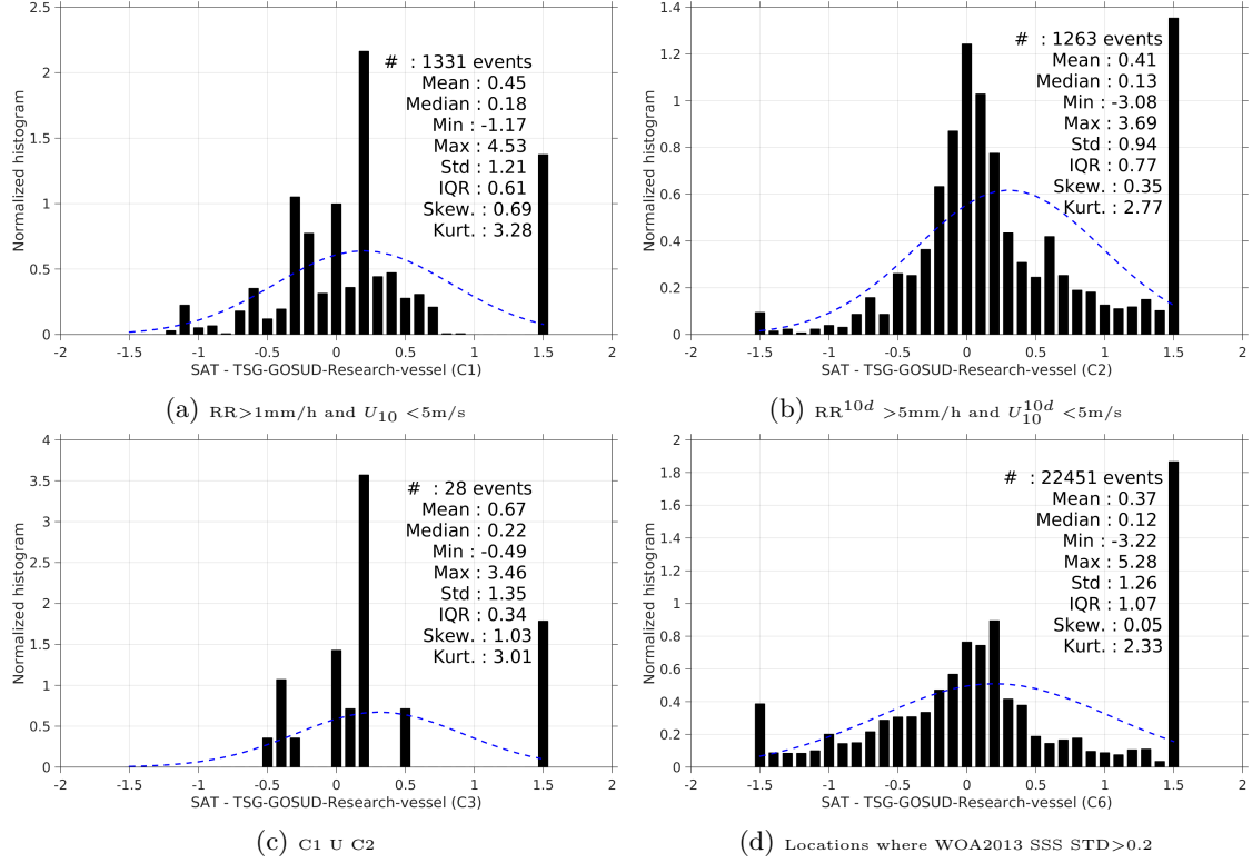
Figure 13: Normalized histogram of \Delta SSS (SMOS-L3-BEC-OA-V1-9DAYS-0.25DEG - TSG-GOSUD-Research-vessel) for 6 different subdatasets corresponding to: RR>1mm/h and U_{10} < 5\text{m/s} (a), RR^{10d} > 5\text{mm/h} and U_{10}^{10d} < 5\text{m/s} (b), C1 U C2 (c), Locations where WOA2013 SSS STD>0.2 (d).
