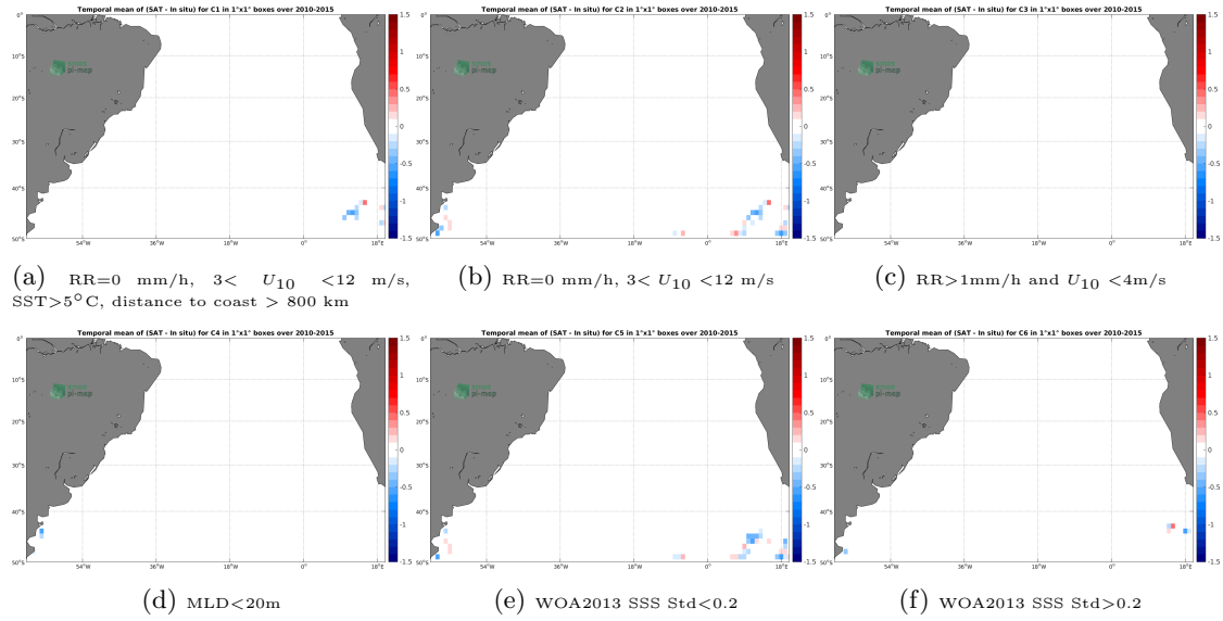
Figure 12: Temporal mean gridded over spatial boxes of size 1^\circ \times 1^\circ of \Delta SSS (SMOS-L3-BEC-OA-V1-9DAYS-0.25DEG - Sea mammals) for 6 different subdatasets corresponding to: RR=0 mm/h, 3 < U_{10} < 12 m/s, SST > 5^\circ C , distance to coast > 800 km (a), RR=0 mm/h, 3 < U_{10} < 12 m/s (b), RR > 1 mm/h and U_{10} < 4 m/s (c), MLD < 20 m (d), WOA2013 SSS Std < 0.2 (e), WOA2013 SSS Std > 0.2 (f).
