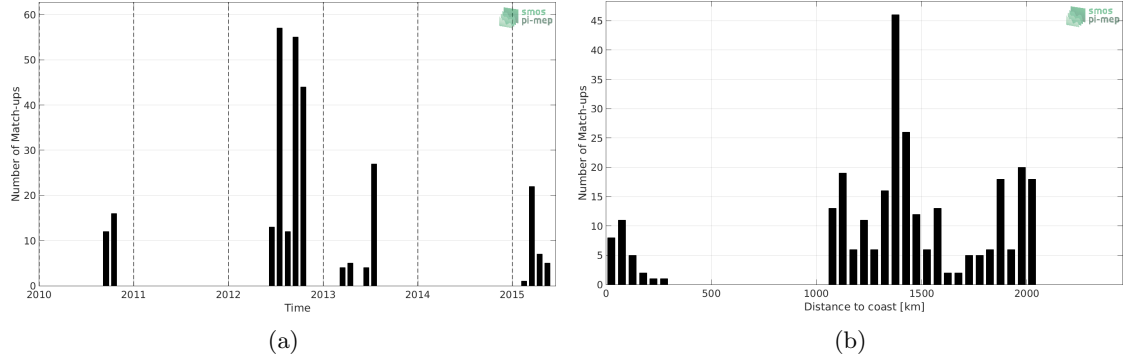
Figure 1: Number of match-ups between Sea mammals and SMOS-L3-BEC-OA-V1-9DAYS-0.25DEG SSS as a function of time (a) and as function of the distance to coast (b) over the South Atlantic Ocean Pi-MEP region and for the full satellite product period.
