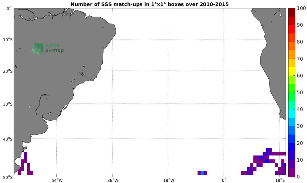
Figure 4: Number of SSS match-ups between Sea mammals SSS and the SMOS-L3-BEC-OA-V1-9DAYS-0.25DEG SSS product for the South Atlantic Ocean Pi-MEP region over 1°x1° boxes and for the full satellite product period.
