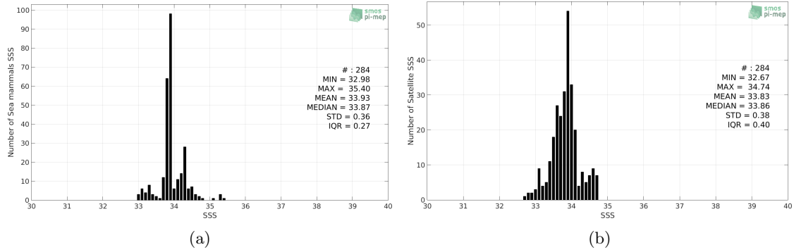
Figure 2: Histograms of SSS from Sea mammals (a) and SMOS-L3-BEC-OA-V1-9DAYS-0.25DEG (b) considering all match-up pairs per bins of 0.1 over the South Atlantic Ocean Pi-MEP region and for the full satellite product period.
