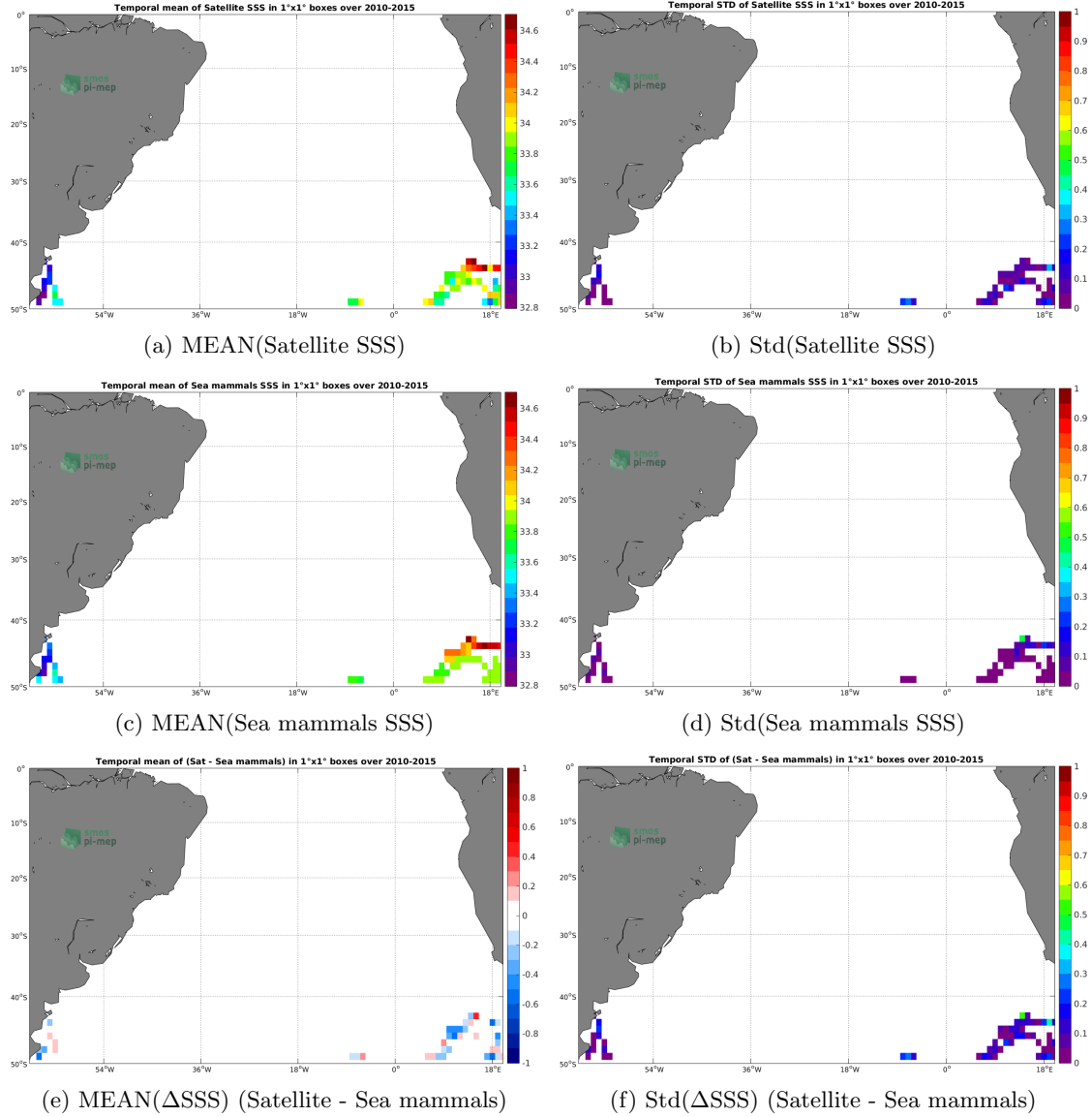
Figure 6: Temporal mean (left) and Std (right) of SSS from SMOS-L3-BEC-OA-V1-9DAYS-0.25DEG (top), Sea mammals (middle), and of \Delta SSS (Satellite - Sea mammals). Only match-up pairs are used to generate these maps.
