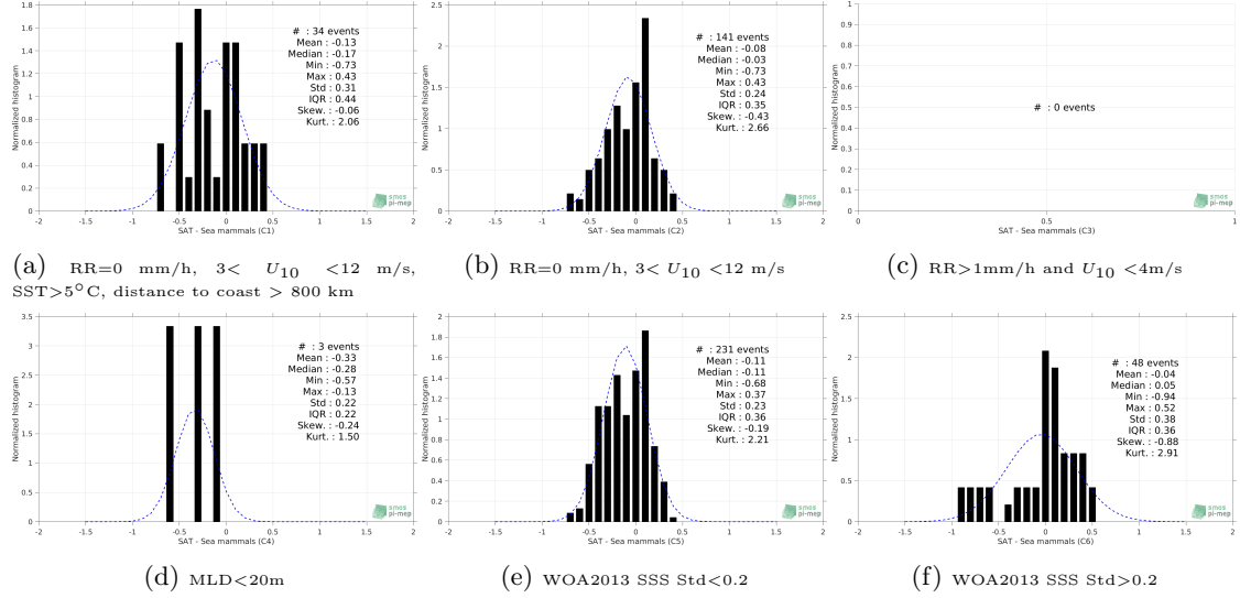
Figure 13: Normalized histogram of \Delta\text{SSS} (SMOS-L3-BEC-OA-V1-9DAYS-0.25DEG - Sea mammals) for 6 different subdatasets corresponding to: RR=0 mm/h, 3 < U_{10} < 12 m/s, SST > 5^\circ\text{C} , distance to coast > 800 km (a), RR=0 mm/h, 3 < U_{10} < 12 m/s (b), RR > 1 mm/h and U_{10} < 4 m/s (c), MLD < 20 m (d), WOA2013 SSS Std < 0.2 (e), WOA2013 SSS Std > 0.2 (f).
