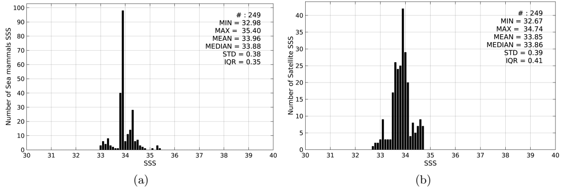
Figure 2: Histograms of SSS from Sea mammals (a) and SMOS-L3-BEC-OA-V1-9DAYS-0.25DEG (b) considering all match-up pairs per bins of 0.1 over the South Atlantic Ocean Pi-MEP region and for the full satellite product period.
