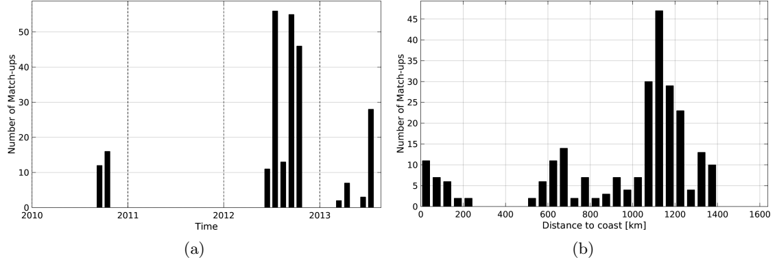
Figure 1: Number of match-ups between Sea mammals and SMOS-L3-BEC-OA-V1-9DAYS-0.25DEG SSS as a function of time (a) and as function of the distance to coast (b) over the South Atlantic Ocean Pi-MEP region and for the full satellite product period.
