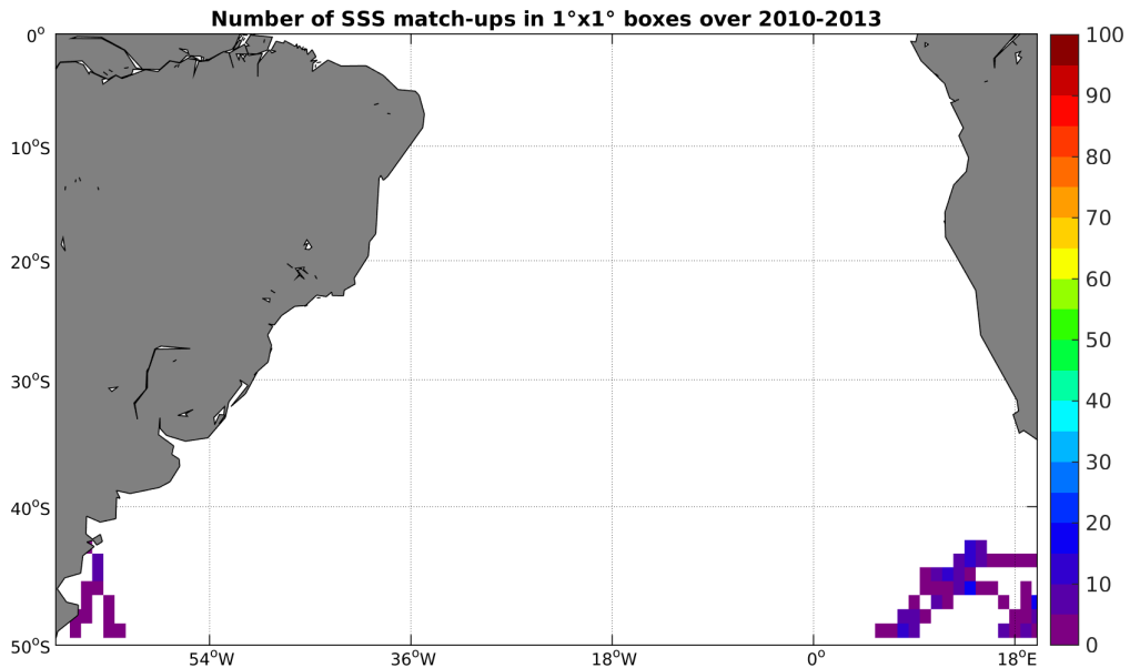
Figure 4: Number of SSS match-ups between Sea mammals SSS and the SMOS-L3-BEC-OA-V1-9DAYS-0.25DEG SSS product for the South Atlantic Ocean Pi-MEP region over 1^\circ \times 1^\circ boxes and for the full satellite product period.
