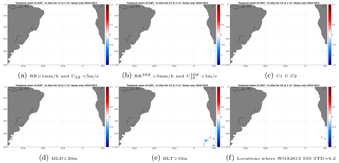
Figure 12: Temporal mean gridded over spatial boxes of size 1^\circ \times 1^\circ of \Delta SSS (SMOS-L3-BEC-OA-V1-9DAYS-0.25DEG - Sea mammals) for 6 different subdatasets corresponding to: RR > 1 mm/h and U_{10} < 5 m/s (a), RR^{10d} > 5 mm/h and U_{10}^{10d} < 5 m/s (b), C1 U C2 (c), MLD < 20 m (d), BLT > 10 m (e), Locations where WOA2013 SSS STD > 0.2 (f).
