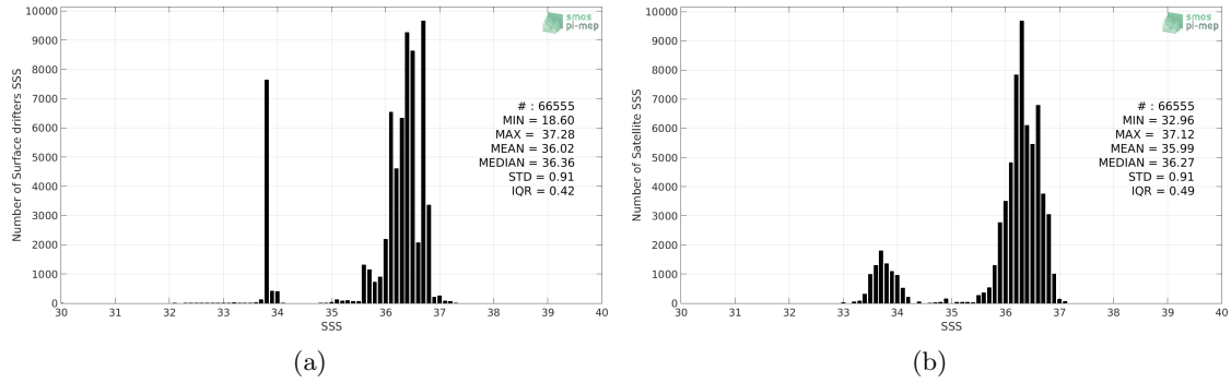
Figure 2: Histograms of SSS from Surface drifters (a) and SMOS-L3-BEC-OA-V1-9DAYS-0.25DEG (b) considering all match-up pairs per bins of 0.1 over the South Atlantic Ocean Pi-MEP region and for the full satellite product period.
