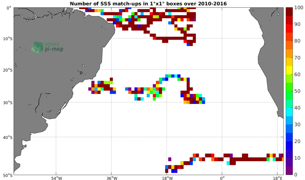
Figure 3: Number of SSS match-ups between Surface drifters SSS and the SMOS-L3-BEC-OA-V1-9DAYS-0.25DEG SSS product for the South Atlantic Ocean Pi-MEP region over 1^\circ \times 1^\circ boxes and for the full satellite product period.
