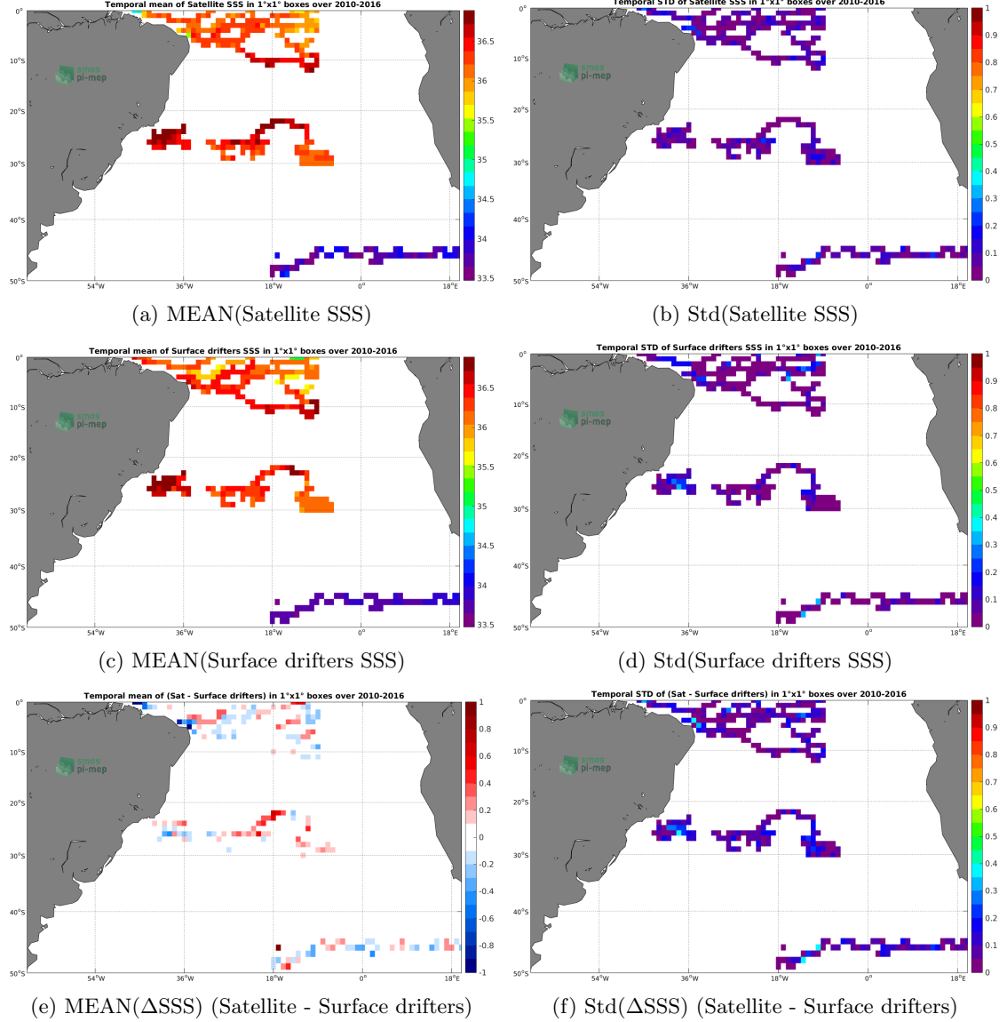
Figure 5: Temporal mean (left) and Std (right) of SSS from SMOS-L3-BEC-OA-V1-9DAYS-0.25DEG (top), Surface drifters (middle), and of \Delta SSS (Satellite - Surface drifters). Only match-up pairs are used to generate these maps.
