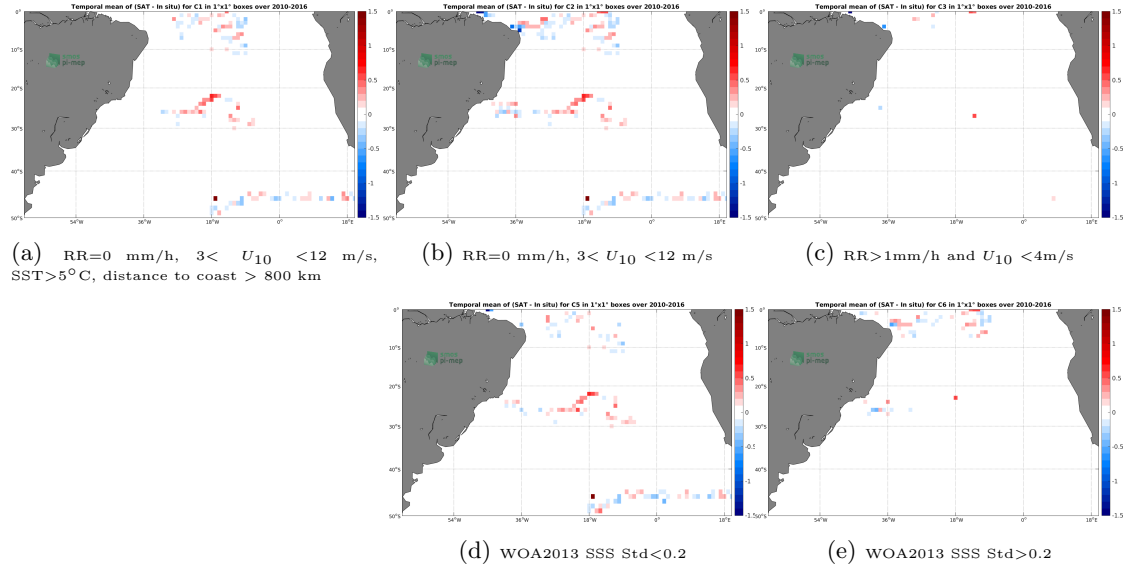
Figure 11: Temporal mean gridded over spatial boxes of size 1^\circ \times 1^\circ of \Delta SSS (SMOS-L3-BEC-OA-V1-9DAYS-0.25DEG - Surface drifters) for 5 different subdatasets corresponding to: RR=0 mm/h, 3 < U_{10} < 12 m/s, SST > 5^\circ C , distance to coast > 800 km (a), RR=0 mm/h, 3 < U_{10} < 12 m/s (b), RR > 1 mm/h and U_{10} < 4 m/s (c), WOA2013 SSS Std < 0.2 (d), WOA2013 SSS Std > 0.2 (e).
