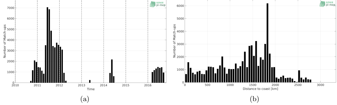
Figure 1: Number of match-ups between Surface drifters and SMOS-L3-BEC-OA-V1-9DAYS-0.25DEG SSS as a function of time (a) and as function of the distance to coast (b) over the South Atlantic Ocean Pi-MEP region and for the full satellite product period.
