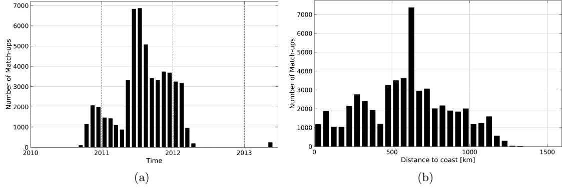
Figure 1: Number of match-ups between Surface drifters and SMOS-L3-BEC-OA-V1-9DAYS-0.25DEG SSS as a function of time (a) and as function of the distance to coast (b) over the South Atlantic Ocean Pi-MEP region and for the full satellite product period.
