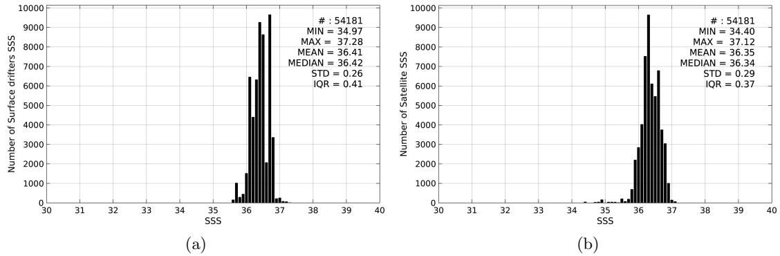
Figure 2: Histograms of SSS from Surface drifters (a) and SMOS-L3-BEC-OA-V1-9DAYS-0.25DEG (b) considering all match-up pairs per bins of 0.1 over the South Atlantic Ocean Pi-MEP region and for the full satellite product period.
