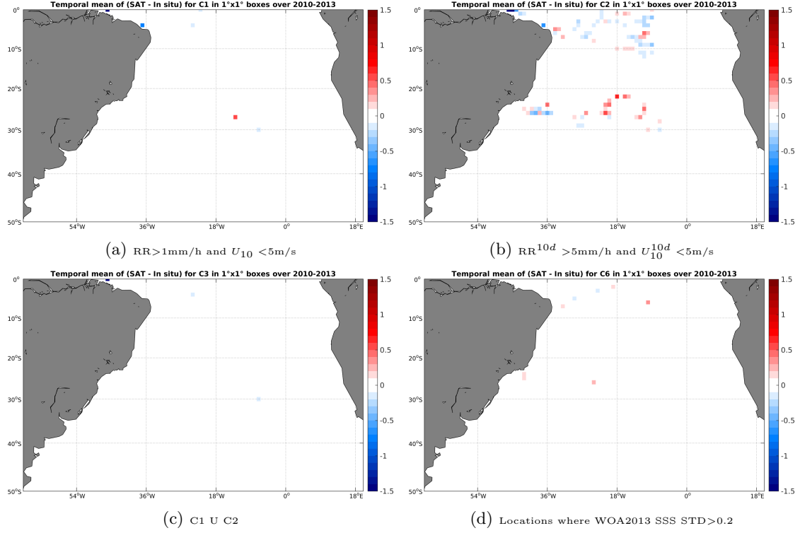
Figure 11: Temporal mean gridded over spatial boxes of size 1^\circ \times 1^\circ of \Delta SSS (SMOS-L3-BEC-OA-V1-9DAYS-0.25DEG - Surface drifters) for 4 different subdatasets corresponding to: RR > 1 mm/h and U_{10} < 5 m/s (a), RR^{10d} > 5 mm/h and U_{10}^{10d} < 5 m/s (b), C1 U C2 (c), Locations where WOA2013 SSS STD > 0.2 (d).
