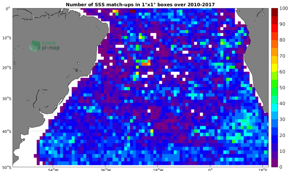
Figure 4: Number of SSS match-ups between Argo SSS and the SMOS-L3-BEC-OA-V1-9DAYS-0.25DEG SSS product for the South Atlantic Ocean Pi-MEP region over 1°x1° boxes and for the full satellite product period.
