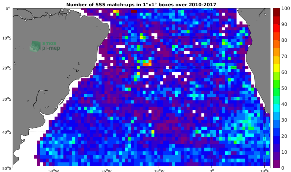
Figure 4: Number of SSS match-ups between Argo SSS and the SMOS-L3-BEC-OA-V1-9DAYS-0.25DEG SSS product for the South Atlantic Ocean Pi-MEP region over 1^\circ \times 1^\circ boxes and for the full satellite product period.
