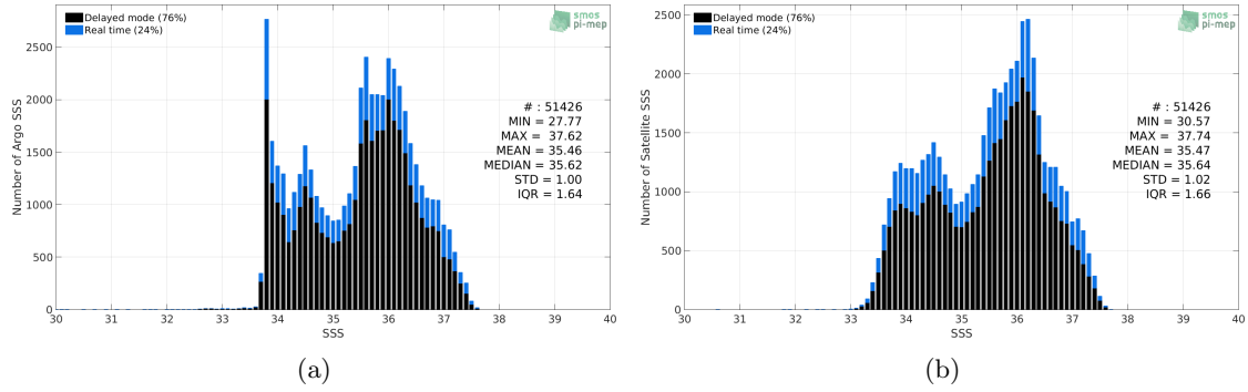
Figure 2: Histograms of SSS from Argo (a) and SMOS-L3-BEC-OA-V1-9DAYS-0.25DEG (b) considering all match-up pairs per bins of 0.1 over the South Atlantic Ocean Pi-MEP region and for the full satellite product period.
