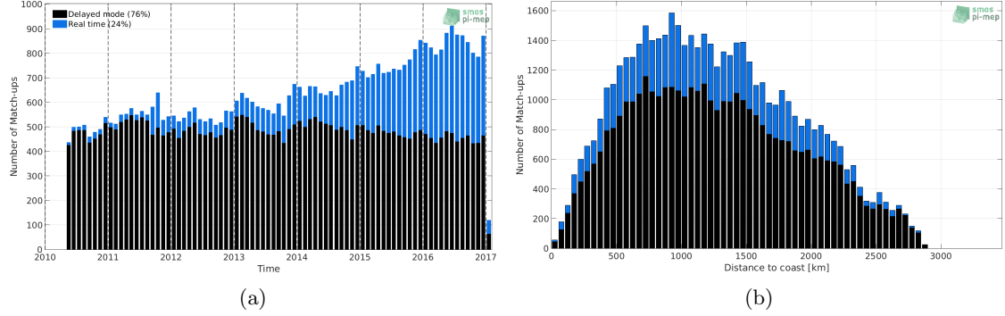
Figure 1: Number of match-ups between Argo and SMOS-L3-BEC-OA-V1-9DAYS-0.25DEG SSS as a function of time (a) and as function of the distance to coast (b) over the South Atlantic Ocean Pi-MEP region and for the full satellite product period.
