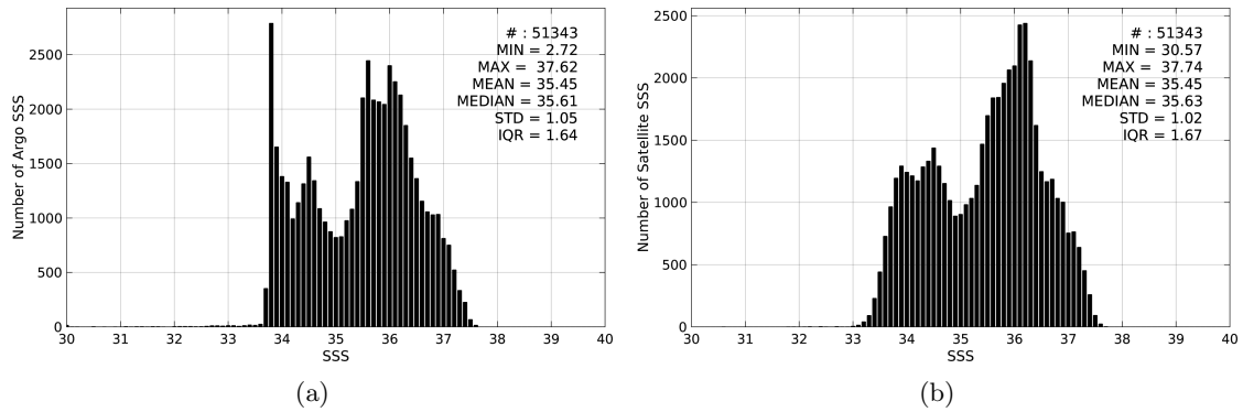
Figure 2: Histograms of SSS from Argo (a) and SMOS-L3-BEC-OA-V1-9DAYS-0.25DEG (b) considering all match-up pairs per bins of 0.1 over the South Atlantic Ocean Pi-MEP region and for the full satellite product period.
