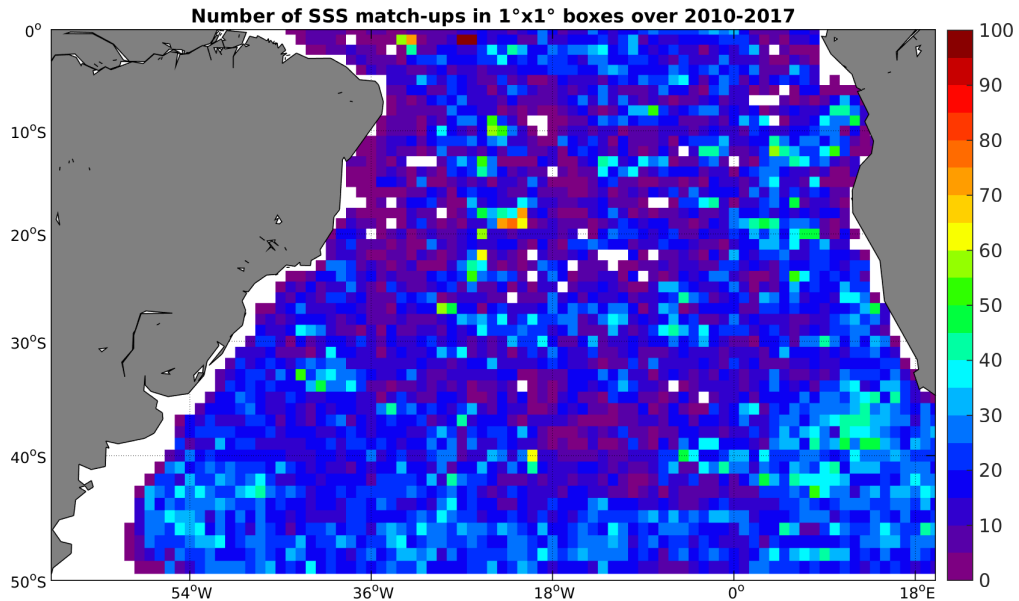
Figure 4: Number of SSS match-ups between Argo SSS and the SMOS-L3-BEC-OA-V1-9DAYS-0.25DEG SSS product for the South Atlantic Ocean Pi-MEP region over 1^\circ \times 1^\circ boxes and for the full satellite product period.
