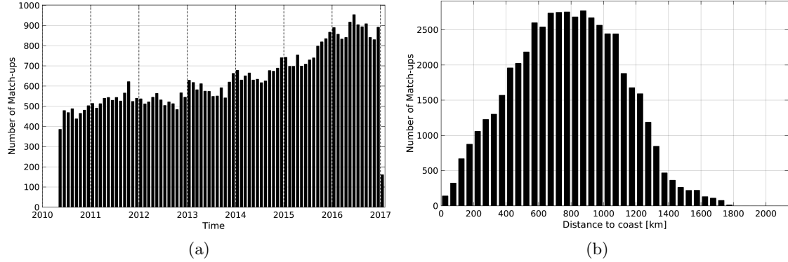
Figure 1: Number of match-ups between Argo and SMOS-L3-BEC-OA-V1-9DAYS-0.25DEG SSS as a function of time (a) and as function of the distance to coast (b) over the South Atlantic Ocean Pi-MEP region and for the full satellite product period.
