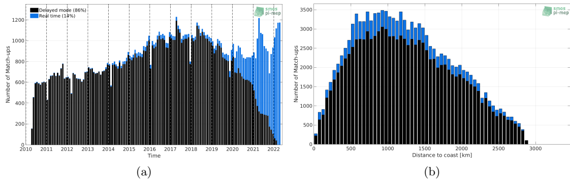
Figure 1: Number of match-ups between Argo and SMOS SSS L2-AVERAGED v700 (ESA) SSS as a function of time (a) and as function of the distance to coast (b) over the South Atlantic Ocean Pi-MEP region and for the full satellite product period.
