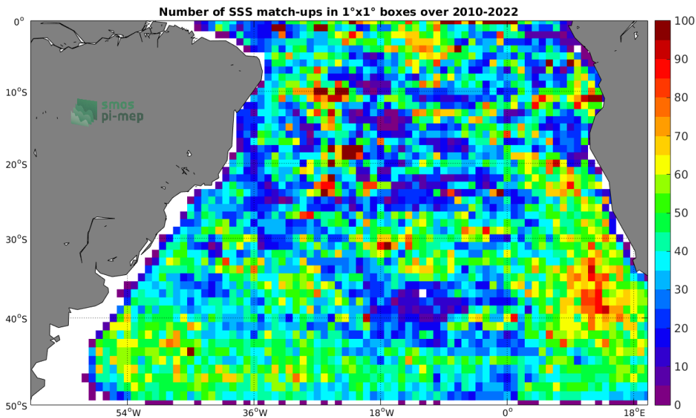
Figure 4: Number of SSS match-ups between Argo SSS and the SMOS SSS L2-AVERAGED v700 (ESA) SSS product for the South Atlantic Ocean Pi-MEP region over 1^\circ \times 1^\circ boxes and for the full satellite product period.
