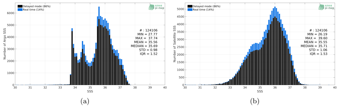
Figure 2: Histograms of SSS from Argo (a) and SMOS SSS L2-AVERAGED v700 (ESA) (b) considering all match-up pairs per bins of 0.1 over the South Atlantic Ocean Pi-MEP region and for the full satellite product period.
