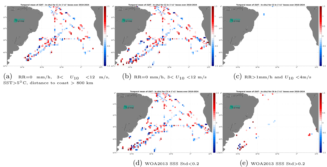
Figure 14: Temporal mean gridded over spatial boxes of size 1^\circ \times 1^\circ of \Delta\text{SSS} (SMOS SSS L2 v700 (ESA) - TSG (SAMOS)) for 5 different subdatasets corresponding to:RR=0 mm/h, 3 < U_{10} < 12 m/s, SST>5°C, distance to coast > 800 km (a), RR=0 mm/h, 3 < U_{10} < 12 m/s (b), RR>1mm/h and U_{10} < 4 m/s (c), WOA2013 SSS Std<0.2 (d), WOA2013 SSS Std>0.2 (e).
