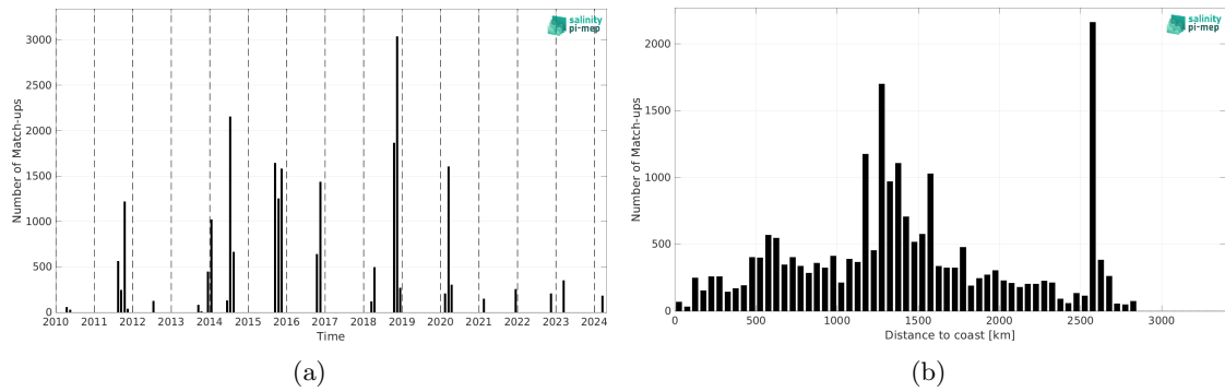
Figure 2: Number of match-ups between TSG (SAMOS) and SMOS SSS L2 v700 (ESA) SSS as a function of time (a) and as function of the distance to coast (b) over the South Atlantic Ocean Pi-MEP region and for the full satellite product period.
