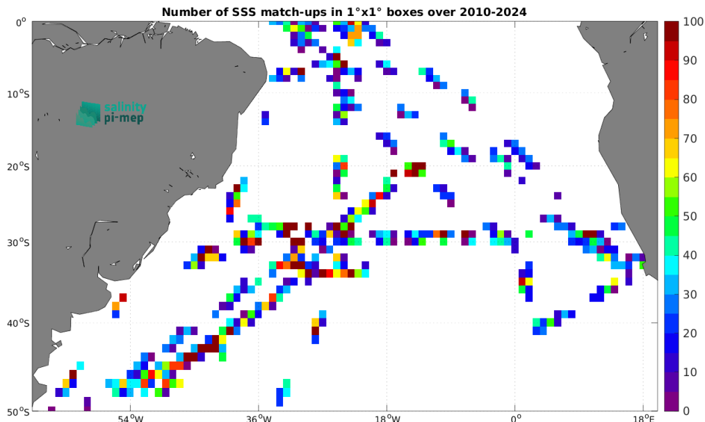
Figure 5: Number of SSS match-ups between TSG (SAMOS) SSS and the SMOS SSS L2 v700 (ESA) SSS product for the South Atlantic Ocean Pi-MEP region over 1^\circ \times 1^\circ boxes and for the full satellite product period.
