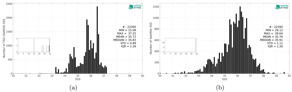
Figure 3: Histograms of SSS from TSG (SAMOS) (a) and SMOS SSS L2 v700 (ESA) (b) considering all match-up pairs per bins of 0.1 over the South Atlantic Ocean Pi-MEP region and for the full satellite product period.
