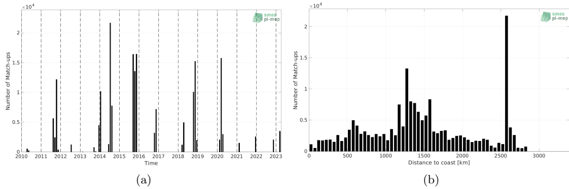
Figure 1: Number of match-ups between TSG (SAMOS) and SMOS SSS L2 v700 (ESA) SSS as a function of time (a) and as function of the distance to coast (b) over the South Atlantic Ocean Pi-MEP region and for the full satellite product period.
