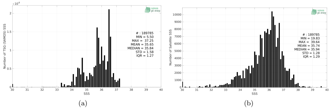
Figure 2: Histograms of SSS from TSG (SAMOS) (a) and SMOS SSS L2 v700 (ESA) (b) considering all match-up pairs per bins of 0.1 over the South Atlantic Ocean Pi-MEP region and for the full satellite product period.
