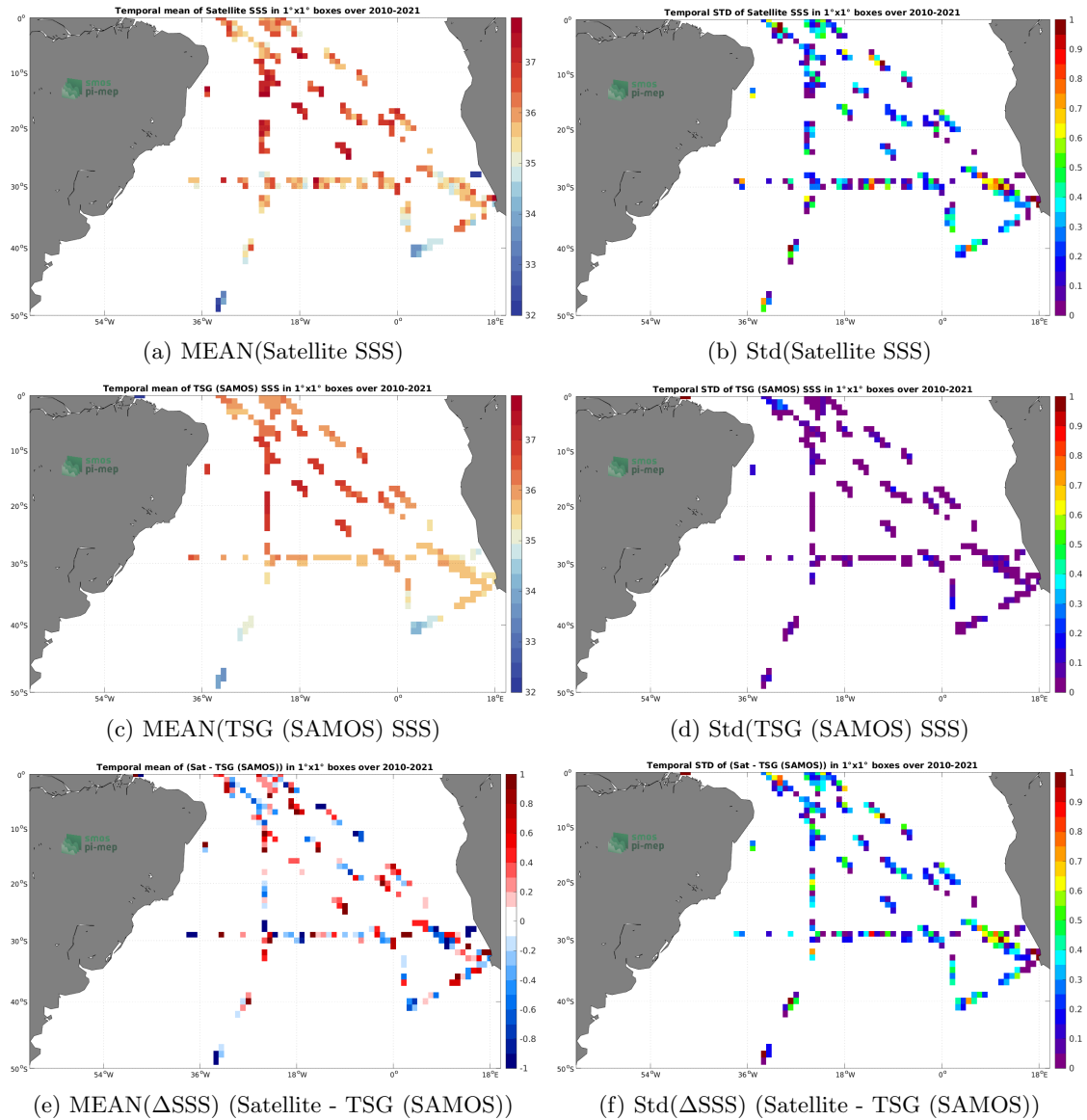
Figure 6: Temporal mean (left) and Std (right) of SSS from SMOS SSS L2 v700 (ESA) (top), TSG (SAMOS) (middle), and of \Delta SSS (Satellite - TSG (SAMOS)). Only match-up pairs are used to generate these maps.
