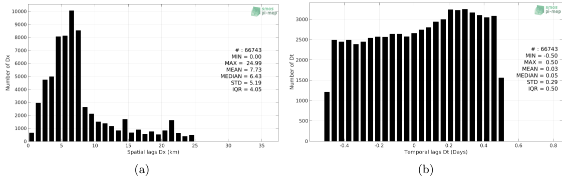
Figure 5: Histograms of the spatial (a) and temporal (b) lags between the location/time of the TSG (SAMOS) measurement and the date of the corresponding SMOS SSS L2 v700 (ESA) SSS pixel.
