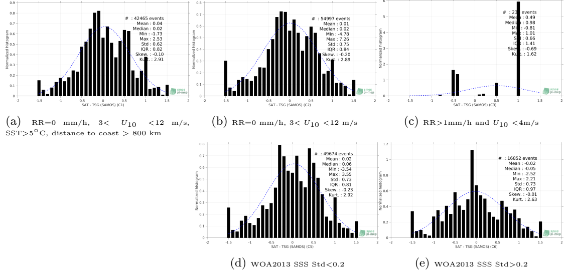
Figure 13: Normalized histogram of \Delta\text{SSS} (SMOS SSS L2 v700 (ESA) - TSG (SAMOS)) for 5 different subdatasets corresponding to: RR=0 mm/h, 3 < U_{10} < 12 m/s, SST > 5^\circ\text{C} , distance to coast > 800 km (a), RR=0 mm/h, 3 < U_{10} < 12 m/s (b), RR > 1\text{mm/h} and U_{10} < 4\text{m/s} (c), WOA2013 SSS Std < 0.2 (d), WOA2013 SSS Std > 0.2 (e).
