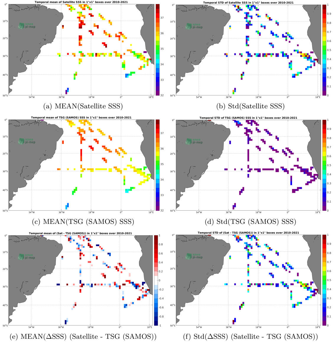
Figure 6: Temporal mean (left) and Std (right) of SSS from SMOS SSS L2 v700 (ESA) (top), TSG (SAMOS) (middle), and of \Delta SSS (Satellite - TSG (SAMOS)). Only match-up pairs are used to generate these maps.
