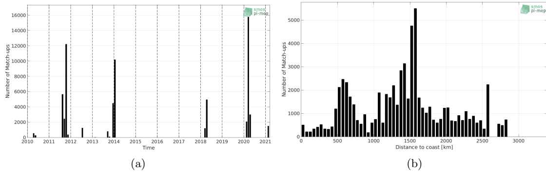
Figure 1: Number of match-ups between TSG (SAMOS) and SMOS SSS L2 v700 (ESA) SSS as a function of time (a) and as function of the distance to coast (b) over the South Atlantic Ocean Pi-MEP region and for the full satellite product period.
