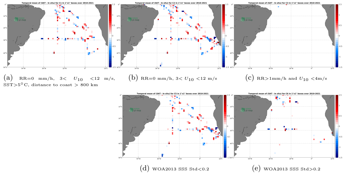
Figure 12: Temporal mean gridded over spatial boxes of size 1^\circ \times 1^\circ of \Delta SSS (SMOS SSS L2 v700 (ESA) - TSG (SAMOS)) for 5 different subdatasets corresponding to: RR=0 mm/h, 3 < U_{10} < 12 m/s, SST > 5^\circ C , distance to coast > 800 km (a), RR=0 mm/h, 3 < U_{10} < 12 m/s (b), RR > 1 mm/h and U_{10} < 4 m/s (c), WOA2013 SSS Std < 0.2 (d), WOA2013 SSS Std > 0.2 (e).
