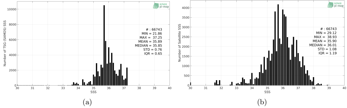
Figure 2: Histograms of SSS from TSG (SAMOS) (a) and SMOS SSS L2 v700 (ESA) (b) considering all match-up pairs per bins of 0.1 over the South Atlantic Ocean Pi-MEP region and for the full satellite product period.
