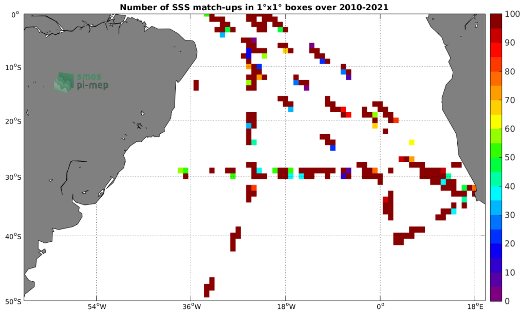
Figure 4: Number of SSS match-ups between TSG (SAMOS) SSS and the SMOS SSS L2 v700 (ESA) SSS product for the South Atlantic Ocean Pi-MEP region over 1^\circ \times 1^\circ boxes and for the full satellite product period.
