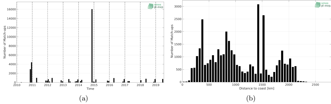
Figure 1: Number of match-ups between TSG (Polarstern) and SMOS SSS L2 v700 (ESA) SSS as a function of time (a) and as function of the distance to coast (b) over the South Atlantic Ocean Pi-MEP region and for the full satellite product period.
