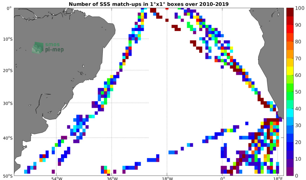
Figure 4: Number of SSS match-ups between TSG (Polarstern) SSS and the SMOS SSS L2 v700 (ESA) SSS product for the South Atlantic Ocean Pi-MEP region over 1^\circ \times 1^\circ boxes and for the full satellite product period.
