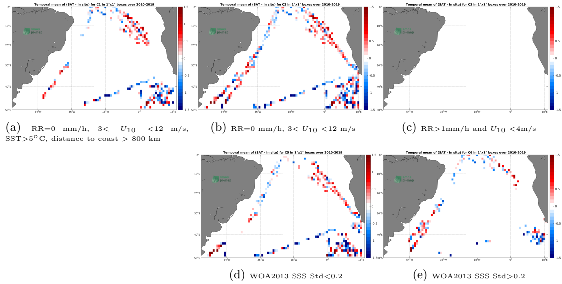
Figure 12: Temporal mean gridded over spatial boxes of size 1^\circ \times 1^\circ of \Delta SSS (SMOS SSS L2 v700 (ESA) - TSG (Polarstern)) for 5 different subdatasets corresponding to: RR=0 mm/h, 3 < U_{10} < 12 m/s, SST > 5^\circ C , distance to coast > 800 km (a), RR=0 mm/h, 3 < U_{10} < 12 m/s (b), RR > 1 mm/h and U_{10} < 4 m/s (c), WOA2013 SSS Std < 0.2 (d), WOA2013 SSS Std > 0.2 (e).
