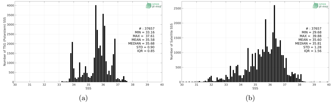
Figure 2: Histograms of SSS from TSG (Polarstern) (a) and SMOS SSS L2 v700 (ESA) (b) considering all match-up pairs per bins of 0.1 over the South Atlantic Ocean Pi-MEP region and for the full satellite product period.
