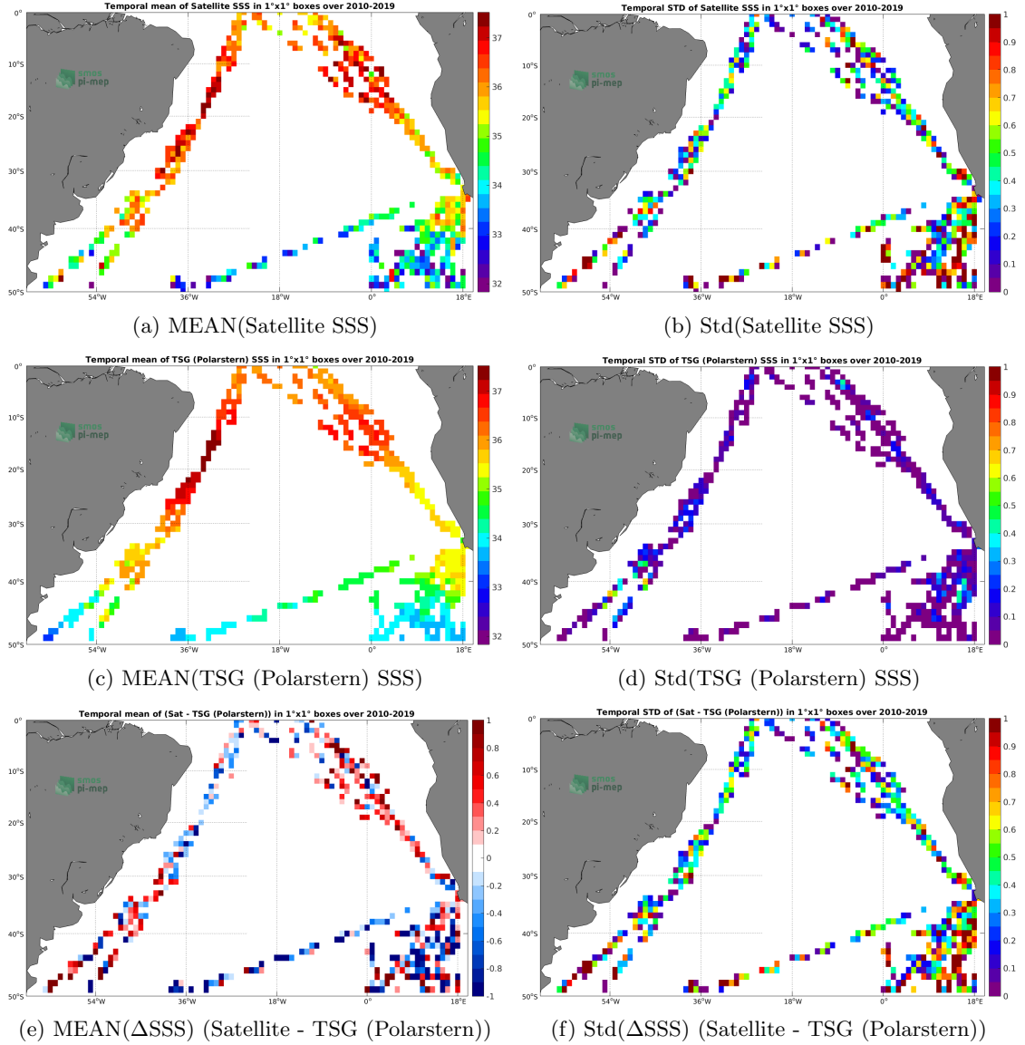
Figure 6: Temporal mean (left) and Std (right) of SSS from SMOS SSS L2 v700 (ESA) (top), TSG (Polarstern) (middle), and of \Delta SSS (Satellite - TSG (Polarstern)). Only match-up pairs are used to generate these maps.
