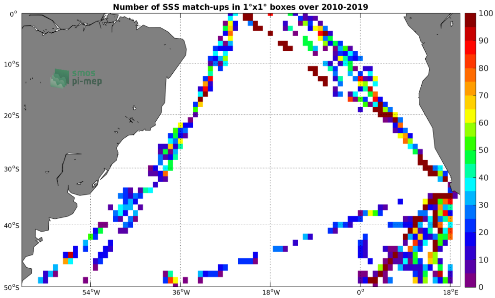
Figure 4: Number of SSS match-ups between TSG (Polarstern) SSS and the SMOS SSS L2 v700 (ESA) SSS product for the South Atlantic Ocean Pi-MEP region over 1^\circ \times 1^\circ boxes and for the full satellite product period.
