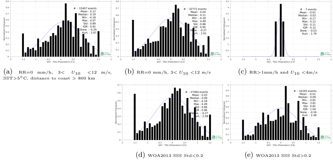
Figure 13: Normalized histogram of \Delta SSS (SMOS SSS L2 v700 (ESA) - TSG (Polarstern)) for 5 different subdatasets corresponding to: RR=0 mm/h, 3 < U_{10} < 12 m/s, SST>5°C, distance to coast > 800 km (a), RR=0 mm/h, 3 < U_{10} < 12 m/s (b), RR>1mm/h and U_{10} < 4 m/s (c), WOA2013 SSS Std<0.2 (d), WOA2013 SSS Std>0.2 (e).
