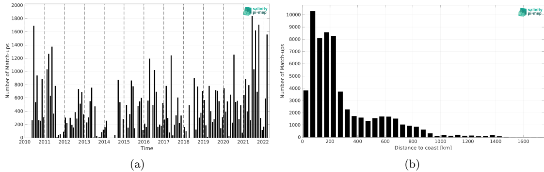
Figure 2: Number of match-ups between TSG (LEGOS-DM) and SMOS SSS L2 v700 (ESA) SSS as a function of time (a) and as function of the distance to coast (b) over the South Atlantic Ocean Pi-MEP region and for the full satellite product period.
