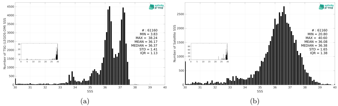
Figure 3: Histograms of SSS from TSG (LEGOS-DM) (a) and SMOS SSS L2 v700 (ESA) (b) considering all match-up pairs per bins of 0.1 over the South Atlantic Ocean Pi-MEP region and for the full satellite product period.
