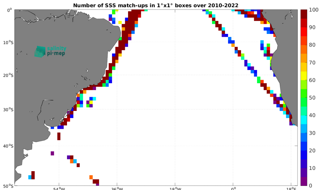
Figure 5: Number of SSS match-ups between TSG (LEGOS-DM) SSS and the SMOS SSS L2 v700 (ESA) SSS product for the South Atlantic Ocean Pi-MEP region over 1^\circ \times 1^\circ boxes and for the full satellite product period.
