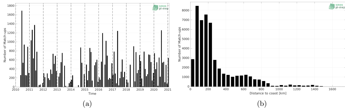
Figure 1: Number of match-ups between TSG (LEGOS-DM) and SMOS SSS L2 v700 (ESA) SSS as a function of time (a) and as function of the distance to coast (b) over the South Atlantic Ocean Pi-MEP region and for the full satellite product period.
