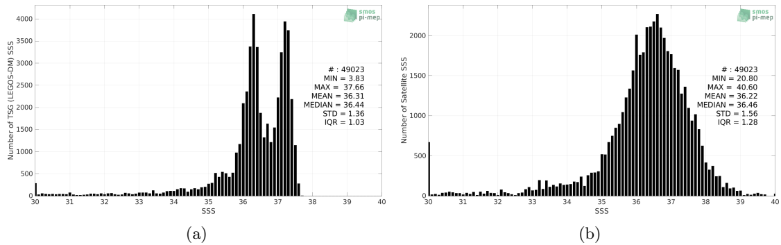
Figure 2: Histograms of SSS from TSG (LEGOS-DM) (a) and SMOS SSS L2 v700 (ESA) (b) considering all match-up pairs per bins of 0.1 over the South Atlantic Ocean Pi-MEP region and for the full satellite product period.
