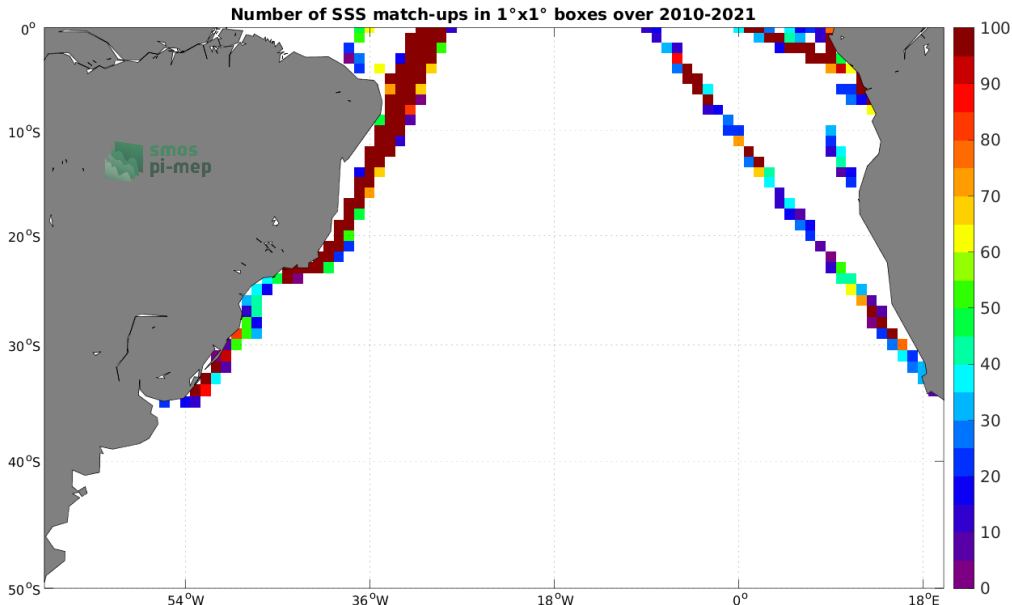
Figure 4: Number of SSS match-ups between TSG (LEGOS-DM) SSS and the SMOS SSS L2 v700 (ESA) SSS product for the South Atlantic Ocean Pi-MEP region over 1^\circ \times 1^\circ boxes and for the full satellite product period.
