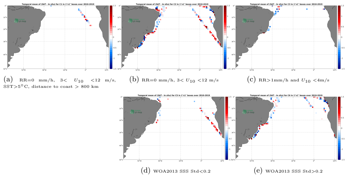
Figure 12: Temporal mean gridded over spatial boxes of size 1^\circ \times 1^\circ of \Delta SSS (SMOS SSS L2 v700 (ESA) - TSG (LEGOS-DM)) for 5 different subdatasets corresponding to: RR=0 mm/h, 3 < U_{10} < 12 m/s, SST > 5^\circ C , distance to coast > 800 km (a), RR=0 mm/h, 3 < U_{10} < 12 m/s (b), RR > 1 mm/h and U_{10} < 4 m/s (c), WOA2013 SSS Std < 0.2 (d), WOA2013 SSS Std > 0.2 (e).
