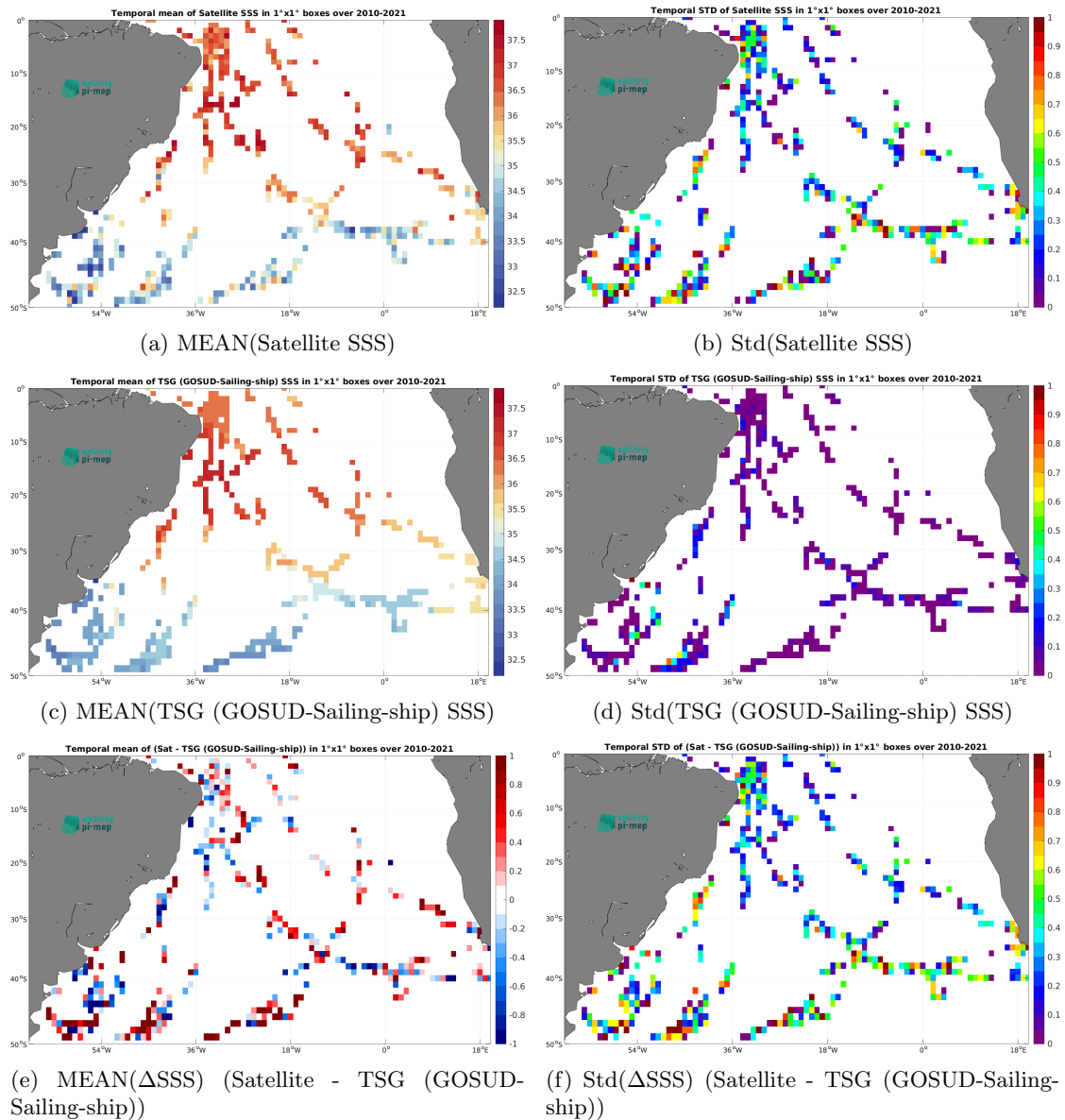
Figure 7: Temporal mean (left) and Std (right) of SSS from SMOS SSS L2 v700 (ESA) (top), TSG (GOSUD-Sailing-ship) (middle), and of \Delta SSS (Satellite - TSG (GOSUD-Sailing-ship)). Only match-up pairs are used to generate these maps.
