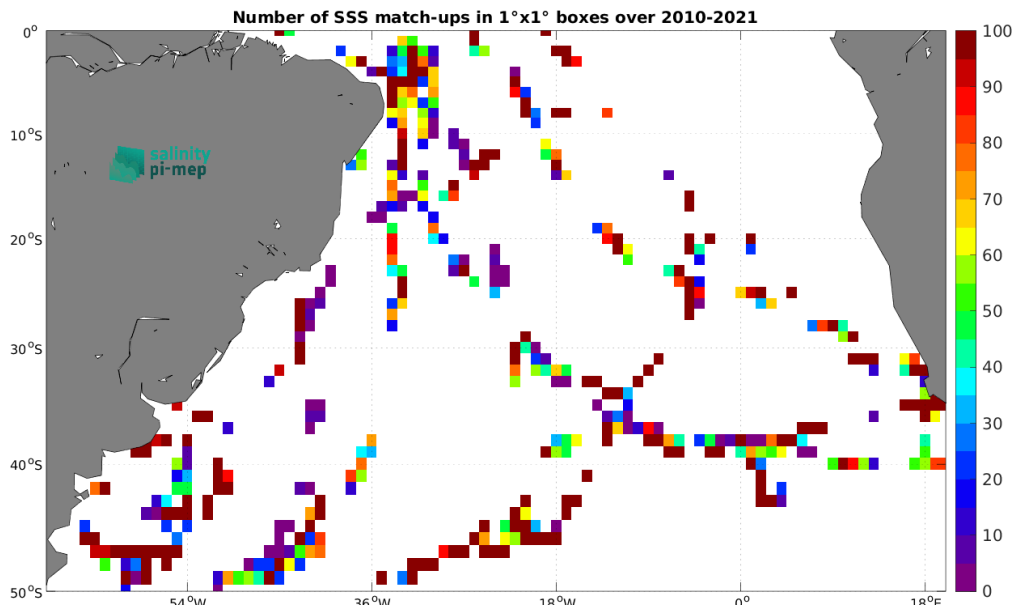
Figure 5: Number of SSS match-ups between TSG (GOSUD-Sailing-ship) SSS and the SMOS SSS L2 v700 (ESA) SSS product for the South Atlantic Ocean Pi-MEP region over 1^\circ \times 1^\circ boxes and for the full satellite product period.
