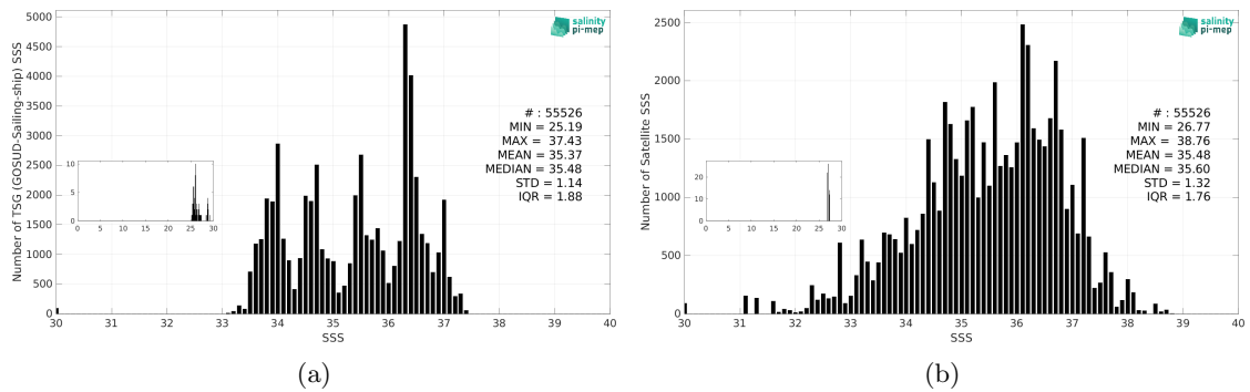
Figure 3: Histograms of SSS from TSG (GOSUD-Sailing-ship) (a) and SMOS SSS L2 v700 (ESA) (b) considering all match-up pairs per bins of 0.1 over the South Atlantic Ocean Pi-MEP region and for the full satellite product period.
