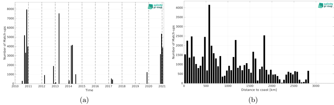
Figure 2: Number of match-ups between TSG (GOSUD-Sailing-ship) and SMOS SSS L2 v700 (ESA) SSS as a function of time (a) and as function of the distance to coast (b) over the South Atlantic Ocean Pi-MEP region and for the full satellite product period.
