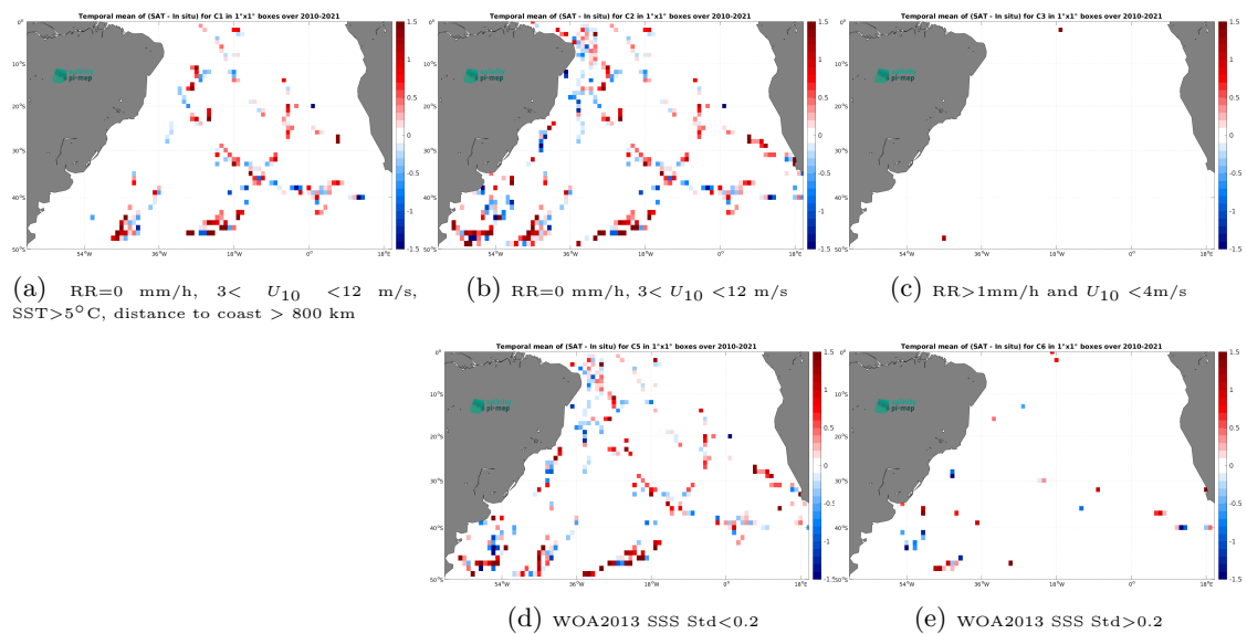
Figure 14: Temporal mean gridded over spatial boxes of size 1^\circ \times 1^\circ of \Delta SSS (SMOS SSS L2 v700 (ESA) - TSG (GOSUD-Sailing-ship)) for 5 different subdatasets corresponding to:RR=0 mm/h, 3 < U_{10} < 12 m/s, SST >5^\circ\text{C} , distance to coast > 800 km (a), RR=0 mm/h, 3 < U_{10} < 12 m/s (b), RR >1 mm/h and U_{10} < 4 m/s (c), WOA2013 SSS Std <0.2 (d), WOA2013 SSS Std >0.2 (e).
