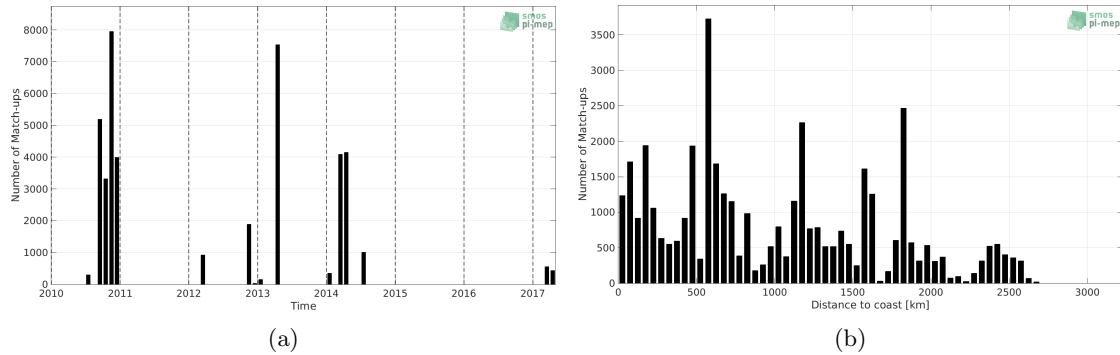
Figure 1: Number of match-ups between TSG (GOSUD-Sailing-ship) and SMOS SSS L2 v700 (ESA) SSS as a function of time (a) and as function of the distance to coast (b) over the South Atlantic Ocean Pi-MEP region and for the full satellite product period.
