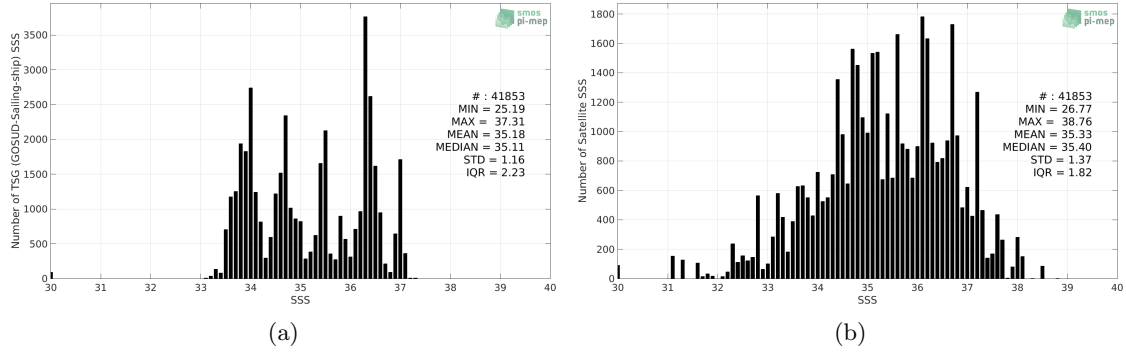
Figure 2: Histograms of SSS from TSG (GOSUD-Sailing-ship) (a) and SMOS SSS L2 v700 (ESA) (b) considering all match-up pairs per bins of 0.1 over the South Atlantic Ocean Pi-MEP region and for the full satellite product period.
