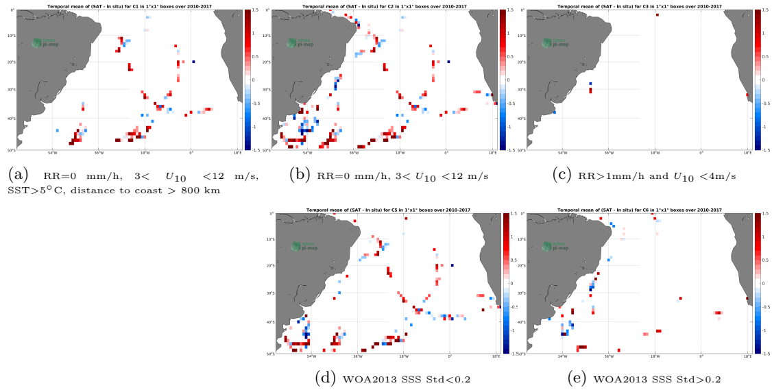
Figure 12: Temporal mean gridded over spatial boxes of size 1^\circ \times 1^\circ of \Delta SSS (SMOS SSS L2 v700 (ESA) - TSG (GOSUD-Sailing-ship)) for 5 different subdatasets corresponding to:RR=0 mm/h, 3 < U_{10} < 12 m/s, SST >5^\circ\text{C} , distance to coast > 800 km (a), RR=0 mm/h, 3 < U_{10} < 12 m/s (b), RR >1 mm/h and U_{10} < 4 m/s (c), WOA2013 SSS Std <0.2 (d), WOA2013 SSS Std >0.2 (e).
