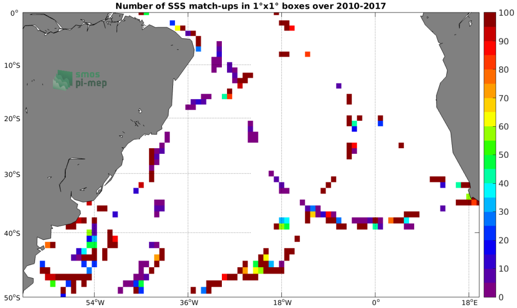
Figure 4: Number of SSS match-ups between TSG (GOSUD-Sailing-ship) SSS and the SMOS SSS L2 v700 (ESA) SSS product for the South Atlantic Ocean Pi-MEP region over 1^\circ \times 1^\circ boxes and for the full satellite product period.
