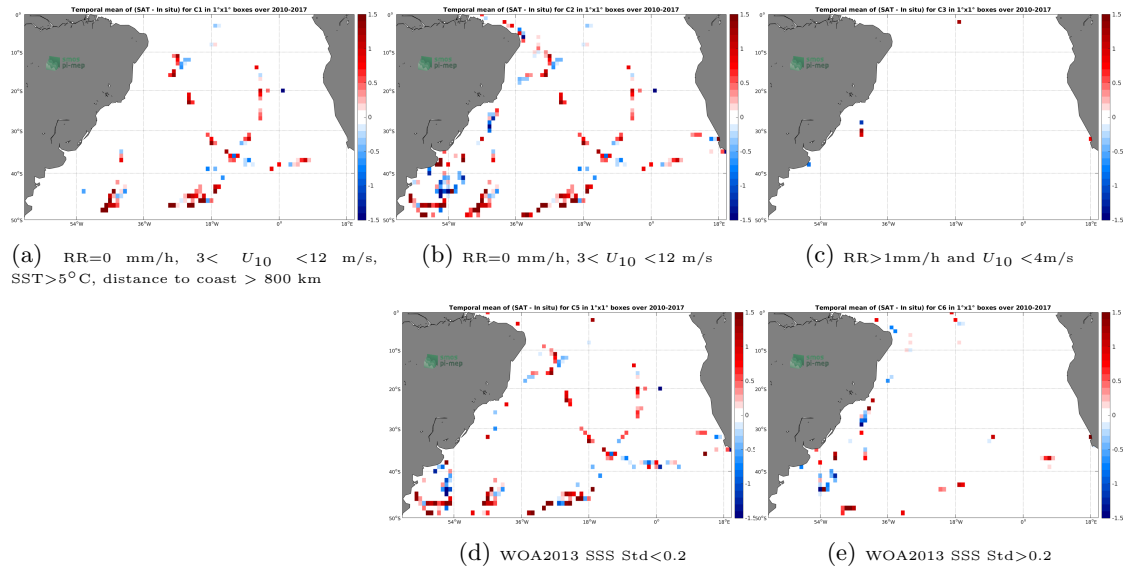
Figure 12: Temporal mean gridded over spatial boxes of size 1^\circ \times 1^\circ of \Delta SSS (SMOS SSS L2 v700 (ESA) - TSG (GOSUD-Sailing-ship)) for 5 different subdatasets corresponding to: RR=0 mm/h, 3 < U_{10} < 12 m/s, SST > 5^\circ C , distance to coast > 800 km (a), RR=0 mm/h, 3 < U_{10} < 12 m/s (b), RR > 1 mm/h and U_{10} < 4 m/s (c), WOA2013 SSS Std < 0.2 (d), WOA2013 SSS Std > 0.2 (e).
