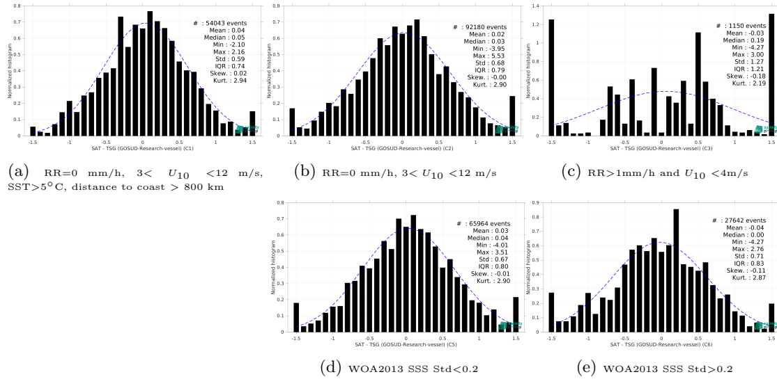
Figure 15: Normalized histogram of \Delta SSS (SMOS SSS L2 v700 (ESA) - TSG (GOSUD-Research-vessel)) for 5 different subdatasets corresponding to: RR=0 mm/h, 3 < U_{10} < 12 m/s, SST > 5°C, distance to coast > 800 km (a), RR=0 mm/h, 3 < U_{10} < 12 m/s (b), RR > 1mm/h and U_{10} < 4 m/s (c), WOA2013 SSS Std < 0.2 (d), WOA2013 SSS Std > 0.2 (e).
