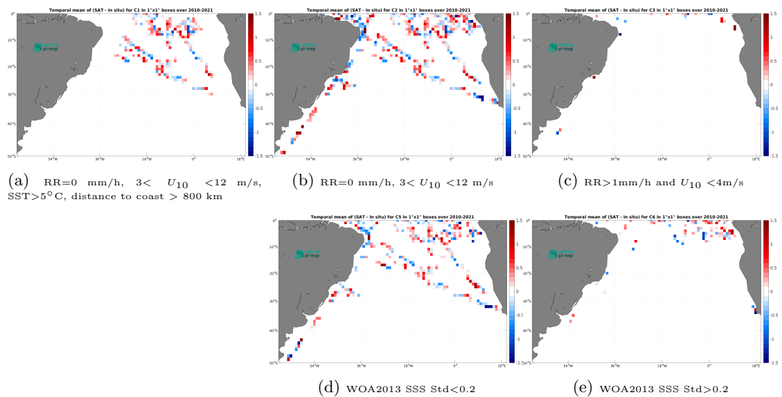
Figure 14: Temporal mean gridded over spatial boxes of size 1^\circ \times 1^\circ of \Delta SSS (SMOS SSS L2 v700 (ESA) - TSG (GOSUD-Research-vessel)) for 5 different subdatasets corresponding to:RR=0 mm/h, 3 < U_{10} < 12 m/s, SST>5°C, distance to coast > 800 km (a), RR=0 mm/h, 3 < U_{10} < 12 m/s (b), RR>1mm/h and U_{10} < 4 m/s (c), WOA2013 SSS Std<0.2 (d), WOA2013 SSS Std>0.2 (e).
