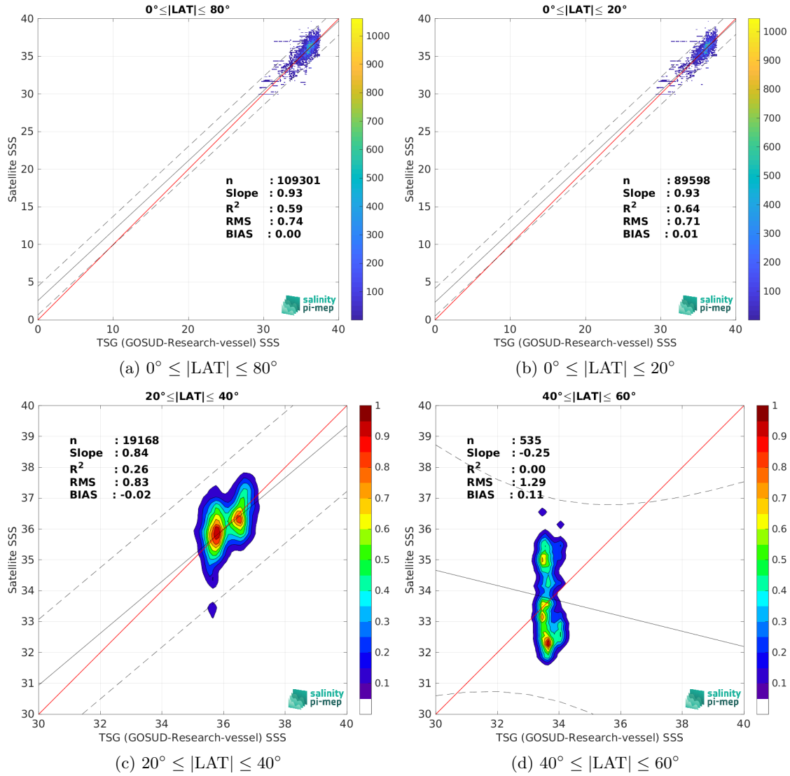
Figure 10: Contour maps of the concentration of SMOS SSS L2 v700 (ESA) SSS (y-axis) versus TSG (GOSUD-Research-vessel) SSS (x-axis) at match-up pairs for different latitude bands. For each plot, the red line shows x=y . The black thin and dashed lines indicate a linear fit through the data cloud and the \pm 95\% confidence levels, respectively. The number match-up pairs n , the slope and R^2 coefficient of the linear fit, the root mean square (RMS) and the mean bias between satellite and in situ data are indicated for each latitude band in each plots.
