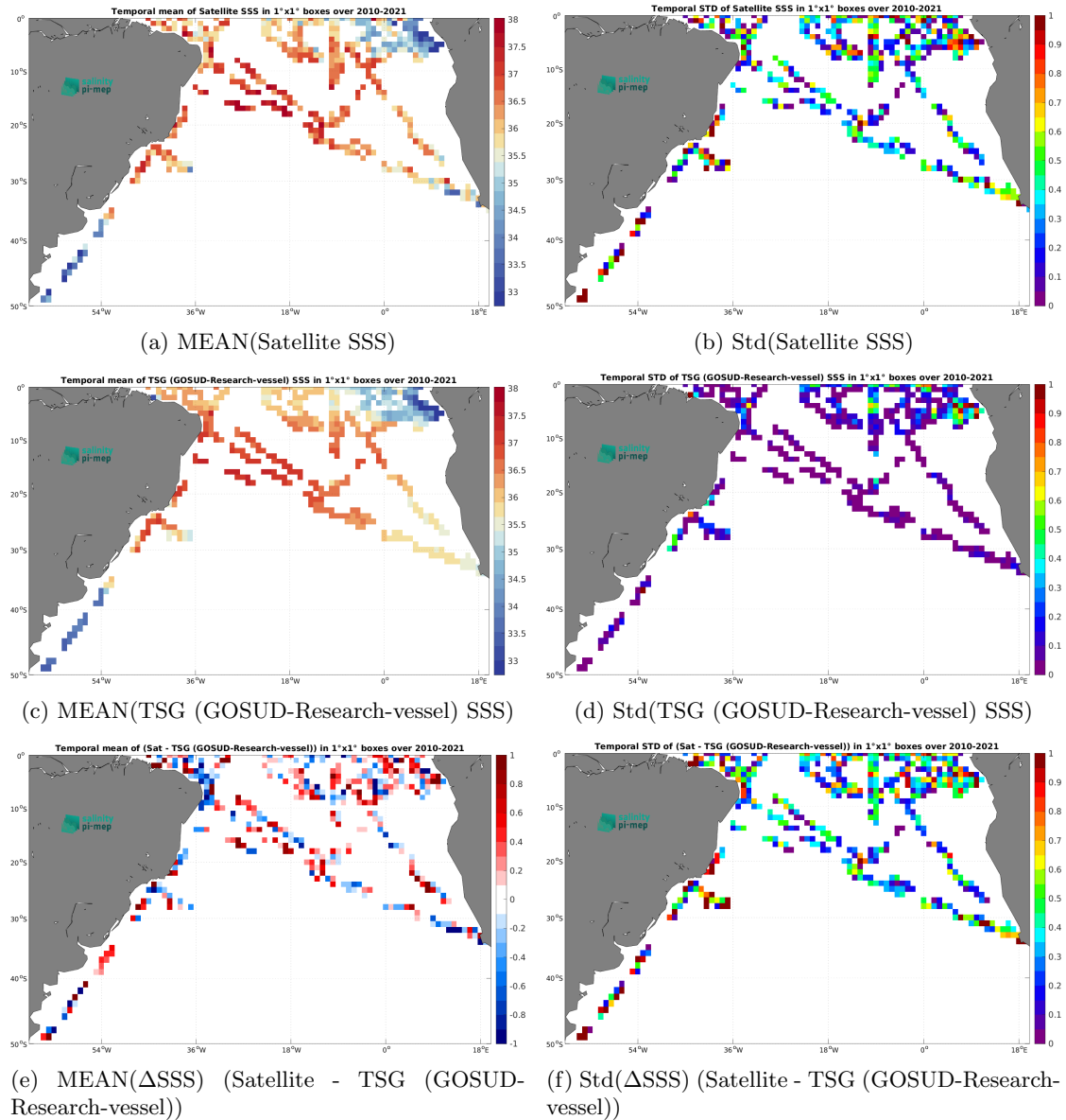
Figure 7: Temporal mean (left) and Std (right) of SSS from SMOS SSS L2 v700 (ESA) (top), TSG (GOSUD-Research-vessel) (middle), and of \Delta SSS (Satellite - TSG (GOSUD-Research-vessel)). Only match-up pairs are used to generate these maps.
