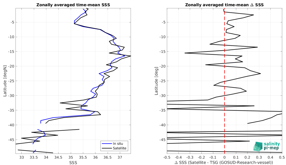
Figure 9: Left panel: Zonal mean SSS from SMOS SSS L2 v700 (ESA) satellite product (black) and from TSG (GOSUD-Research-vessel) (blue). Right panel: Zonal mean of \Delta SSS (Satellite - TSG (GOSUD-Research-vessel)) for all the collected Pi-MEP match-up pairs estimated over the full satellite product period.
