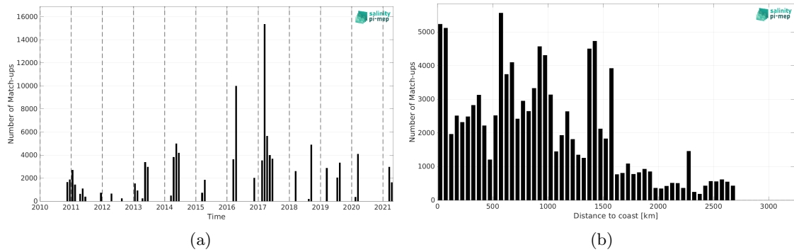
Figure 1: Number of match-ups between TSG (GOSUD-Research-vessel) and SMOS SSS L2 v700 (ESA) SSS as a function of time (a) and as function of the distance to coast (b) over the South Atlantic Ocean Pi-MEP region and for the full satellite product period.
