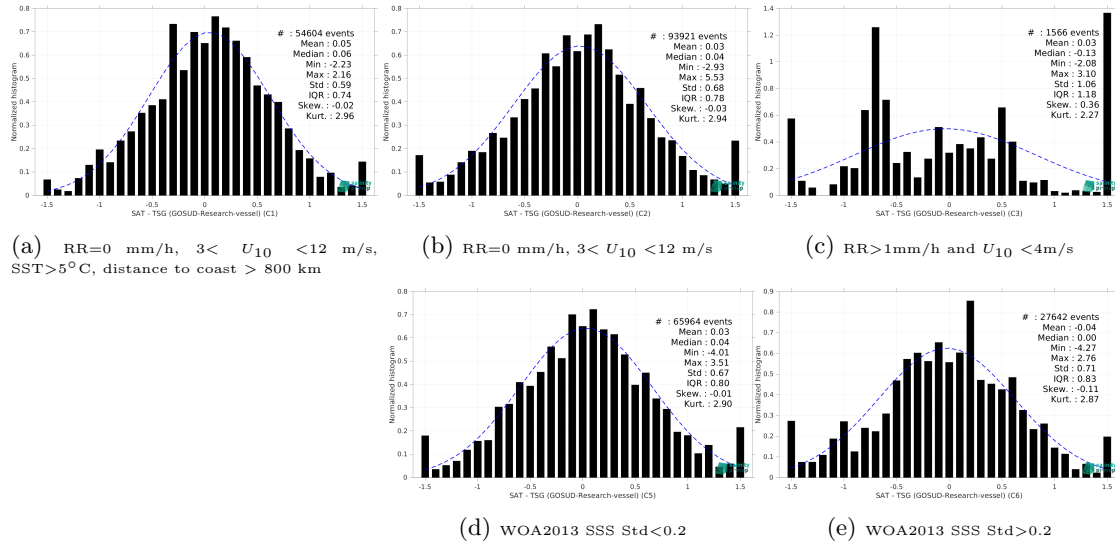
Figure 13: Normalized histogram of \Delta SSS (SMOS SSS L2 v700 (ESA) - TSG (GOSUD-Research-vessel)) for 5 different subdatasets corresponding to: RR=0 mm/h, 3 < U_{10} < 12 m/s, SST > 5°C, distance to coast > 800 km (a), RR=0 mm/h, 3 < U_{10} < 12 m/s (b), RR > 1mm/h and U_{10} < 4 m/s (c), WOA2013 SSS Std < 0.2 (d), WOA2013 SSS Std > 0.2 (e).
