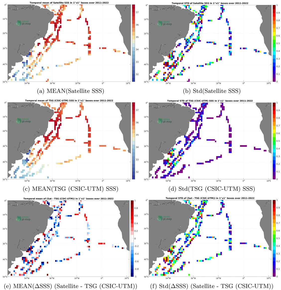
Figure 6: Temporal mean (left) and Std (right) of SSS from SMOS SSS L2 v700 (ESA) (top), TSG (CSIC-UTM) (middle), and of \Delta SSS (Satellite - TSG (CSIC-UTM)). Only match-up pairs are used to generate these maps.
