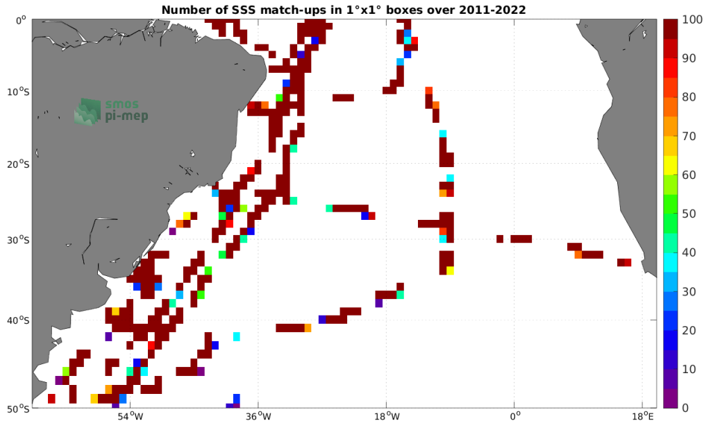
Figure 4: Number of SSS match-ups between TSG (CSIC-UTM) SSS and the SMOS SSS L2 v700 (ESA) SSS product for the South Atlantic Ocean Pi-MEP region over 1^\circ \times 1^\circ boxes and for the full satellite product period.
