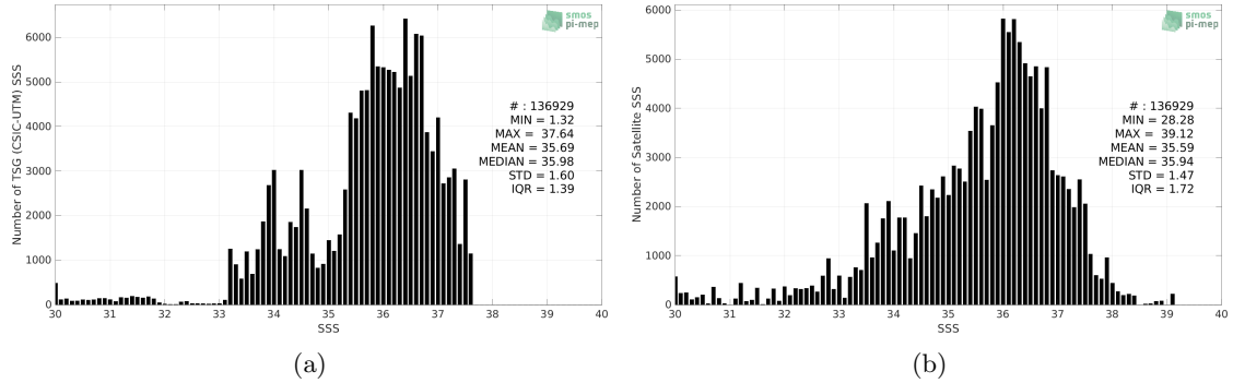
Figure 2: Histograms of SSS from TSG (CSIC-UTM) (a) and SMOS SSS L2 v700 (ESA) (b) considering all match-up pairs per bins of 0.1 over the South Atlantic Ocean Pi-MEP region and for the full satellite product period.
