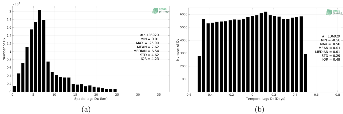
Figure 5: Histograms of the spatial (a) and temporal (b) lags between the location/time of the TSG (CSIC-UTM) measurement and the date of the corresponding SMOS SSS L2 v700 (ESA) SSS pixel.
