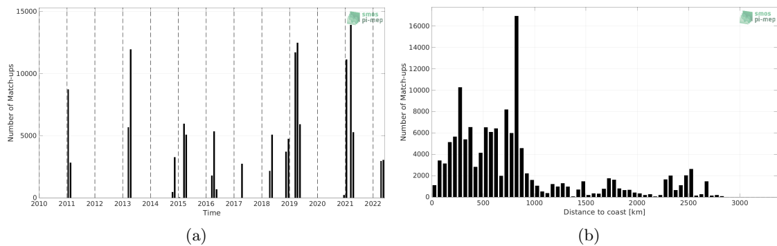
Figure 1: Number of match-ups between TSG (CSIC-UTM) and SMOS SSS L2 v700 (ESA) SSS as a function of time (a) and as function of the distance to coast (b) over the South Atlantic Ocean Pi-MEP region and for the full satellite product period.
