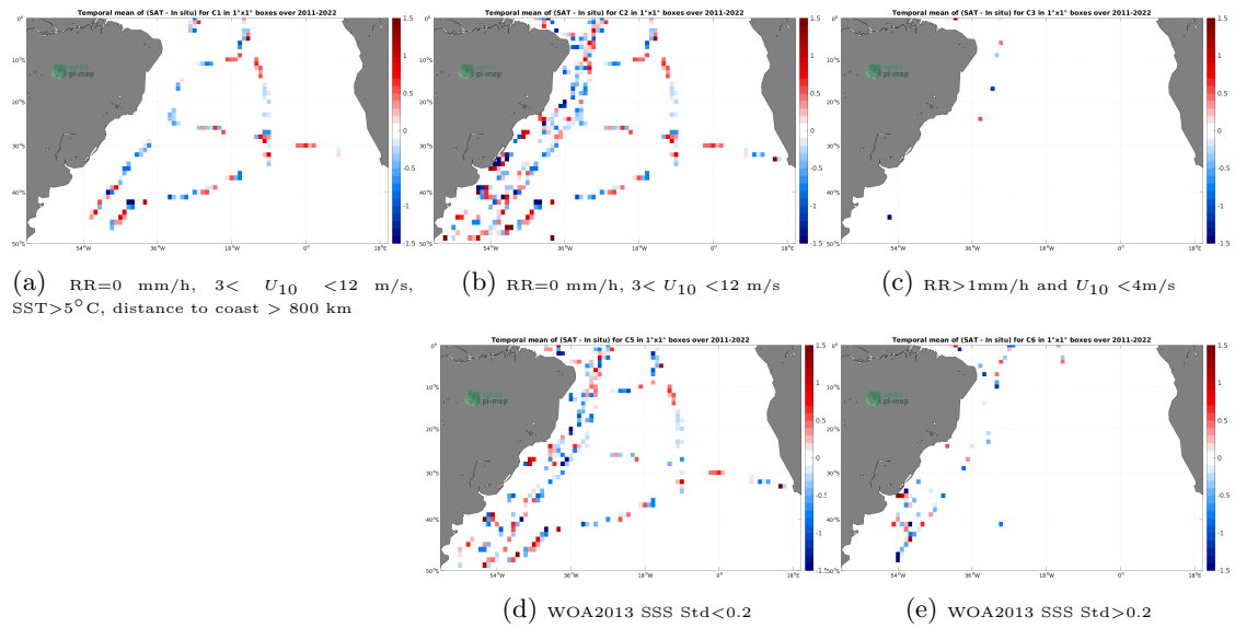
Figure 12: Temporal mean gridded over spatial boxes of size 1^\circ \times 1^\circ of \Delta SSS (SMOS SSS L2 v700 (ESA) - TSG (CSIC-UTM)) for 5 different subdatasets corresponding to:RR=0 mm/h, 3 < U_{10} < 12 m/s, SST >5^\circ\text{C} , distance to coast > 800 km (a), RR=0 mm/h, 3 < U_{10} < 12 m/s (b), RR >1 mm/h and U_{10} < 4 m/s (c), WOA2013 SSS Std <0.2 (d), WOA2013 SSS Std >0.2 (e).
