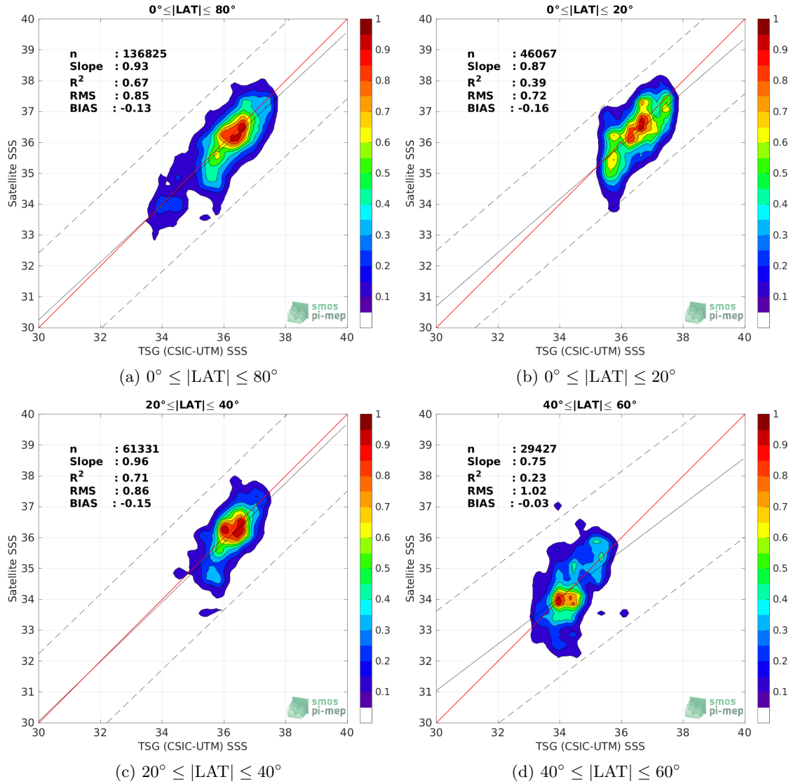
Figure 9: Contour maps of the concentration of SMOS SSS L2 v700 (ESA) SSS (y-axis) versus TSG (CSIC-UTM) SSS (x-axis) at match-up pairs for different latitude bands. For each plot, the red line shows x=y . The black thin and dashed lines indicate a linear fit through the data cloud and the \pm 95\% confidence levels, respectively. The number match-up pairs n , the slope and R^2 coefficient of the linear fit, the root mean square (RMS) and the mean bias between satellite and in situ data are indicated for each latitude band in each plots.
