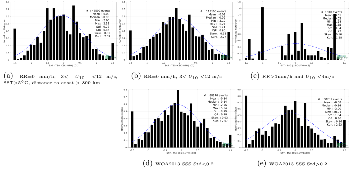
Figure 13: Normalized histogram of \Delta SSS (SMOS SSS L2 v700 (ESA) - TSG (CSIC-UTM)) for 5 different subdatasets corresponding to: RR=0 mm/h, 3 < U_{10} < 12 m/s, SST>5°C, distance to coast > 800 km (a), RR=0 mm/h, 3 < U_{10} < 12 m/s (b), RR>1mm/h and U_{10} < 4 m/s (c), WOA2013 SSS Std<0.2 (d), WOA2013 SSS Std>0.2 (e).
