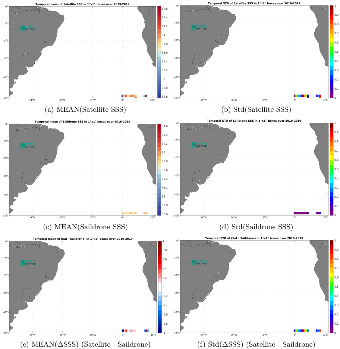
Figure 7: Temporal mean (left) and Std (right) of SSS from SMOS SSS L2 v700 (ESA) (top), Saildrone (middle), and of \Delta SSS (Satellite - Saildrone). Only match-up pairs are used to generate these maps.
