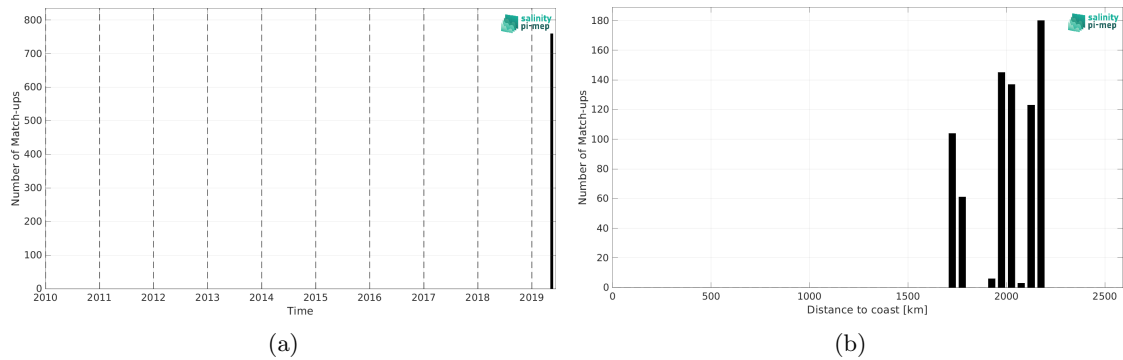
Figure 2: Number of match-ups between Saildrone and SMOS SSS L2 v700 (ESA) SSS as a function of time (a) and as function of the distance to coast (b) over the South Atlantic Ocean Pi-MEP region and for the full satellite product period.
