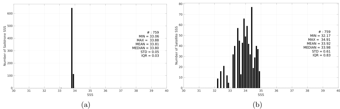
Figure 3: Histograms of SSS from Saildrone (a) and SMOS SSS L2 v700 (ESA) (b) considering all match-up pairs per bins of 0.1 over the South Atlantic Ocean Pi-MEP region and for the full satellite product period.
