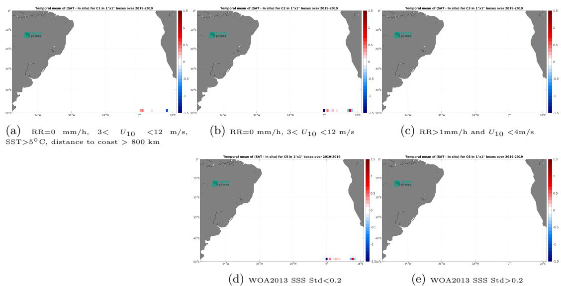
Figure 14: Temporal mean gridded over spatial boxes of size 1^\circ \times 1^\circ of \Delta SSS (SMOS SSS L2 v700 (ESA) - Saldrone) for 5 different subdatasets corresponding to:RR=0 mm/h, 3 < U_{10} < 12 m/s, SST>5°C, distance to coast > 800 km (a), RR=0 mm/h, 3 < U_{10} < 12 m/s (b), RR>1mm/h and U_{10} < 4 m/s (c), WOA2013 SSS Std<0.2 (d), WOA2013 SSS Std>0.2 (e).
