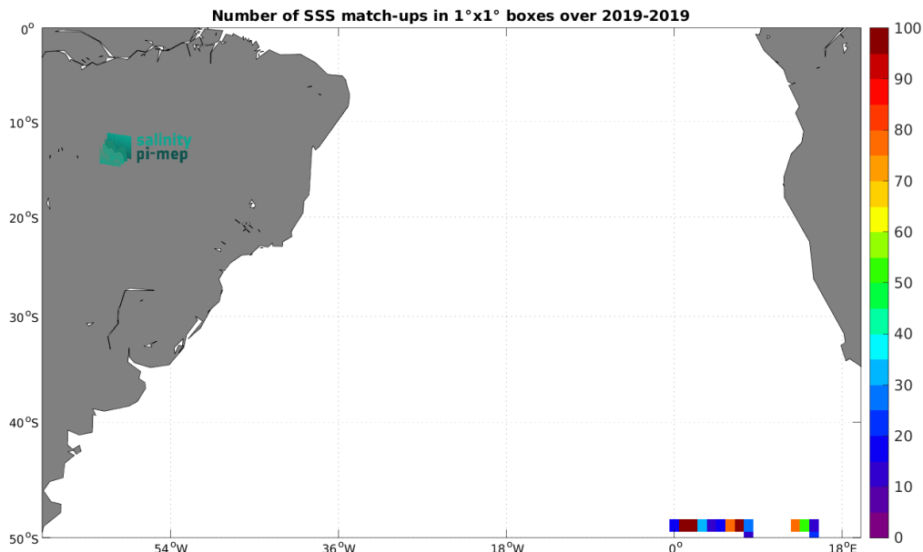
Figure 5: Number of SSS match-ups between Saildrone SSS and the SMOS SSS L2 v700 (ESA) SSS product for the South Atlantic Ocean Pi-MEP region over 1^\circ \times 1^\circ boxes and for the full satellite product period.
