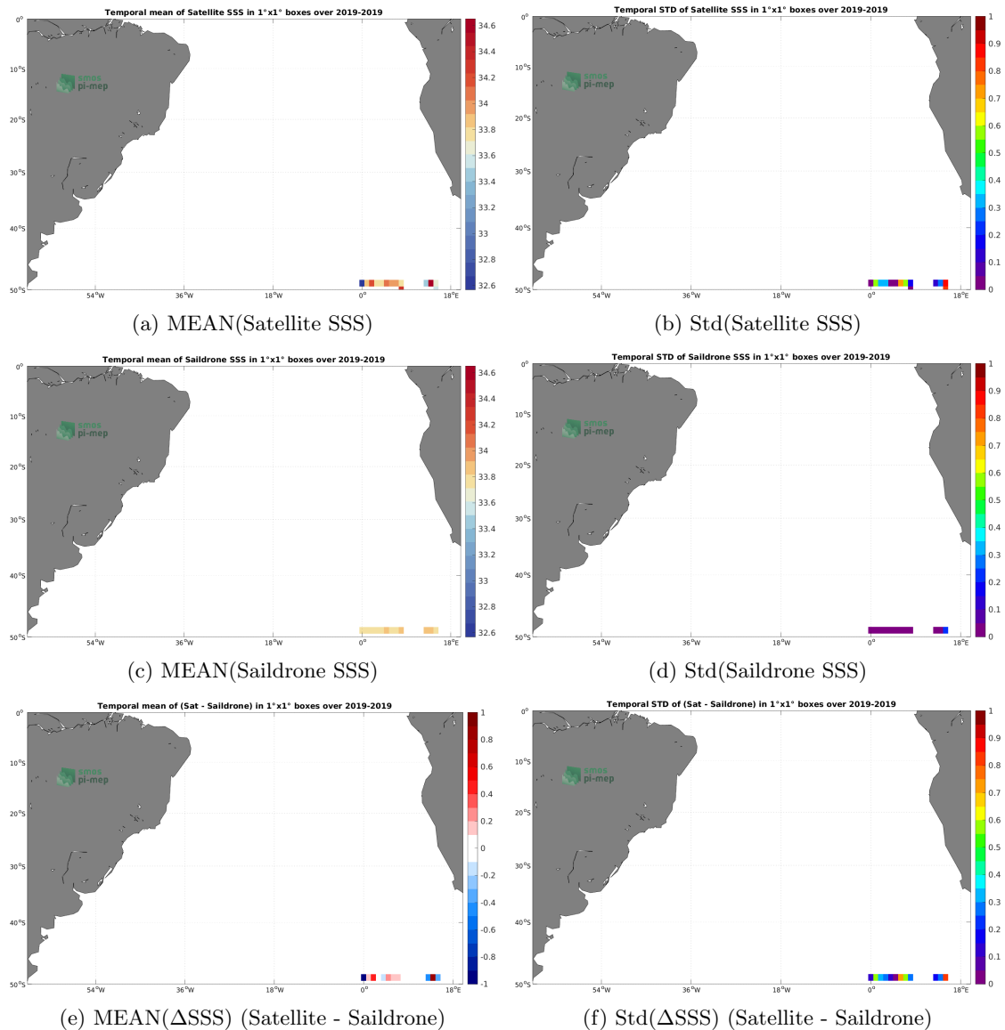
Figure 6: Temporal mean (left) and Std (right) of SSS from SMOS SSS L2 v700 (ESA) (top), Saildrone (middle), and of \Delta SSS (Satellite - Saildrone). Only match-up pairs are used to generate these maps.
