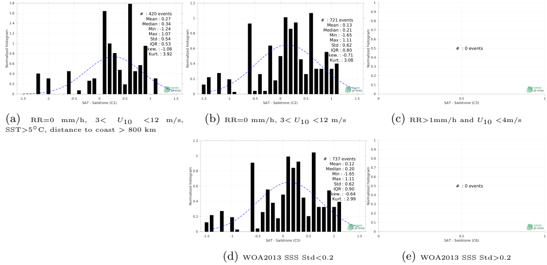
Figure 13: Normalized histogram of \Delta SSS (SMOS SSS L2 v700 (ESA) - Sairdrone) for 5 different subdatasets corresponding to: RR=0 mm/h, 3 < U_{10} < 12 m/s, SST > 5°C, distance to coast > 800 km (a), RR=0 mm/h, 3 < U_{10} < 12 m/s (b), RR > 1mm/h and U_{10} < 4 m/s (c), WOA2013 SSS Std < 0.2 (d), WOA2013 SSS Std > 0.2 (e).
