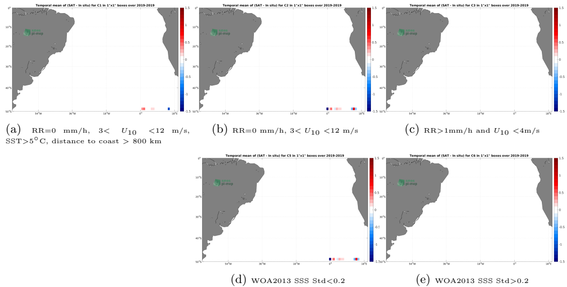
Figure 12: Temporal mean gridded over spatial boxes of size 1^{\circ}\times 1^{\circ} of \Delta\text{SSS} (SMOS SSS L2 v700 (ESA) - Sairdrone) for 5 different subdatasets corresponding to:RR=0 mm/h, 3 < U_{10} < 12 m/s, SST >5^{\circ}\text{C} , distance to coast > 800 km (a), RR=0 mm/h, 3 < U_{10} < 12 m/s (b), RR >1 mm/h and U_{10} < 4 m/s (c), WOA2013 SSS Std <0.2 (d), WOA2013 SSS Std >0.2 (e).
