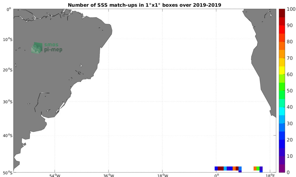
Figure 4: Number of SSS match-ups between Saildrone SSS and the SMOS SSS L2 v700 (ESA) SSS product for the South Atlantic Ocean Pi-MEP region over 1^\circ \times 1^\circ boxes and for the full satellite product period.
