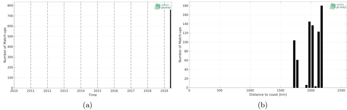
Figure 1: Number of match-ups between Saildrone and SMOS SSS L2 v700 (ESA) SSS as a function of time (a) and as function of the distance to coast (b) over the South Atlantic Ocean Pi-MEP region and for the full satellite product period.
