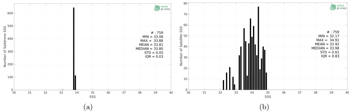
Figure 2: Histograms of SSS from Saildrone (a) and SMOS SSS L2 v700 (ESA) (b) considering all match-up pairs per bins of 0.1 over the South Atlantic Ocean Pi-MEP region and for the full satellite product period.
