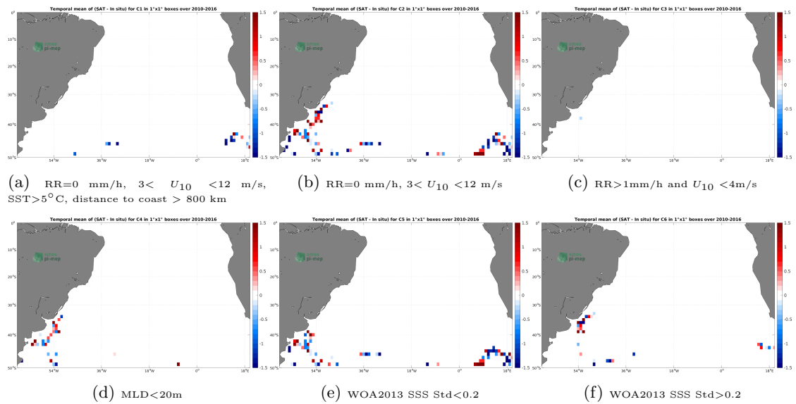
Figure 12: Temporal mean gridded over spatial boxes of size 1^\circ \times 1^\circ of \Delta SSS (SMOS SSS L2 v700 (ESA) - Marine mammals) for 6 different subdatasets corresponding to:RR=0 mm/h, 3 < U_{10} < 12 m/s, SST > 5^\circ\text{C} , distance to coast > 800 km (a), RR=0 mm/h, 3 < U_{10} < 12 m/s (b), RR > 1 mm/h and U_{10} < 4 m/s (c),MLD < 20 m (d),WOA2013 SSS Std < 0.2 (e),WOA2013 SSS Std > 0.2 (f).
