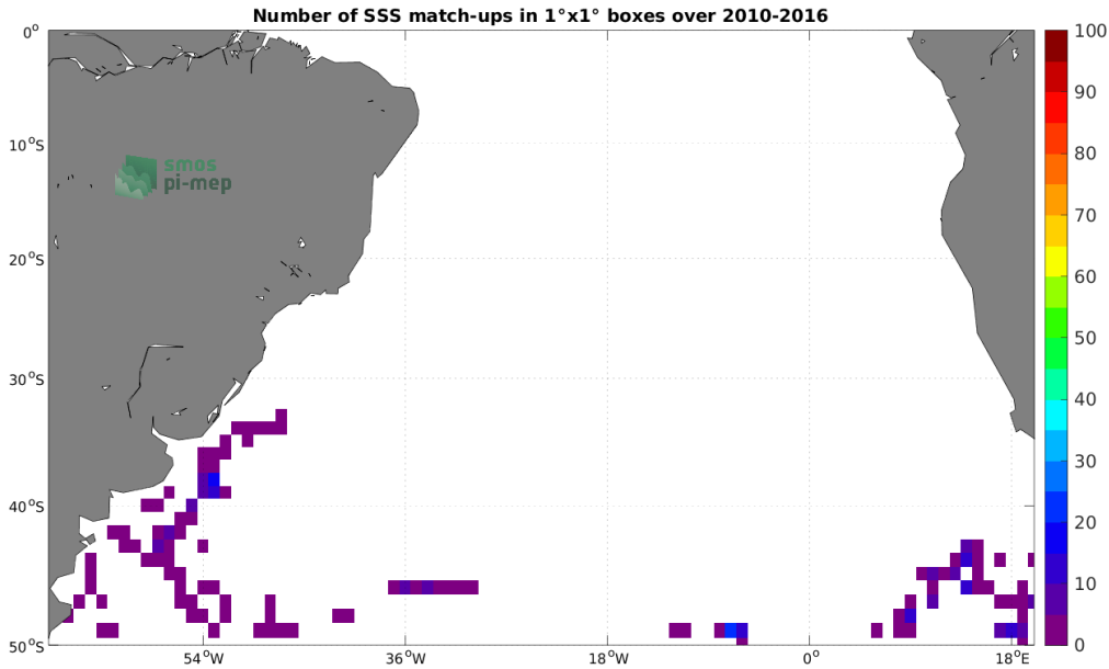
Figure 4: Number of SSS match-ups between Marine mammals SSS and the SMOS SSS L2 v700 (ESA) SSS product for the South Atlantic Ocean Pi-MEP region over 1^\circ \times 1^\circ boxes and for the full satellite product period.
