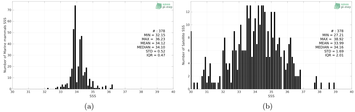
Figure 2: Histograms of SSS from Marine mammals (a) and SMOS SSS L2 v700 (ESA) (b) considering all match-up pairs per bins of 0.1 over the South Atlantic Ocean Pi-MEP region and for the full satellite product period.
