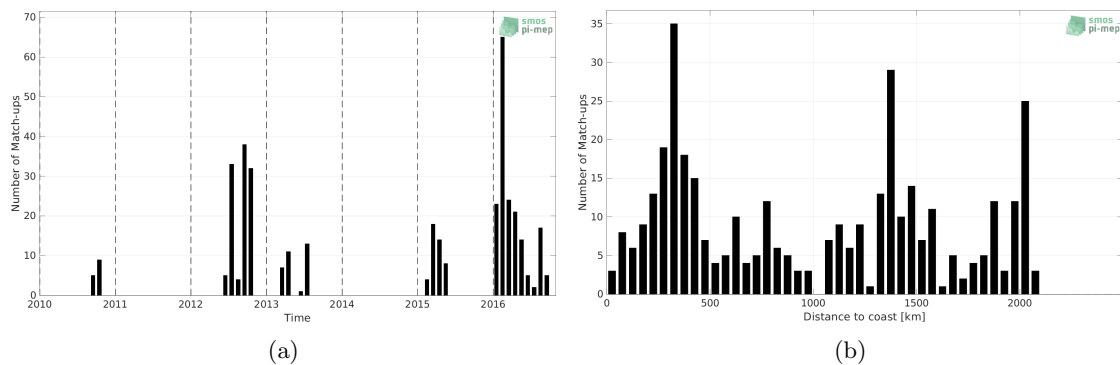
Figure 1: Number of match-ups between Marine mammals and SMOS SSS L2 v700 (ESA) SSS as a function of time (a) and as function of the distance to coast (b) over the South Atlantic Ocean Pi-MEP region and for the full satellite product period.
