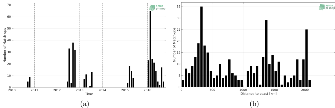
Figure 1: Number of match-ups between Marine mammals and SMOS SSS L2 v700 (ESA) SSS as a function of time (a) and as function of the distance to coast (b) over the South Atlantic Ocean Pi-MEP region and for the full satellite product period.
