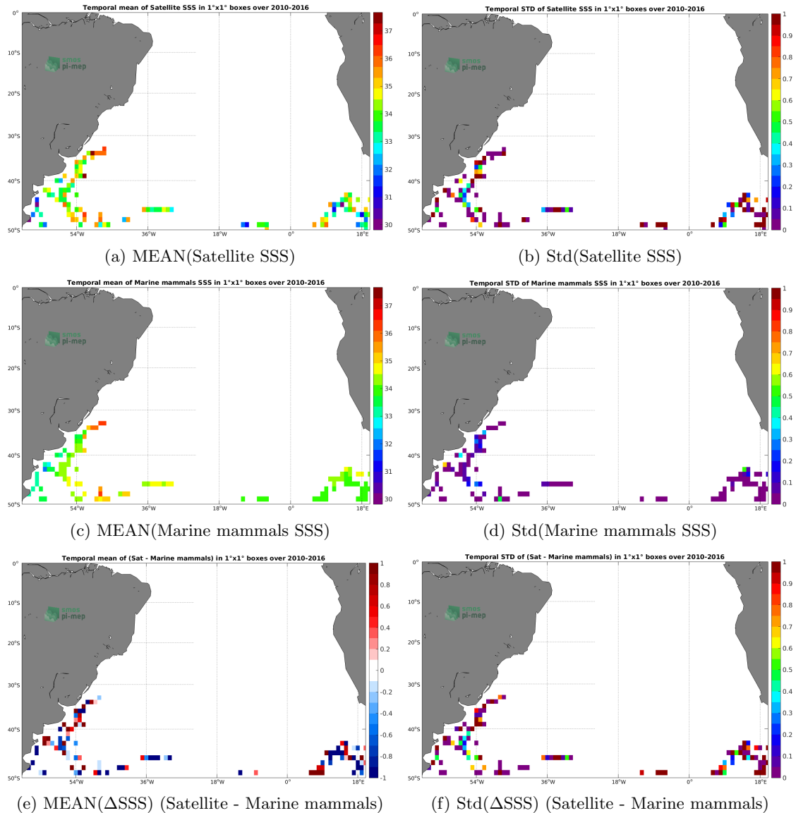
Figure 6: Temporal mean (left) and Std (right) of SSS from SMOS SSS L2 v700 (ESA) (top), Marine mammals (middle), and of \Delta SSS (Satellite - Marine mammals). Only match-up pairs are used to generate these maps.
