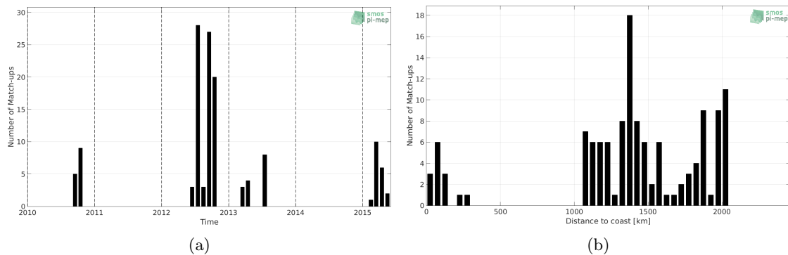
Figure 1: Number of match-ups between Sea mammals and SMOS SSS L2 v700 (ESA) SSS as a function of time (a) and as function of the distance to coast (b) over the South Atlantic Ocean Pi-MEP region and for the full satellite product period.
