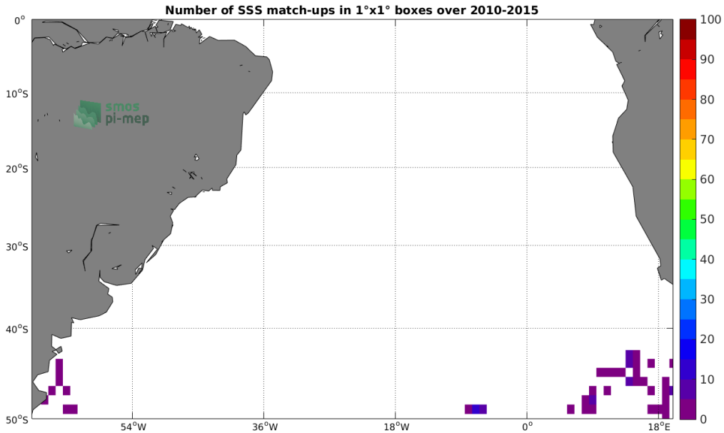
Figure 4: Number of SSS match-ups between Sea mammals SSS and the SMOS SSS L2 v700 (ESA) SSS product for the South Atlantic Ocean Pi-MEP region over 1°x1° boxes and for the full satellite product period.
