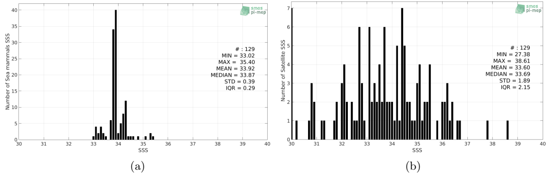
Figure 2: Histograms of SSS from Sea mammals (a) and SMOS SSS L2 v700 (ESA) (b) considering all match-up pairs per bins of 0.1 over the South Atlantic Ocean Pi-MEP region and for the full satellite product period.
