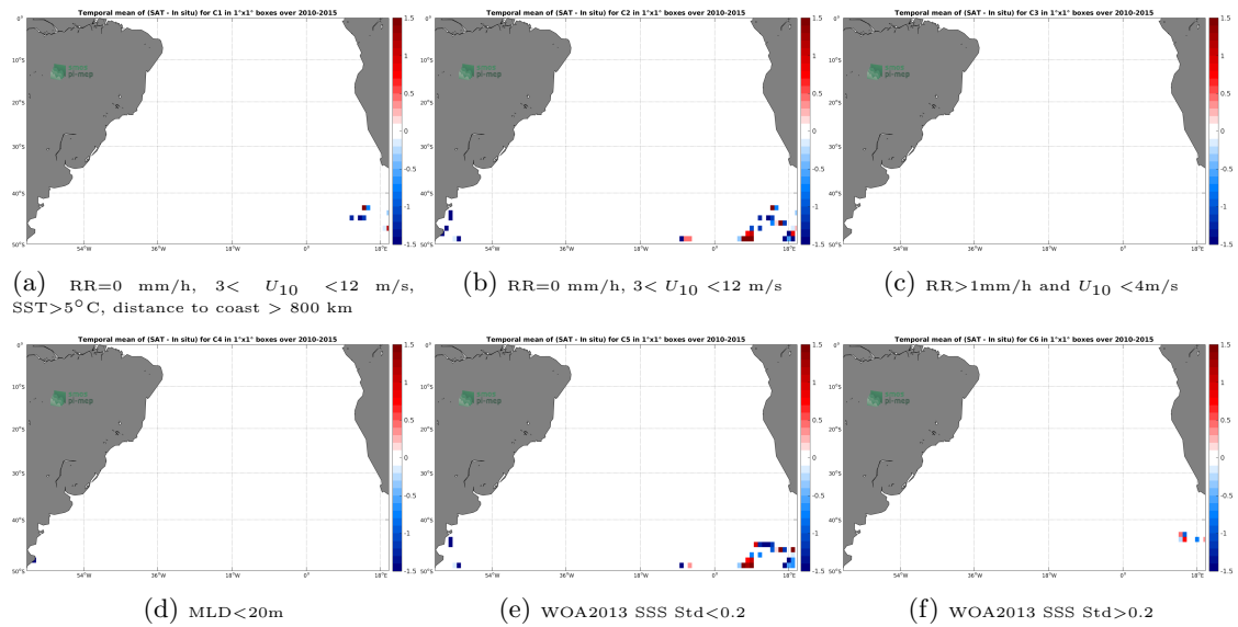
Figure 12: Temporal mean gridded over spatial boxes of size 1^{\circ}\times 1^{\circ} of \Delta\text{SSS} (SMOS SSS L2 v700 (ESA) - Sea mammals) for 6 different subdatasets corresponding to:RR=0 mm/h, 3 < U_{10} < 12 m/s, SST >5^{\circ}\text{C} , distance to coast > 800 km (a), RR=0 mm/h, 3 < U_{10} < 12 m/s (b), RR >1\text{mm/h} and U_{10} < 4\text{m/s} (c),MLD <20\text{m} (d),WOA2013 SSS Std <0.2 (e),WOA2013 SSS Std >0.2 (f).
