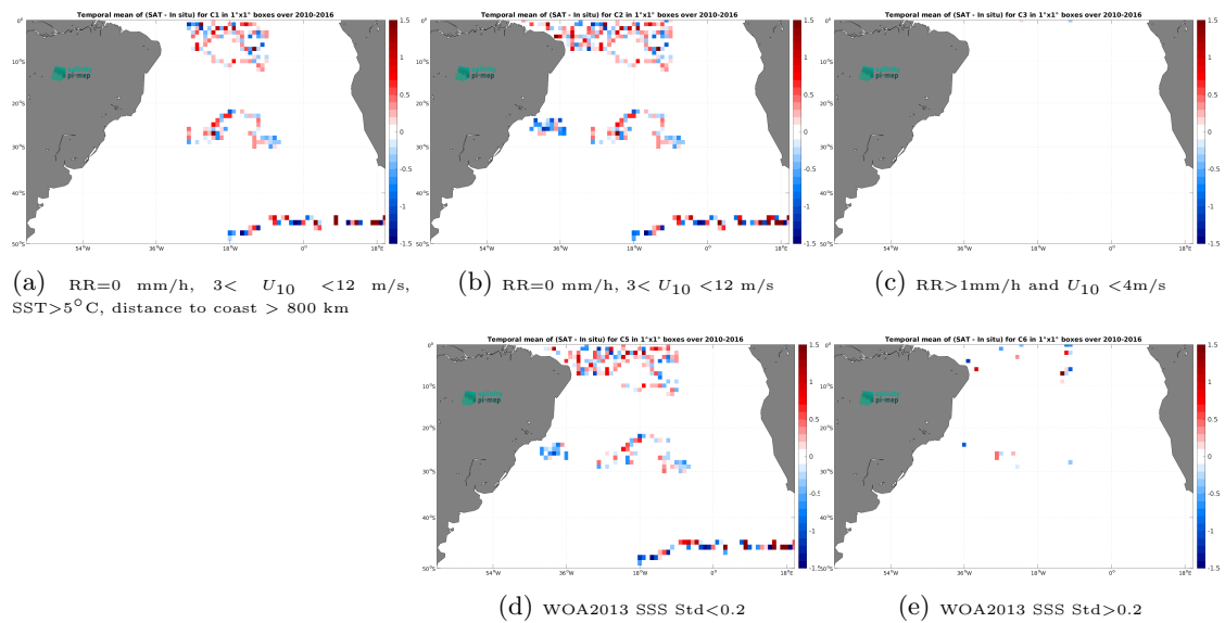
Figure 13: Temporal mean gridded over spatial boxes of size 1^\circ \times 1^\circ of \Delta SSS (SMOS SSS L2 v700 (ESA) - Surface drifters) for 5 different subdatasets corresponding to:RR=0 mm/h, 3 < U_{10} < 12 m/s, SST >5^\circ\text{C} , distance to coast > 800 km (a), RR=0 mm/h, 3 < U_{10} < 12 m/s (b), RR >1 mm/h and U_{10} < 4 m/s (c), WOA2013 SSS Std <0.2 (d), WOA2013 SSS Std >0.2 (e).
