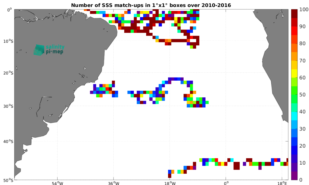
Figure 4: Number of SSS match-ups between Surface drifters SSS and the SMOS SSS L2 v700 (ESA) SSS product for the South Atlantic Ocean Pi-MEP region over 1^{\circ} \times 1^{\circ} boxes and for the full satellite product period.
