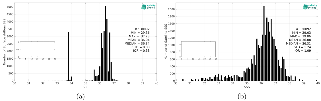
Figure 3: Histograms of SSS from Surface drifters (a) and SMOS SSS L2 v700 (ESA) (b) considering all match-up pairs per bins of 0.1 over the South Atlantic Ocean Pi-MEP region and for the full satellite product period.
