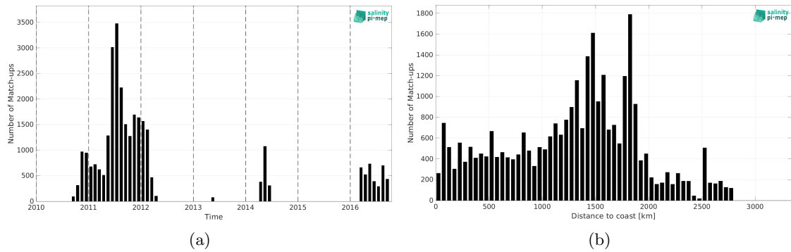
Figure 2: Number of match-ups between Surface drifters and SMOS SSS L2 v700 (ESA) SSS as a function of time (a) and as function of the distance to coast (b) over the South Atlantic Ocean Pi-MEP region and for the full satellite product period.
