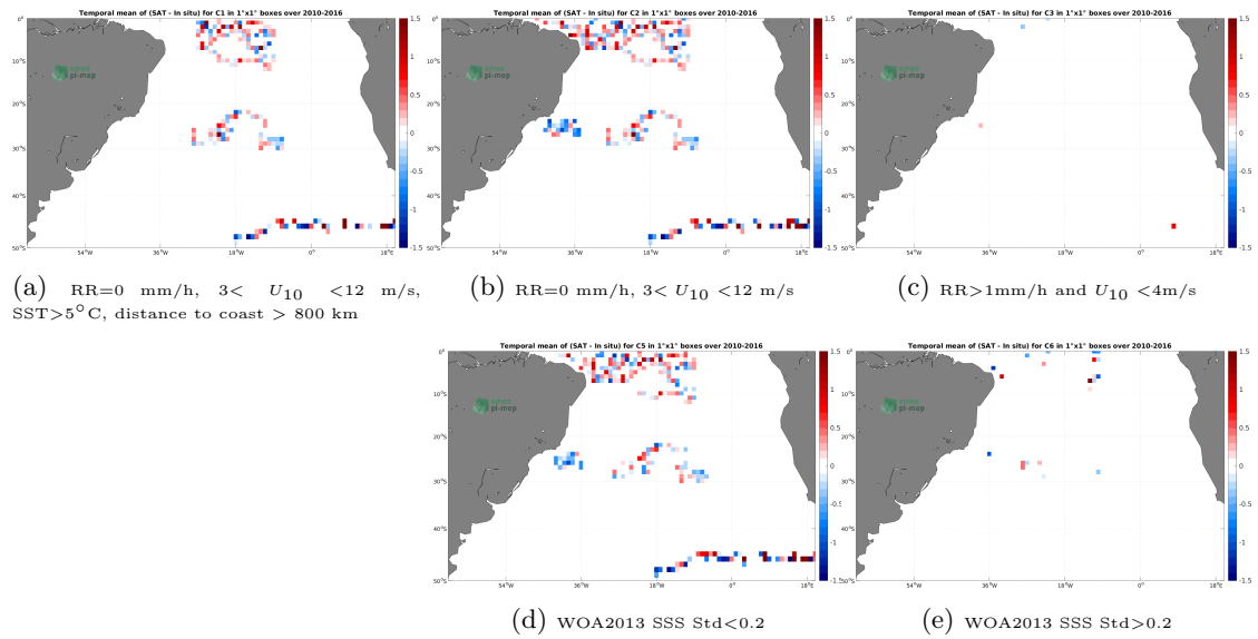
Figure 11: Temporal mean gridded over spatial boxes of size 1^\circ \times 1^\circ of \Delta SSS (SMOS SSS L2 v700 (ESA) - Surface drifters) for 5 different subdatasets corresponding to:RR=0 mm/h, 3 < U_{10} < 12 m/s, SST >5^\circ\text{C} , distance to coast > 800 km (a), RR=0 mm/h, 3 < U_{10} < 12 m/s (b), RR >1 mm/h and U_{10} < 4 m/s (c), WOA2013 SSS Std <0.2 (d), WOA2013 SSS Std >0.2 (e).
