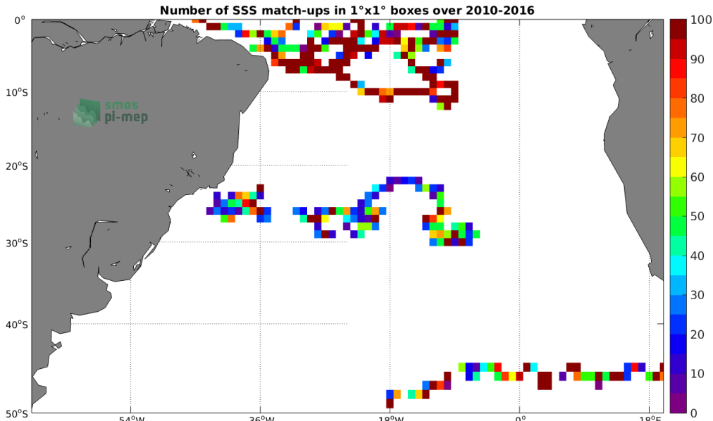
Figure 3: Number of SSS match-ups between Surface drifters SSS and the SMOS SSS L2 v700 (ESA) SSS product for the South Atlantic Ocean Pi-MEP region over 1^\circ \times 1^\circ boxes and for the full satellite product period.
