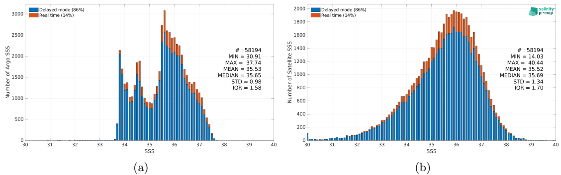
Figure 2: Histograms of SSS from Argo (a) and SMOS SSS L2 v700 (ESA) (b) considering all match-up pairs per bins of 0.1 over the South Atlantic Ocean Pi-MEP region and for the full satellite product period.
