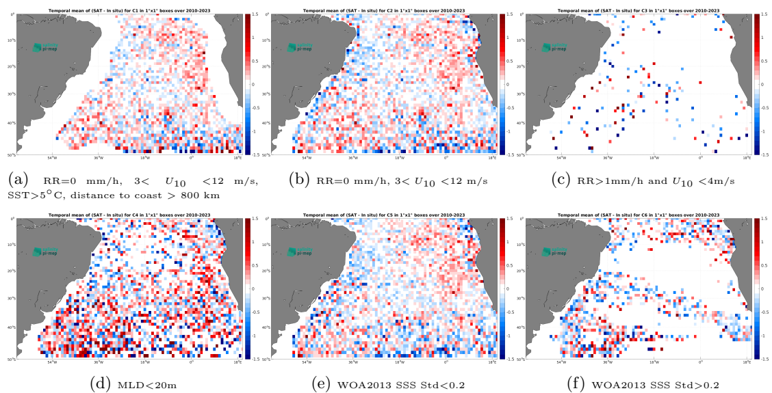
Figure 12: Temporal mean gridded over spatial boxes of size 1^\circ \times 1^\circ of \Delta SSS (SMOS SSS L2 v700 (ESA) - Argo) for 6 different subdatasets corresponding to:RR=0 mm/h, 3 < U_{10} < 12 m/s, SST >5^\circ C, distance to coast > 800 km (a), RR=0 mm/h, 3 < U_{10} < 12 m/s (b), RR >1 mm/h and U_{10} < 4 m/s (c),MLD <20 m (d),WOA2013 SSS Std <0.2 (e),WOA2013 SSS Std >0.2 (f).
