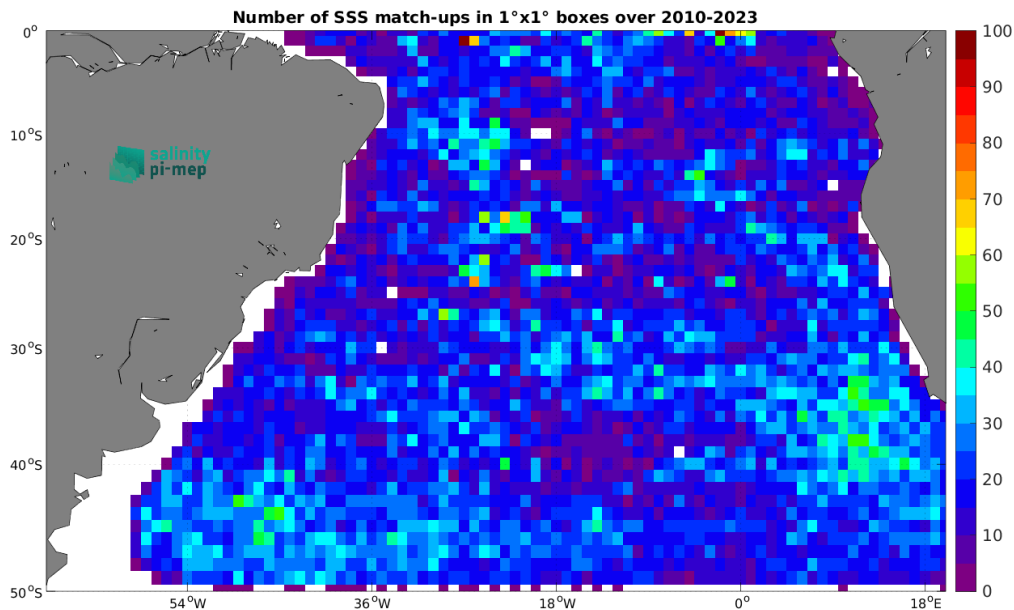
Figure 4: Number of SSS match-ups between Argo SSS and the SMOS SSS L2 v700 (ESA) SSS product for the South Atlantic Ocean Pi-MEP region over 1^\circ \times 1^\circ boxes and for the full satellite product period.
