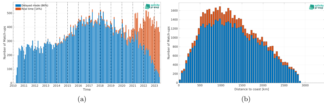
Figure 1: Number of match-ups between Argo and SMOS SSS L2 v700 (ESA) SSS as a function of time (a) and as function of the distance to coast (b) over the South Atlantic Ocean Pi-MEP region and for the full satellite product period.
