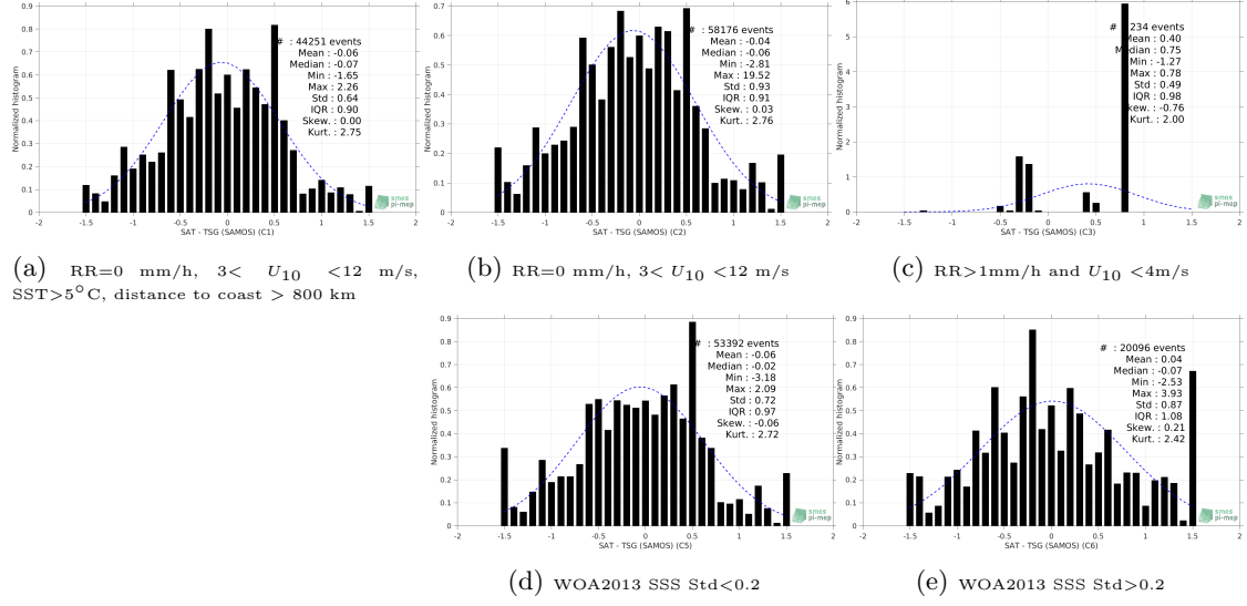
Figure 13: Normalized histogram of \Delta SSS (SMOS SSS L2 v662 (ESA) - TSG (SAMOS)) for 5 different subdatasets corresponding to: RR=0 mm/h, 3 < U_{10} < 12 m/s, SST>5°C, distance to coast > 800 km (a), RR=0 mm/h, 3 < U_{10} < 12 m/s (b), RR>1mm/h and U_{10} < 4 m/s (c), WOA2013 SSS Std<0.2 (d), WOA2013 SSS Std>0.2 (e).
