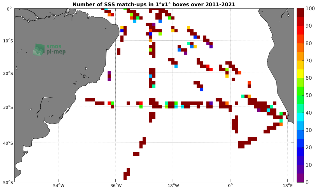
Figure 4: Number of SSS match-ups between TSG (SAMOS) SSS and the SMOS SSS L2 v662 (ESA) SSS product for the South Atlantic Ocean Pi-MEP region over 1^\circ \times 1^\circ boxes and for the full satellite product period.
